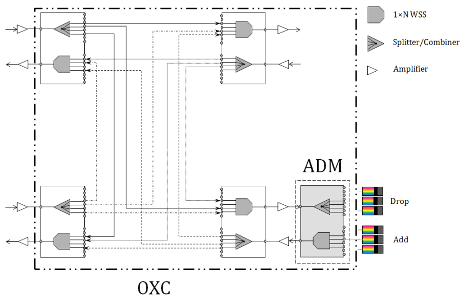
Figure 3.4: WSS-based OXC.
