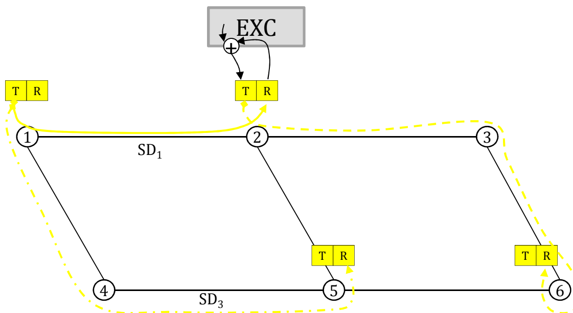
Figure 7.3: Transceiver reutilization.
