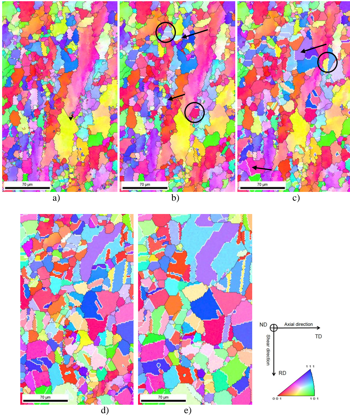
Figure 6-26 Inverse Pole Figure maps showing the gradual evolution of PDRX process of the sample deformed to 1.5 at 1000 °C and 0.01\text{s}^{-1} , white lines represent twin boundary, a) After deformation, b) 20s, c) 20s, d) 15s, e) 15s, all of them are times for each individual heating step and the white lines represent twin boundaries
