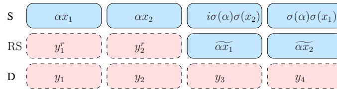
Figure 3.15: Transmission frame of the Incomplete DF protocol in the 1-relay case implemented with a distributed Golden code
