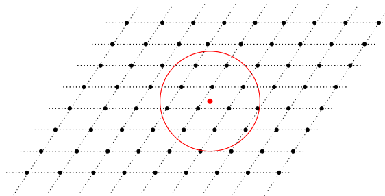
Figure 1.9: Search in an hypersphere centered on the received signal
