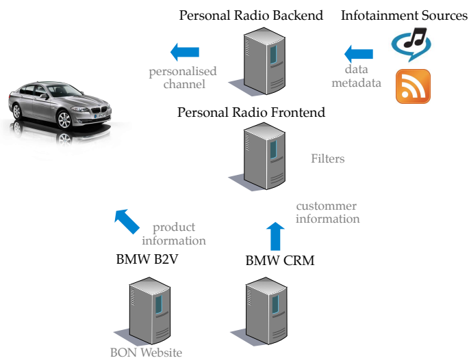
Figure 31: Integration of customer relationship management in the personal radio
