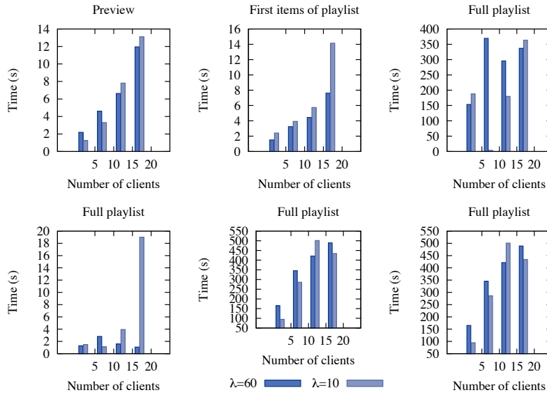
Figure 75: Stress tests of the architecture with different charges of clients and different number of concurrent threads for the server
