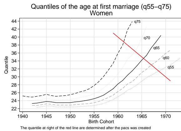
FIGURE 3.22: Quantiles (women)
