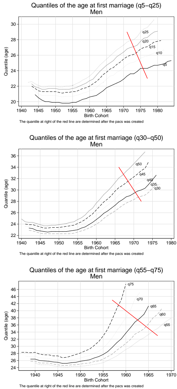
FIGURE 3.20: Quantiles (men)
