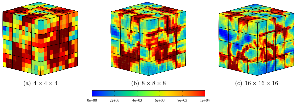
Figure 4.28: Dislocation density (in \text{mm}^{-2} ) after 10% applied strain
