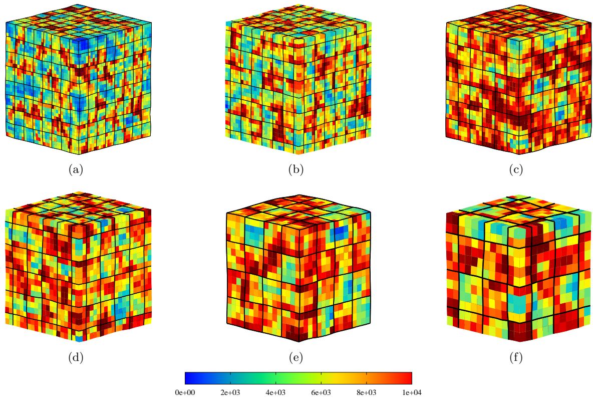
Figure 4.34: Distribution of all dislocation densities (in mm -2 ) after 10% tensile strain
