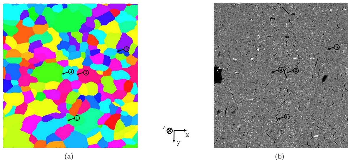
Figure 6.6: (a) free surface of the recorded volume and (b) SEM micrograph After 4.5 % applied strain. Grain boundaries (1), (2), (3) and (4) are those characterised in Figure 6.7. The loading direction is horizontal.
