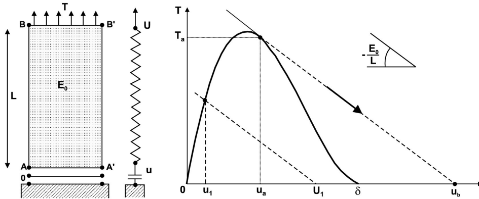
Figure 5.9: Simple uniaxial configuration that illustrates the "solution jumps": (a) the plate and interface elements and (b) the interface nodes response, applied traction ( \mathbf{T} ) versus displacement ( \mathbf{U} ), see (Chaboche et al. 2001)
