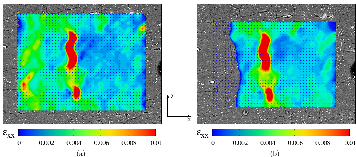
Figure 3.10: Strain distributions (a) with sub-pixel interpolation (b) without sub-pixel interpolation
