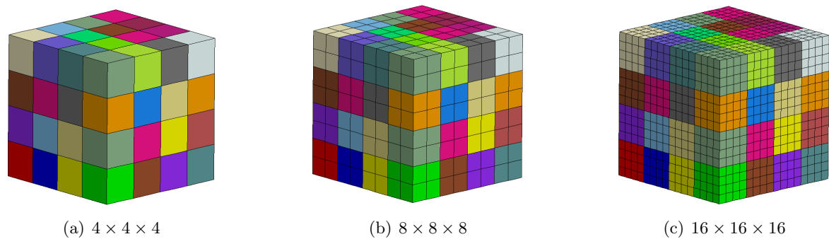
Figure 4.25: Polycrystalline aggregates with a regular mesh of 64 grains with (a) 4 \times 4 \times 4 , (b) 8 \times 8 \times 8 and (c) 16 \times 16 \times 16 elements used to evaluate mesh density on macroscopic behavior
