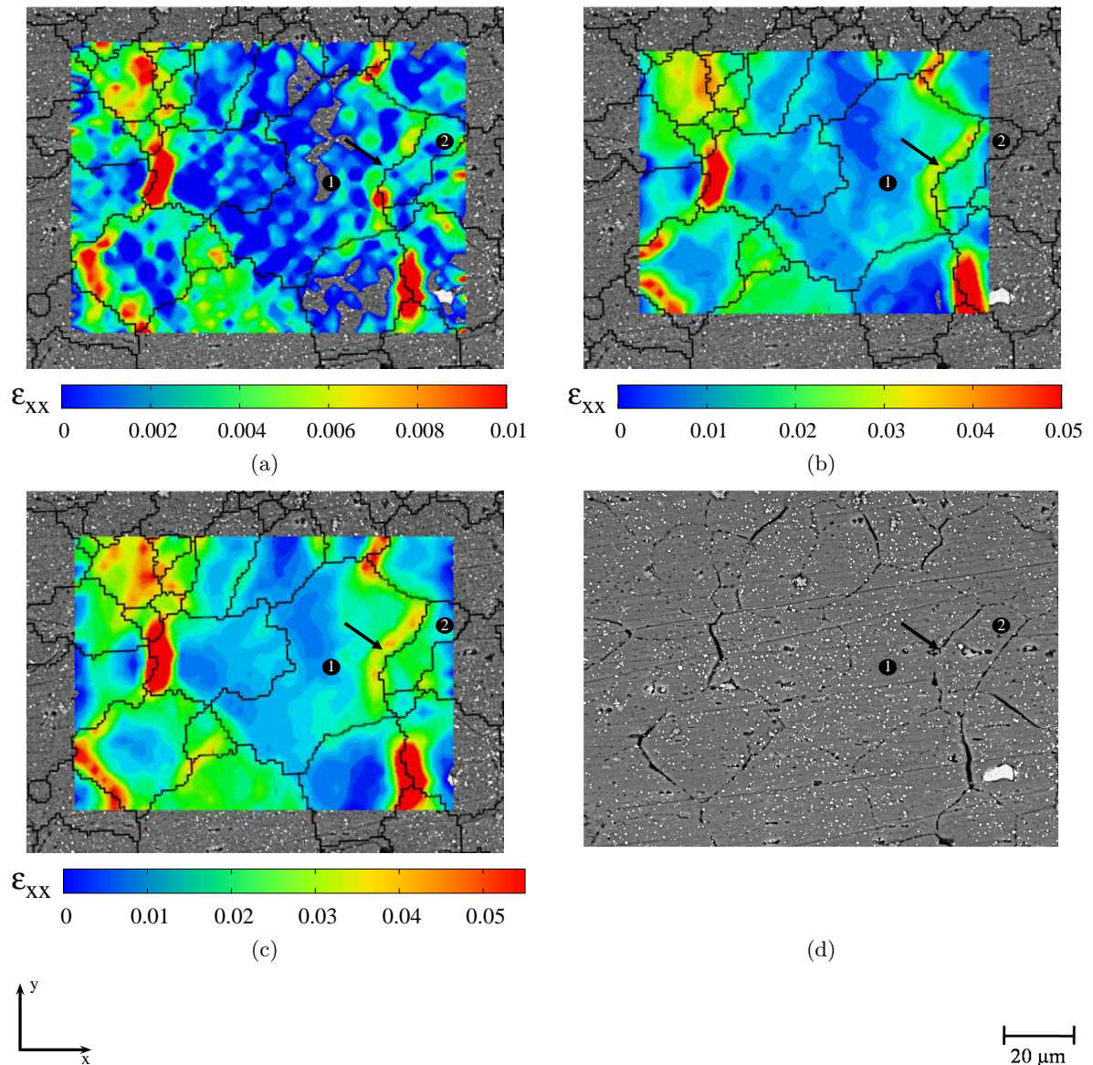
Figure 3.15: Strain distributions for Specimen (I) at small magnification along the x direction for macroscopic applied strains of (a) 0.5%, (b) 1.6% and (c) 2.6%, and (d) SEM image taken after 4.5% applied strain. Black arrow indicates a region with high strain level at a grain boundary that did not crack.
