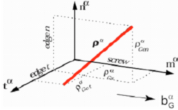
Figure 4.8: Local orthogonal coordinate system for a generic geometrically necessary dislocation line in an arbitrary slip system \alpha (Busso et al. 2000)
