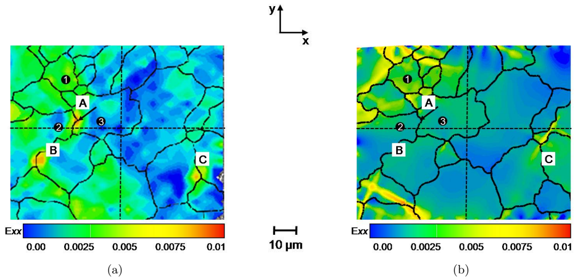
Figure 4.46: (a) Measured and (b) predicted axial strain fields after an average tensile strain of 0.0045. The load is applied along the x axis.
