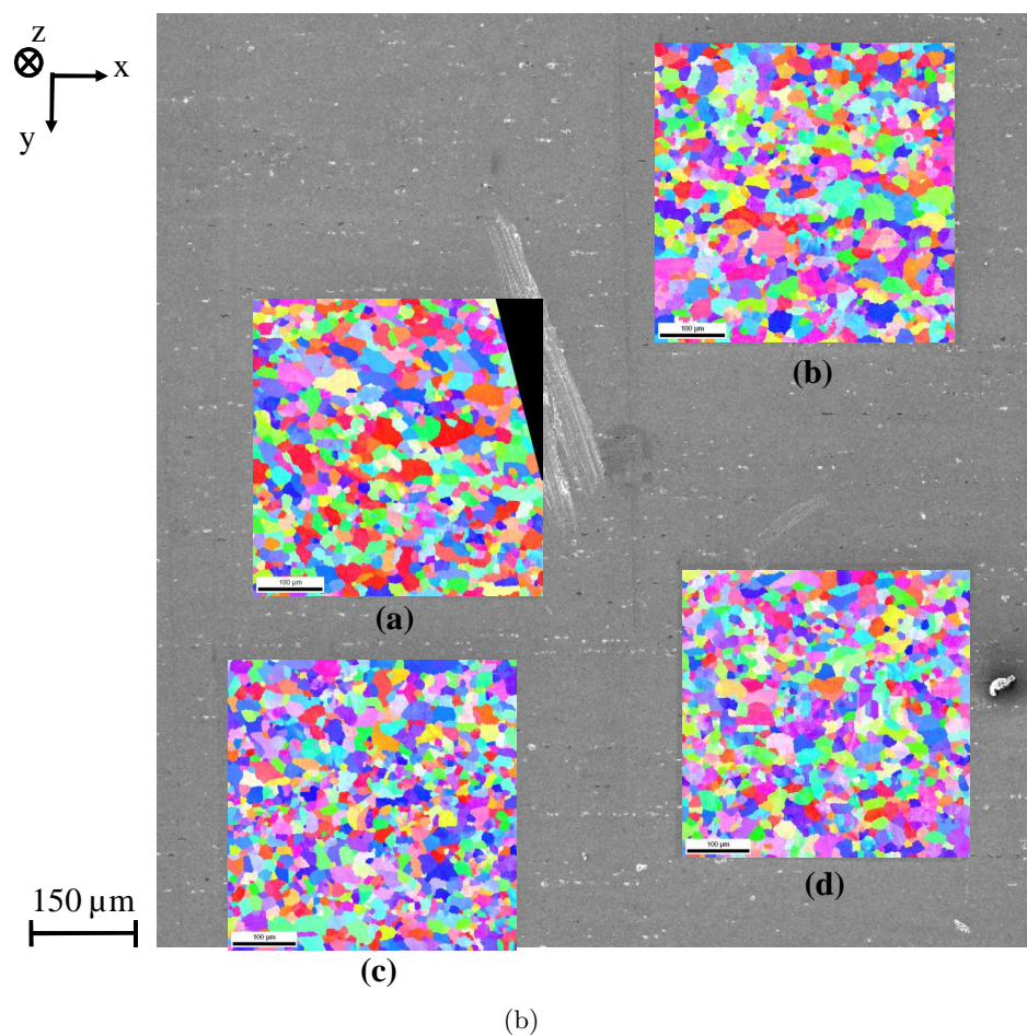
Figure 6.3: (a) surface slice obtained by microtomography and (b) corresponding EBSD maps and SEM micrographs. Here, the link between this two analysis tools was made with the central scratch as a fiducial mark.
