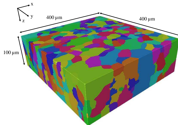
Figure 6.5: Recorded microstructure with a serial sectioning of 3 μm per step.
