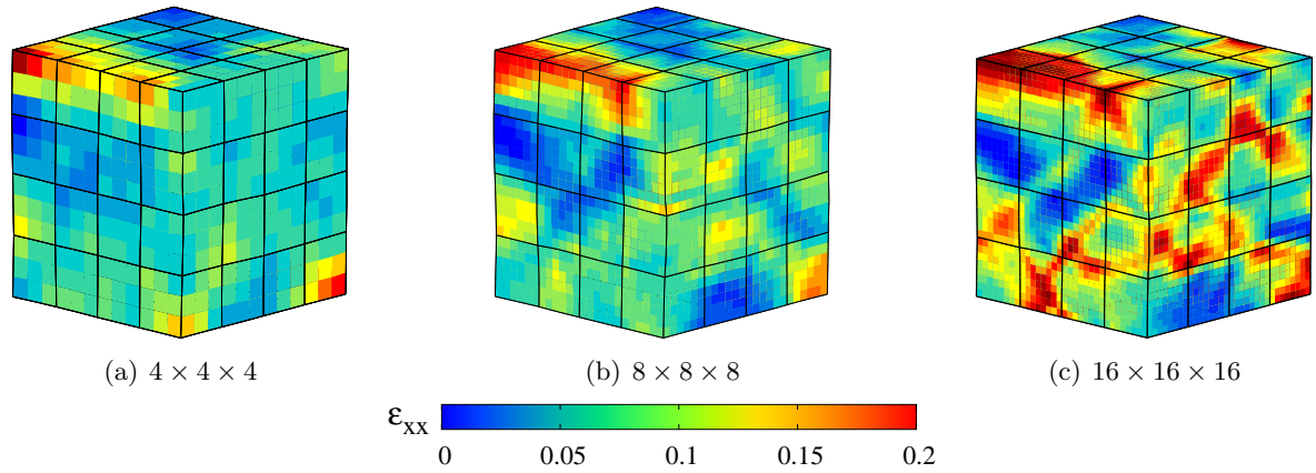
Figure 4.27: Accumulated plastic strain distribution after 10% applied strain
