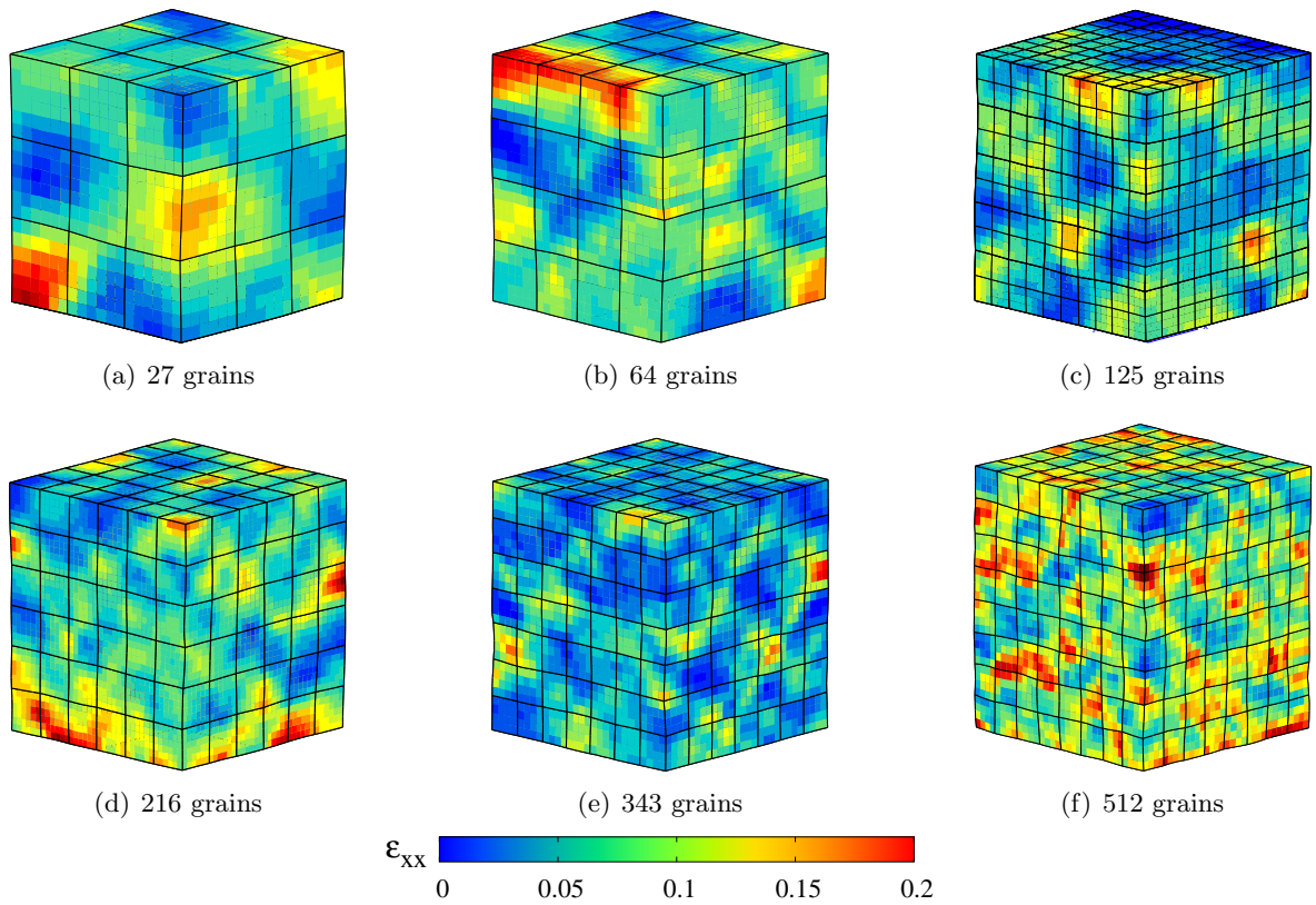
Figure 4.21: Accumulated plastic strain distribution after 10% applied strain
