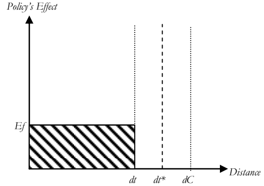
Figure 2a. Second case dt^* > dt
