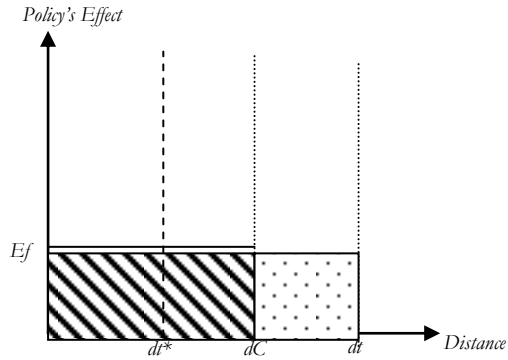
Figure 3a. Third case dt > dC
