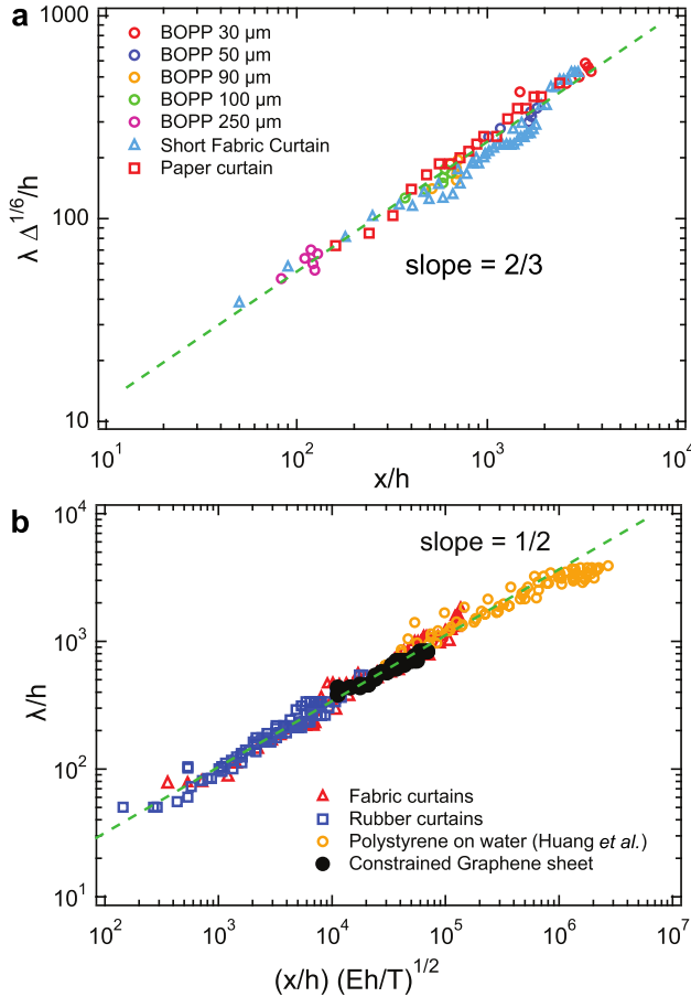
FIG. 3 (color online). Master curves gathering all data. (a) Normalized wavelength, \tilde{\lambda} = \lambda \Delta^{1/6}/h , as a function of the normalized distance, \tilde{x} = x/h , from the constrained edge for short light sheets (fabric curtain, paper curtain, and constrained plastic sheets). Dashed line: \tilde{\lambda} = 2.89\tilde{x}^{0.65} . (BOPP, biaxially oriented polypropylene). (b) Normalized wavelength \tilde{\lambda} = \lambda/h as a function of the normalized distance from the constrained edge \tilde{x} = (x/h)(Eh/T)^{1/2} for sheets under tension: fabric curtains, rubber curtains, suspended bilayer graphene sheet, and polystyrene thin films deposited on water from Ref. [14]. Dashed line: \tilde{\lambda} = 2.85\tilde{x}^{0.52} .
