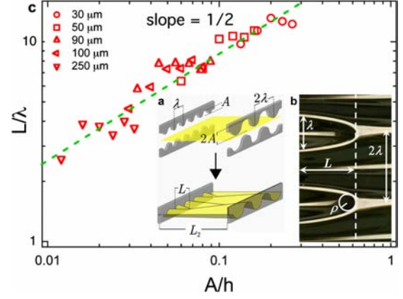
FIG. 2 (color online). (a) Schematic representation of the wrinkle experiments. (b) Morphology of the transition \lambda to 2\lambda for a constrained plastic sheet for A = 6 mm and \lambda = 8 mm. (c) Evolution of the normalized length of a wrinkle, L/\lambda , with the normalized amplitude, A/h (fixed wavelength, \lambda = 8 mm), for different thicknesses as indicated.
