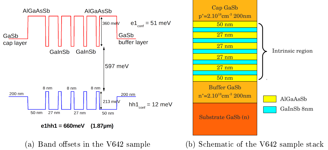
Figure 3.3: Band offset (a) and structure (b) of sample V642
