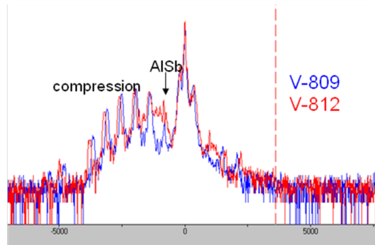
Figure 3.6: High resolution X-ray diffraction (HRXRD) measurements on strained samples V809 and V812
