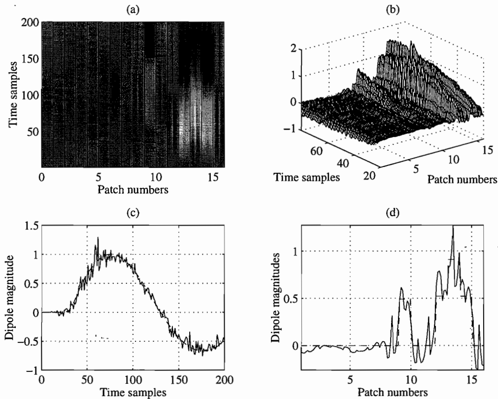
Figure 5 — Results of the LORETA method.
