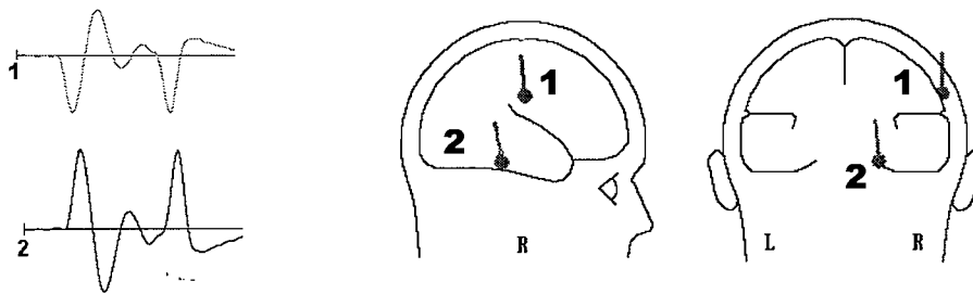
Figure 6 — Apparition of a phantom source when over-fitting the data to make the RV index decrease. Source 1 is very close to the original source location SI , while source 2 is a typical spurious or phantom source to account for the bias introduced by the simplified sphere model.
