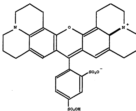
Sulforhodamine 101 Sulforhodamine 640
