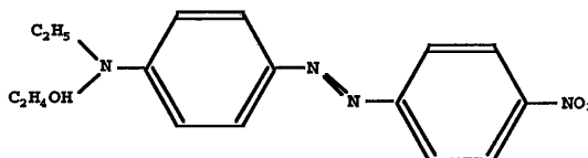
Disperse Red 1
