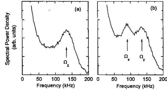
Figure 4. Intensity correlation spectrum of a lattice with \theta = 40^\circ : (a) observation along the z axis; (b) observation direction in the x - z plane at 10^\circ with respect to the z axis. The detected polarization was linear along y , and \Delta = -5\Gamma .
