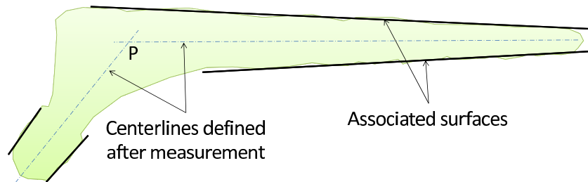
Figure A.3: Optimization through Root Mean Square criterion
