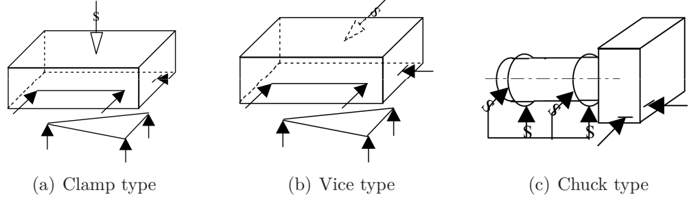
Figure 2.3: Clamping principles (Paris, 1995)
