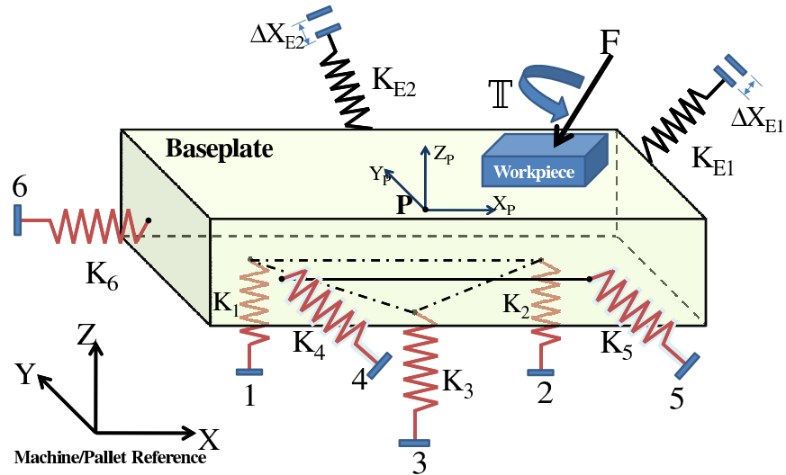
Figure 4.6: Modeling of clamps, XYZ: Pallet reference
