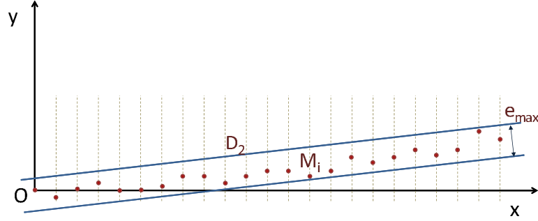
Figure 2.9: Association of measured points by Tchebychev criteria (Dursapt, 2009)
