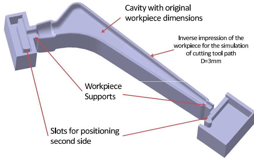
Figure 3.15: Inverse workpiece impression for simulation through boolean operation
