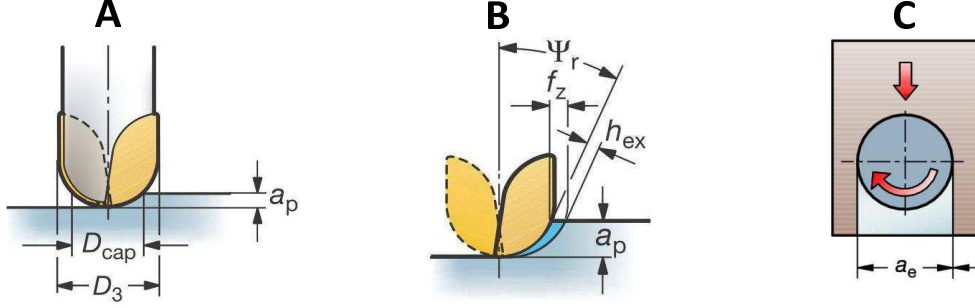
Figure 2.37: Ball nose end mill cutter (Sandviken, 2011)
