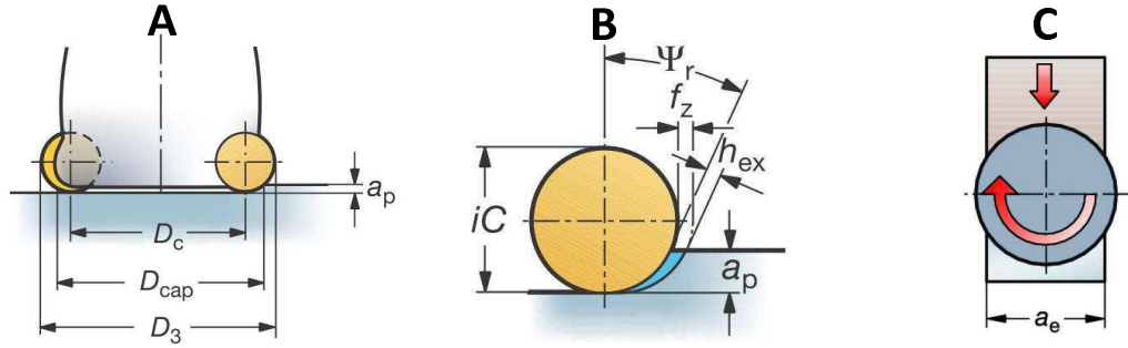
Figure 2.36: Round cutting edge cutter (Sandviken, 2011)
