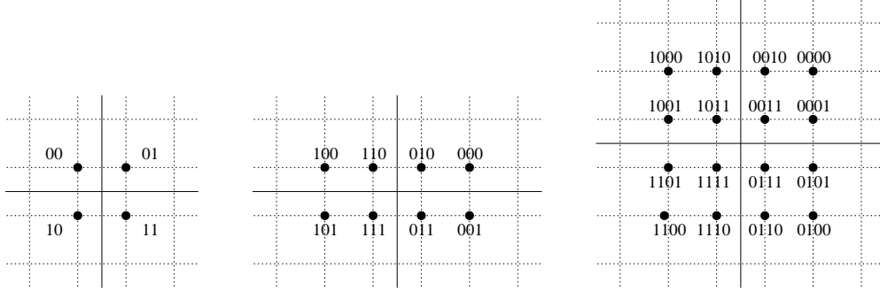
FIGURE 1.3 – Exemples de constellations q-QAM
