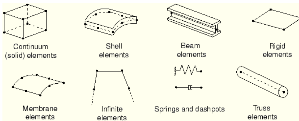
Fig.1. Finite element families used in analysis [6].
