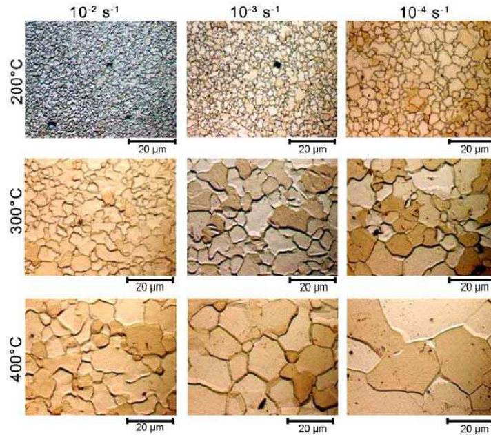
Fig.4. Optical micrographs specimens illustrating the DRX microstructure under uniaxial compression at various deformation conditions ranging from 200 to 400°C and 10^{-2} to 10^{-4} s ^{-1} [16].
