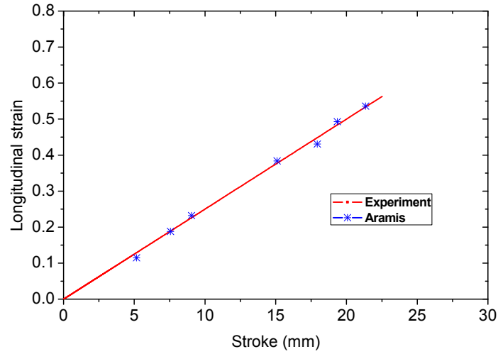
Fig.11 Comparison between the strains measured from the tensile set-up and ARAMIS system (200 0 C, 0.01s -1 )
