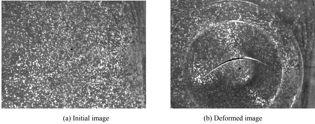
Fig.10. Test blank before and after deformation
