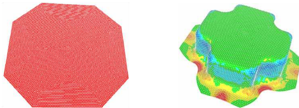
Fig.5. Initial mesh (left) and final mesh (right) after deep drawing process.
