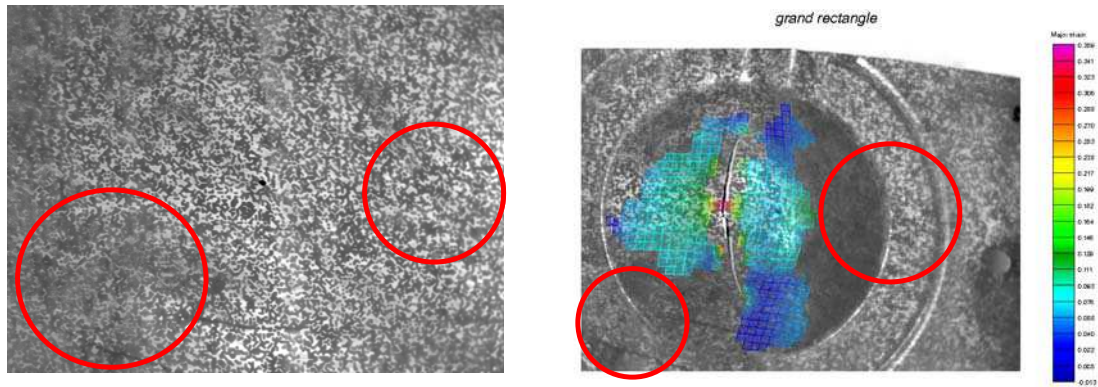
Fig.11. The calculation with bad grid pattern
