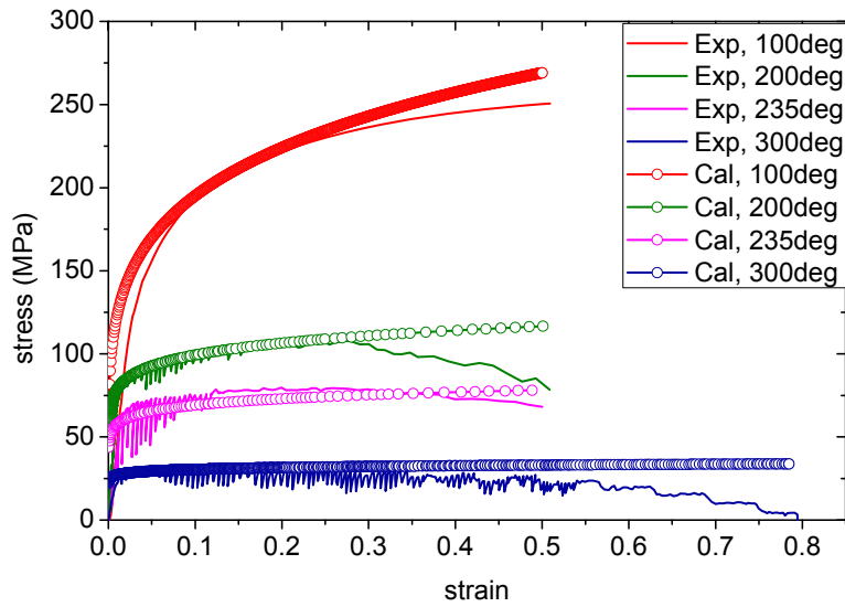
(b) \dot{\epsilon} = 0.001 \text{ s}^{-1}
