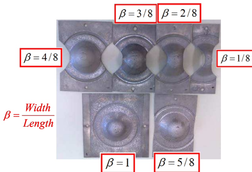
Fig.8. Specimens after Nakazima tests
