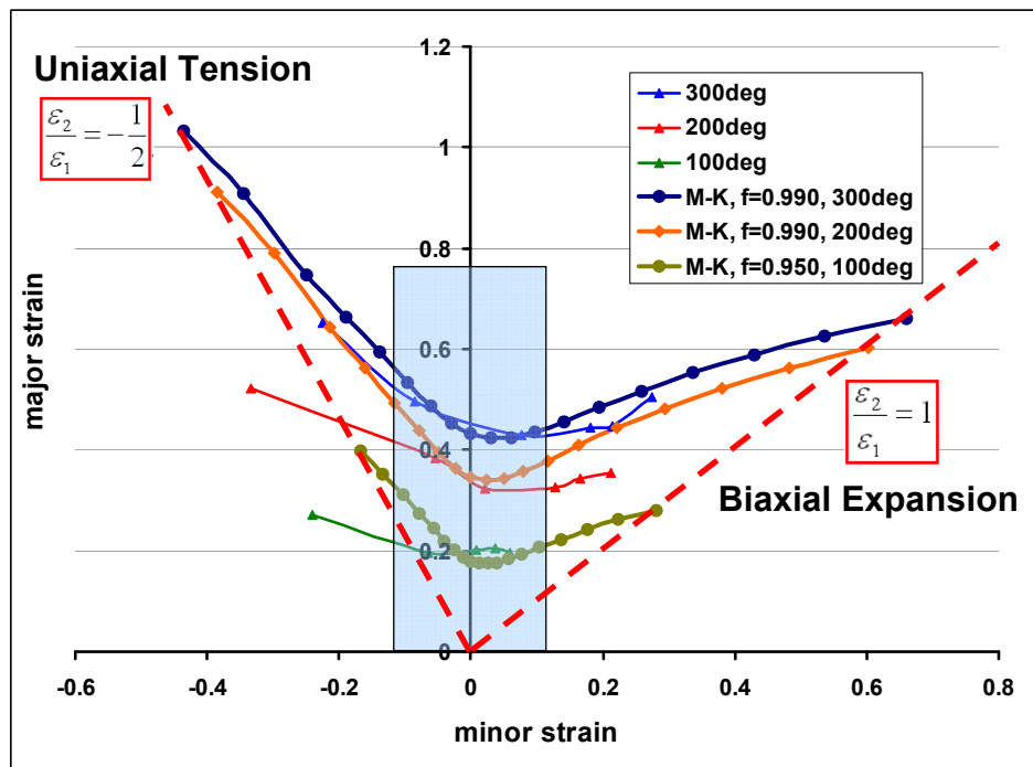
Fig.26. M-K prediction and experiment FLD comparison
