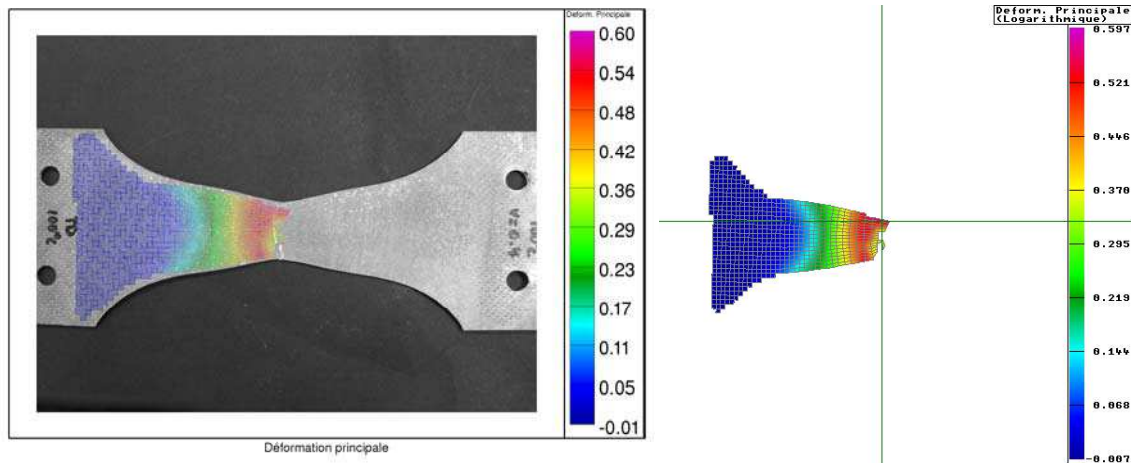
Fig.10. ARAMIS measurement at 100°C in transverse direction ( \dot{\epsilon} = 0.01s^{-1} )
