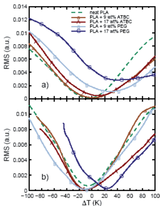
Figure 7. Root-mean-square distances (RMS) between 2D Field×Temperature spectra obtained in melt and after 18 days of exposure to probe vapors at 70 °C. Distances are plotted against different temperature shifts \Delta T of vapor spectra for: (a) TEMPOL and (b) AminoTEMPO spin probes. Corresponding spectra with minimal residues are plotted respectively in Figures 4 and 5.
