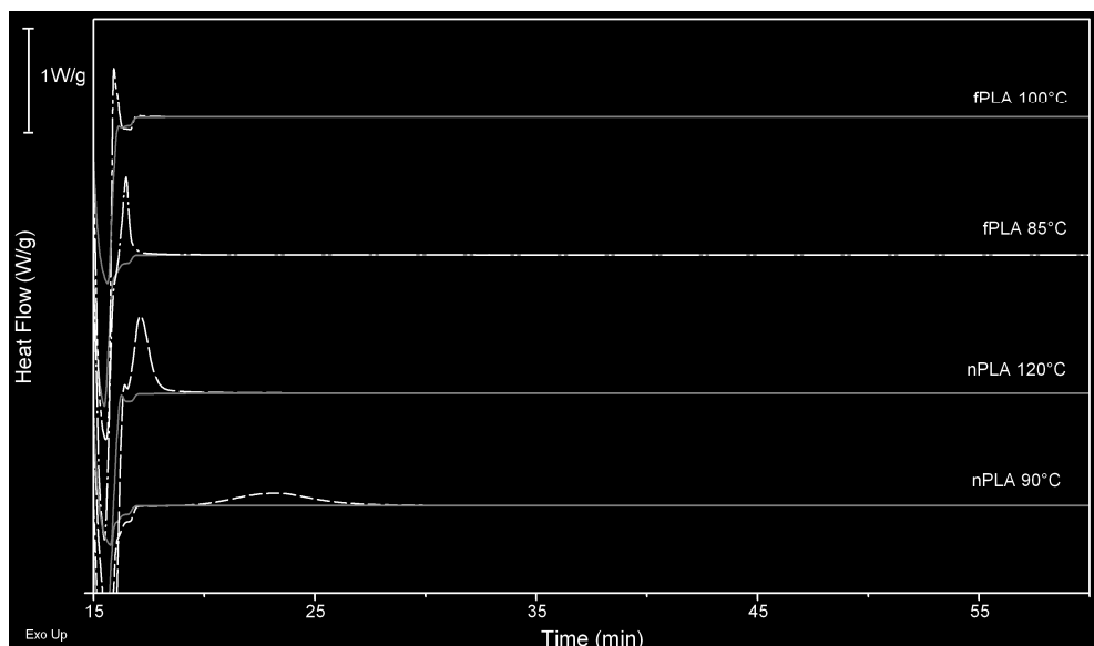
Figure 3. DSC thermograms for neat and formulated P(D,L)LA (black lines) during isothermal cold crystallization at 90 and 120 °C for neat P(D,L)LA and 85 and 100 °C for formulated P(D,L)LA. Baseline, obtained with sapphire at each crystallization temperature, are grey solid lines. The curves were vertically shifted for legibility.
