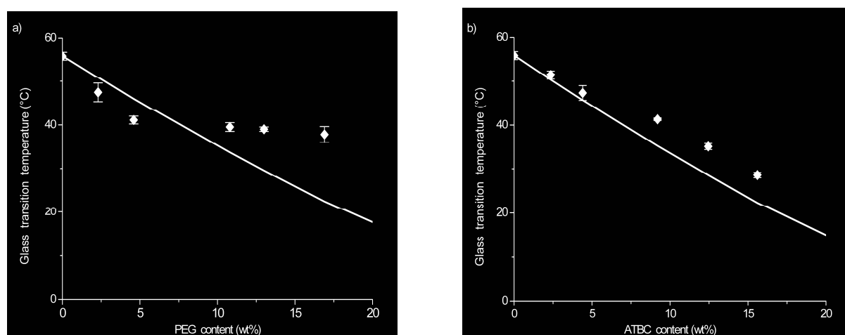
Figure 2. Glass transition temperature of P(D,L)LA/plasticizers: Experimental results ( \blacklozenge ) and Fox equation ( — ). (a), PEG 300/P(D,L)LA; (b), ATBC/P(D,L)LA.
