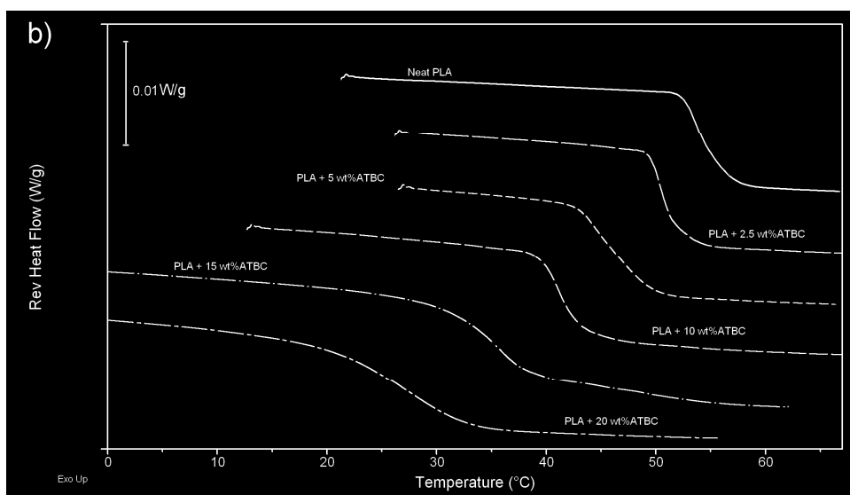
Figure 1b. MDSC thermograms for neat P(D,L)LA and formulated P(D,L)LA with ATBC heated at 1\text{ }^{\circ}\text{C}.\text{min}^{-1} . The curves were vertically shifted for legibility.
