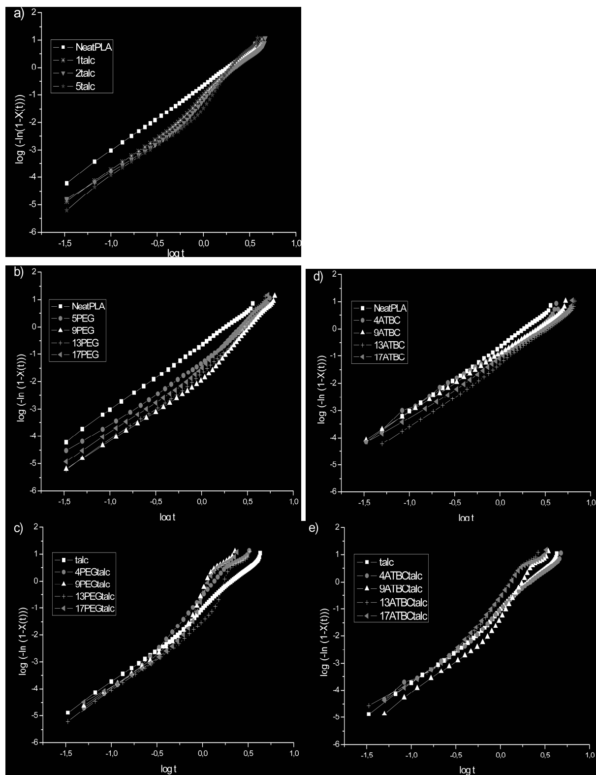
Figure 3. Plots of \log(-\ln(1-X(T))) versus \log t for non isothermal crystallization at 10\text{ }^{\circ}\text{C.min}^{-1} of (a) P(D,L)LA / talc, (b) P(D,L)LA / PEG, (c) P(D,L)LA / talc / PEG, (d) P(D,L)LA / ATBC and (e) P(D,L)LA / talc / ATBC.
