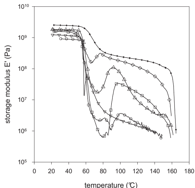
Figure 2. Evolution of the storage modulus with temperature of P(D,L)LA samples having different crystallinity. Symbols: extruded P(D,L)LA (o), quenched P(D,L)LA ( \square ), annealed P(D,L)LA 15 min 80 °C ( \triangle ), 15 min 85 °C ( \nabla ), 15 min 90 °C ( \diamond ), and 25 min 92 °C (+).
