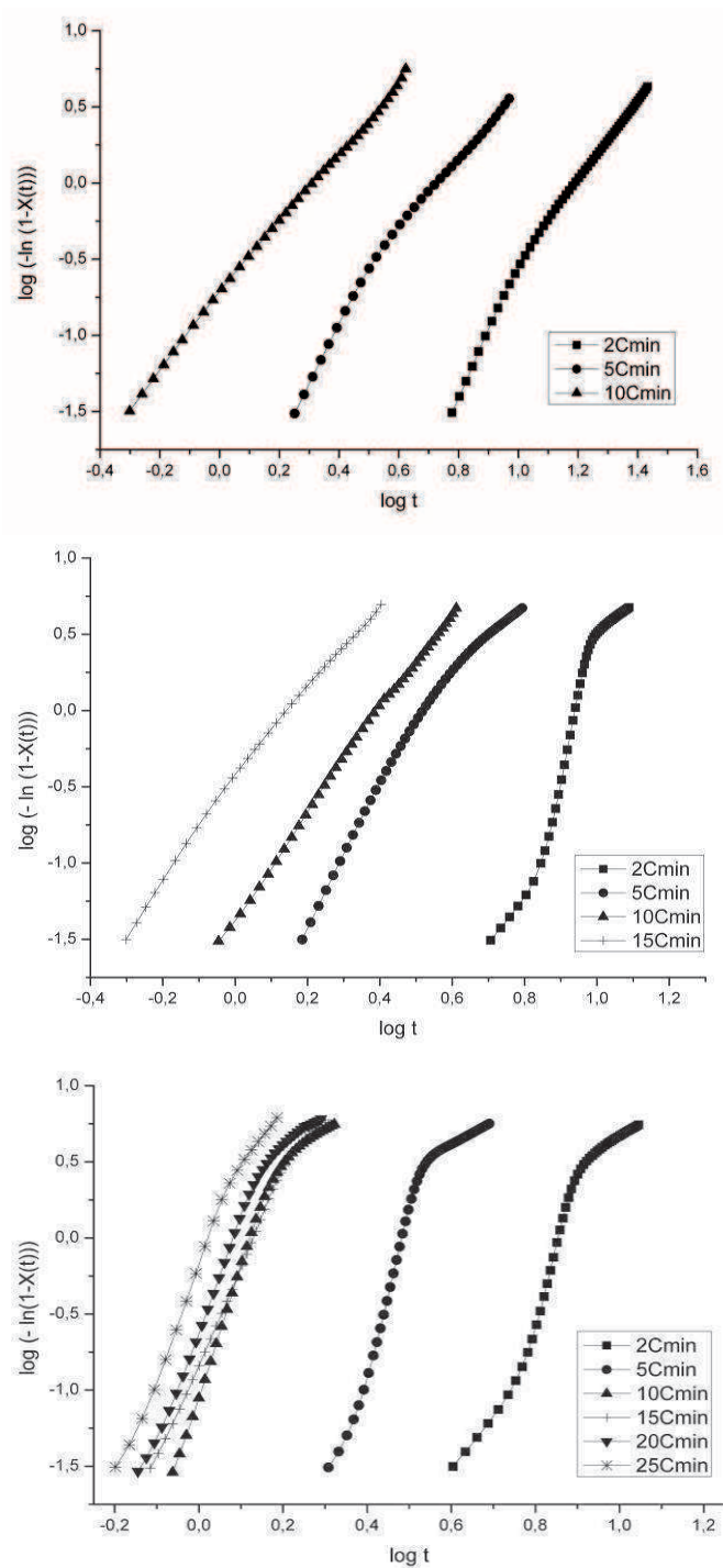
Figure 5. Plots of \log(-\ln(1-X(T))) versus \log t for non isothermal crystallization of (a) neat P(D,L)LA, (b) P(D,L)LA / talc and (c) P(D,L)LA / talc / 17 wt% ATBC.
