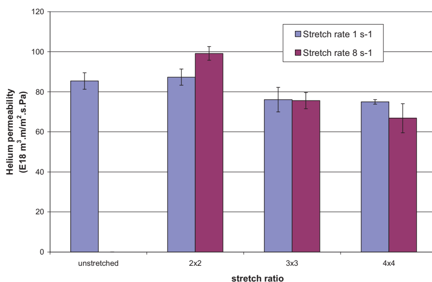
Figure 1. Evolution of helium permeability of P(D,L)LA 4042D drawn films as a function of the stretch ratio at two stretch rates, 1 s -1 and 8 s -1 .
