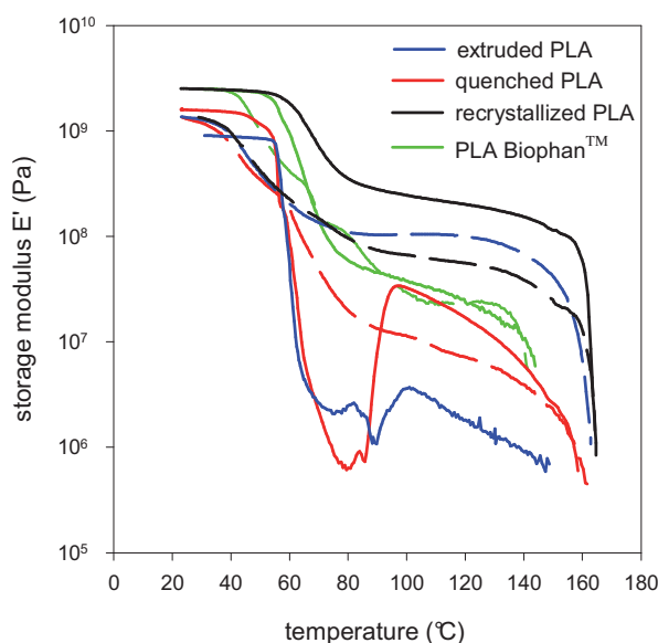
Figure 6. Thermo-mechanical properties of P(D,L)LA films before (solid line) and after conditioning (dashed line) in ethyl acetate atmosphere at an activity of 0.5 and 25 °C for 3 days.
