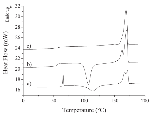
Figure 1. Heat flow curves of P(D,L)LA samples in the first heating cycle: a) extruded P(D,L)LA, b) quenched P(D,L)LA, c) recrystallized P(D,L)LA (92 °C/25 min).
