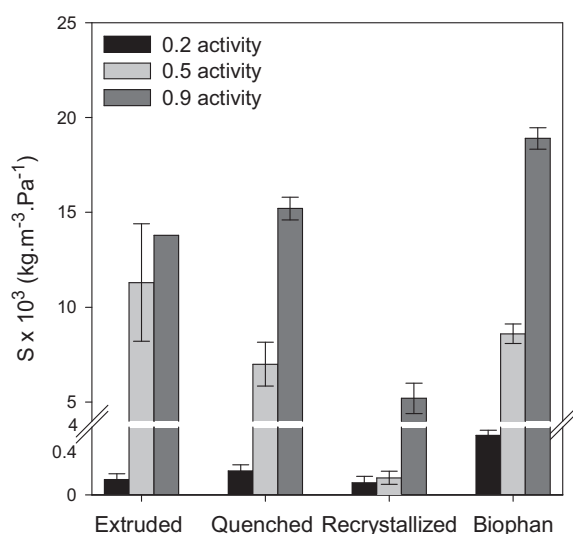
Figure 4. Apparent solubility coefficient ( S ) of ethyl acetate in P(D,L)LA samples with varying crystallinity at different activities ( p/p_0 ) at 25^\circ\text{C} . In order to display the small values, the ordinate was cut between 0.4 and 4 \cdot 10^{-3} \text{ kg.m}^{-3}.\text{Pa}^{-1} .
