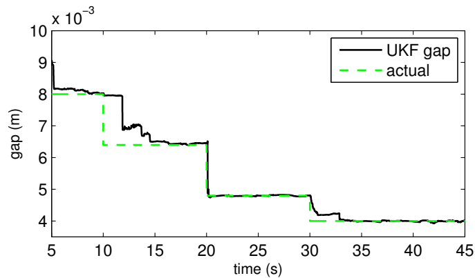
(b) Zoom on time window from t = 5 - 45\text{s}
