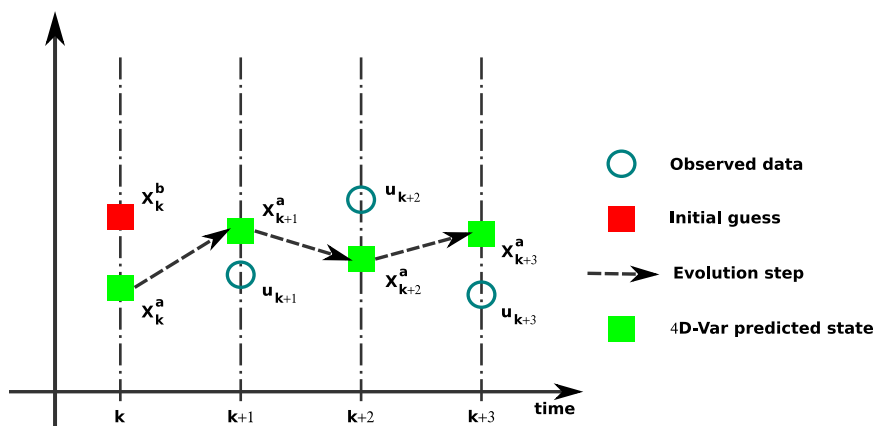
Figure 2.1: Principle of data assimilation by means of the 4D-Var approach.
