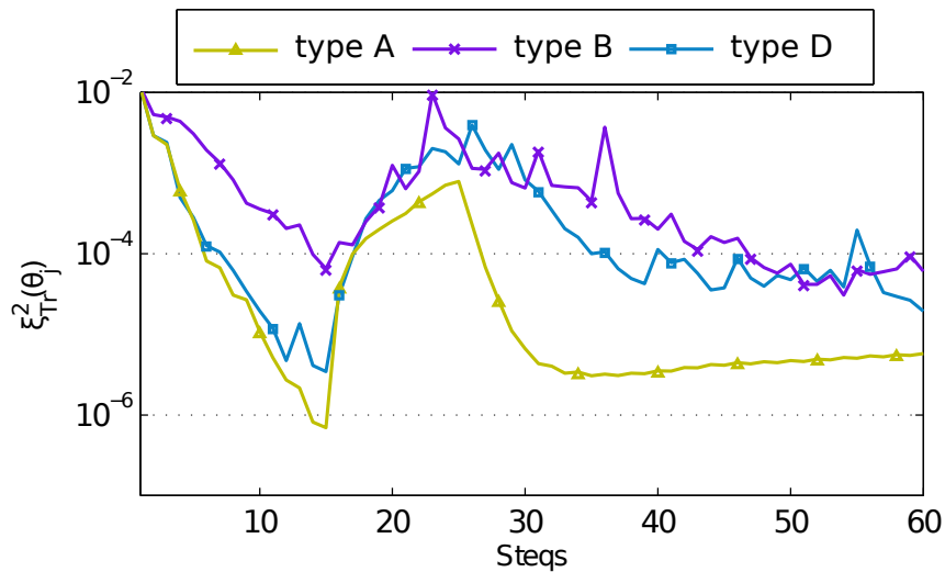
Figure 5.12: Comparison of \xi_{T_r}^2(\theta_j) residual along the ERC-UKF identification process for different designs of error noise covariance matrix Q in the case of evolving structural damage: type A ( \nu = 0.1 ), type B ( \kappa = 0.5 ) and type D ( \mu = 1.0 ).
