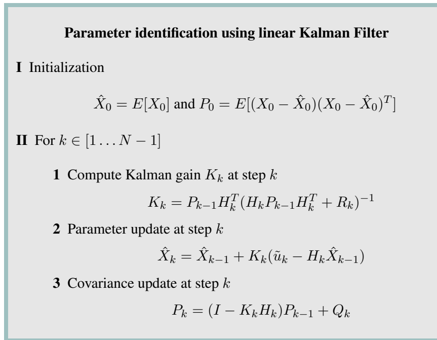
Figure 3.4: Linear Kalman Filter algorithm for parameter identification.
