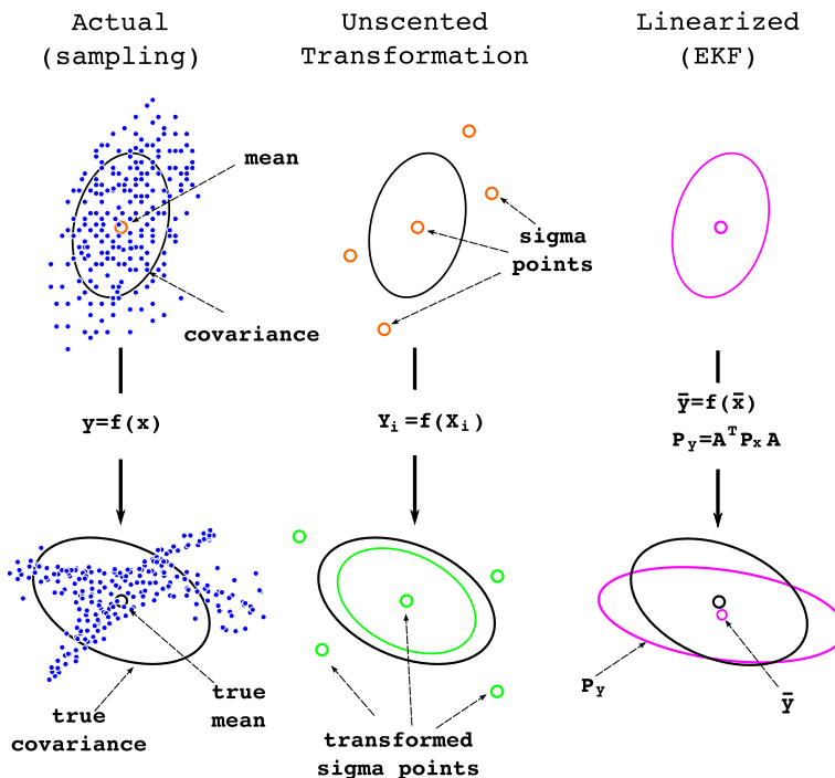
Figure C.1: Illustrative comparison between the Unscented and linearization methods for nonlinear stochastic transformations.
