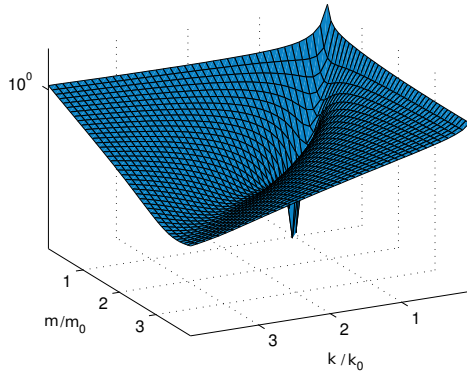
(b) ERC functional ( \xi_{Tr}^2 )
