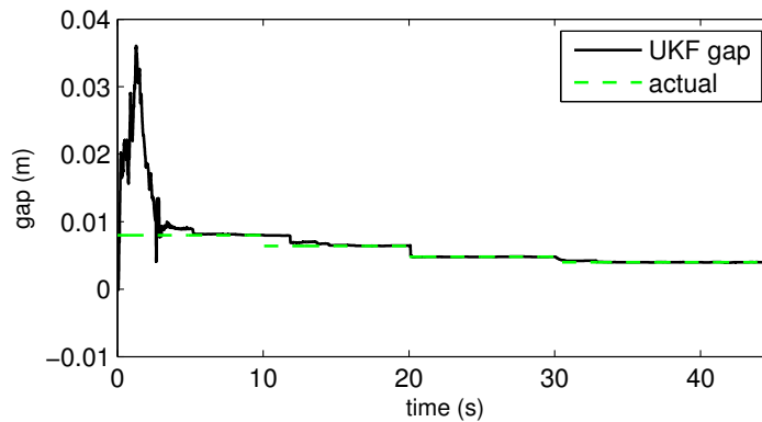
(a) Complete identification process
