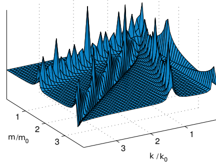
(c) Least squares functional \|\tilde{u} - \Pi q_{\text{direct}}\|^2
