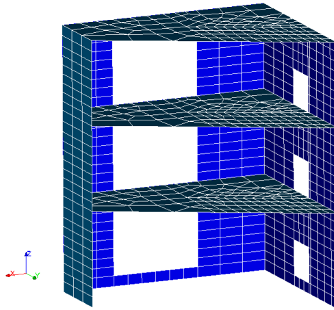
(b) Finite Element model
