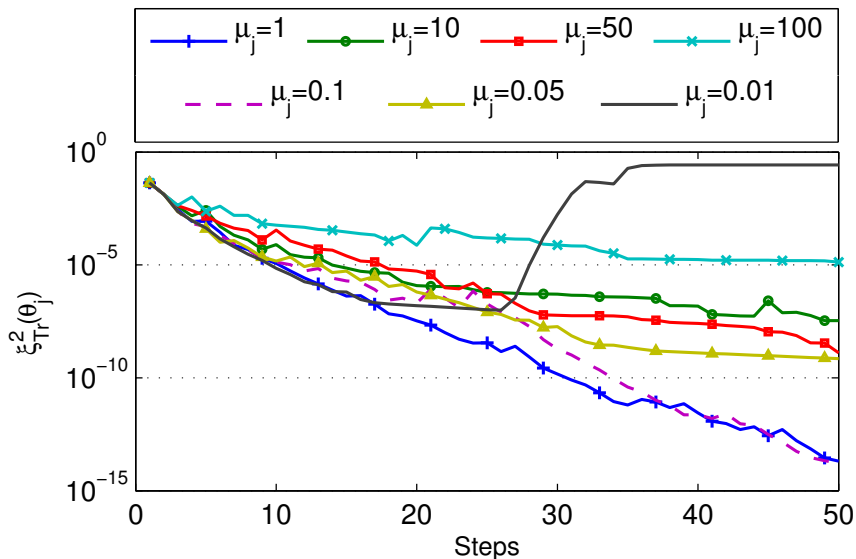
Figure 5.8: Comparison of \xi_{Tr}^2(\theta_j) residual along the ERC-UKF identification process for different values of \mu_j in a \mathcal{Q}_j = \mu \text{diag}(P_j^\theta) design (Type D).
