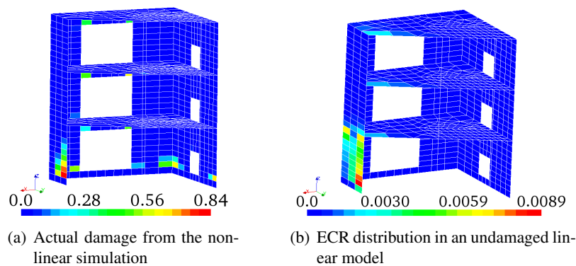
Figure 6.3: Results of an ECR analysis use to spatially localize nonlinear structural behavior (damage law).
