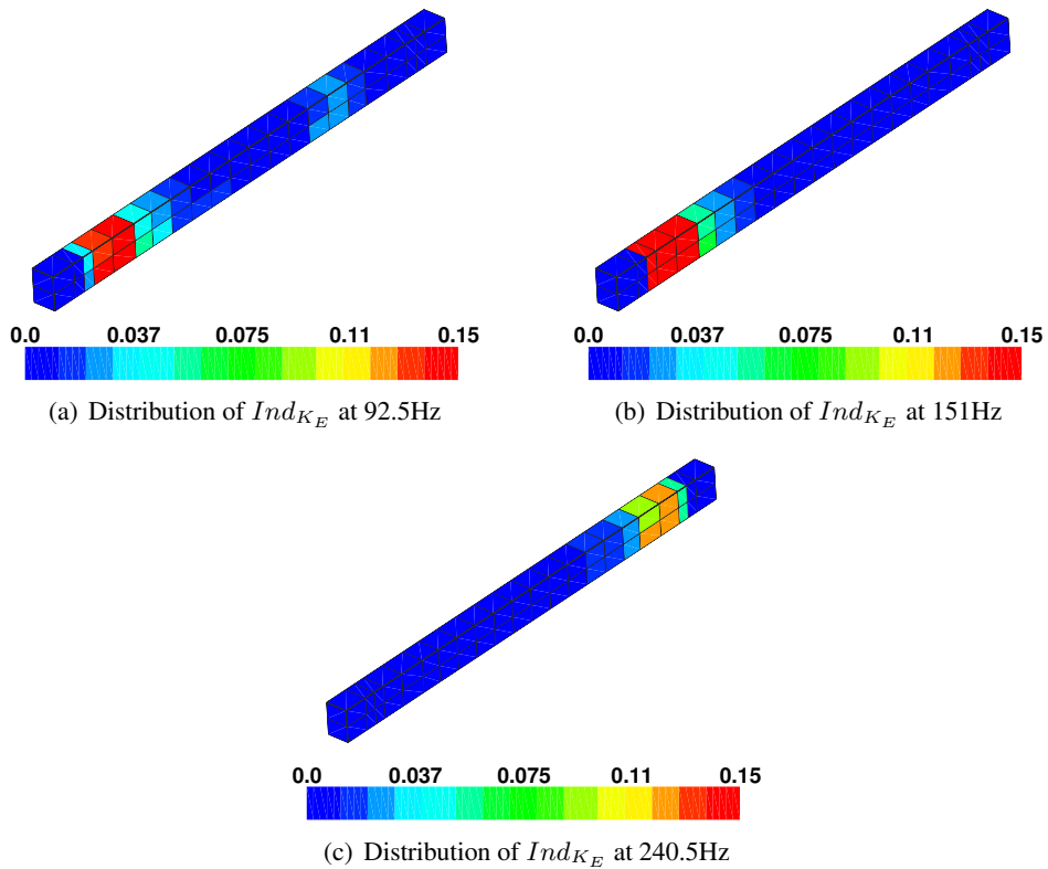
Figure 7.12: ECR analysis for the reinforced concrete beam FE model with boundary impedances. Distribution of Ind_{K_E} estimators over the structure at relevant peak error frequencies.
