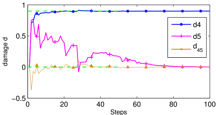
Figure 3.13: Identification of model parameters \theta defined in (3.23) by means of the ECR and UKF coupled strategy.
