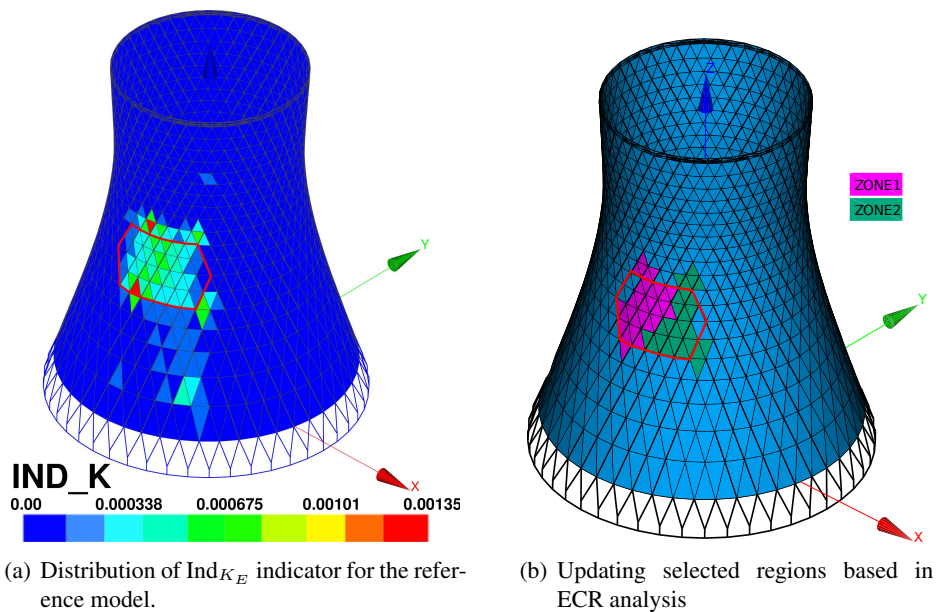
Figure 4.3: Results of the preliminary ECR analysis over the power plant cooling tower FE model.
