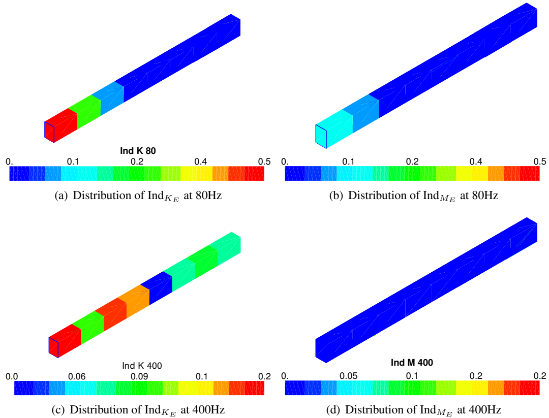
Figure 4.18: Preliminary ECR analysis for a perfect double-clamped concrete beam FE model. Distribution of IndK and IndM estimators over the structure for different frequencies.
