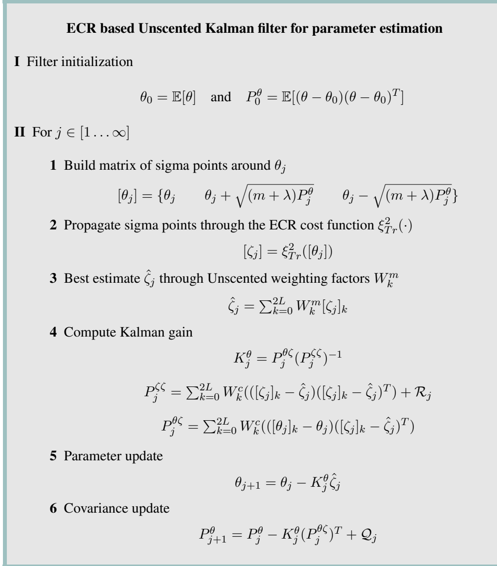
Figure 3.7: Description of the Unscented Kalman filter with ECR cost functions in observation space for minimization purpose.
