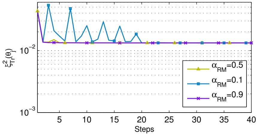
Figure 5.9: Comparison of \xi_{Tr}^2(\theta_j) residual along the ERC-UKF identification process for different values of \alpha_{RM} in a Robbins-Monro modeling of Q_j (Type C).
