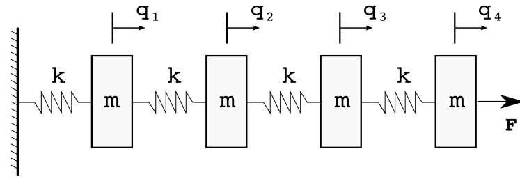
(a) 4-DOF system definition
