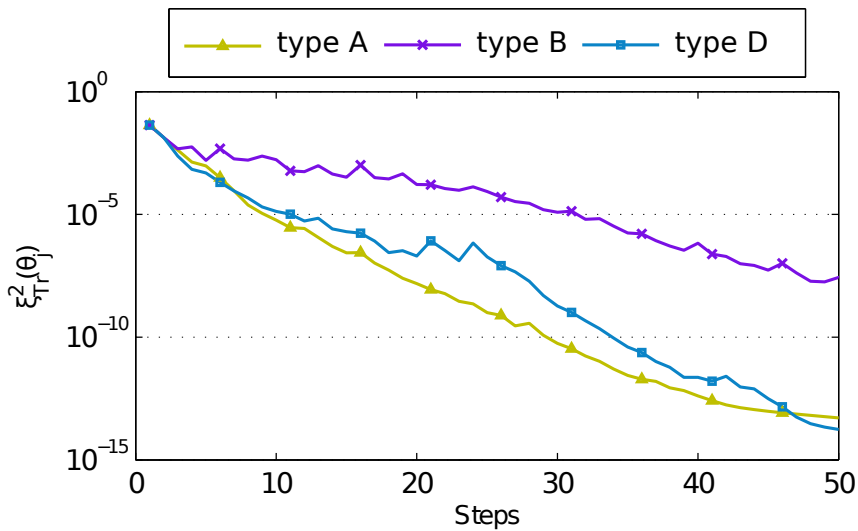
Figure 5.10: Comparison of \xi_{Tr}^2(\theta_j) residual along the ERC-UKF identification process for different designs of error noise covariance matrix Q : type A ( \nu = 0.1 ), type B ( \kappa = 0.5 ) and type D ( \mu = 1.0 ).
