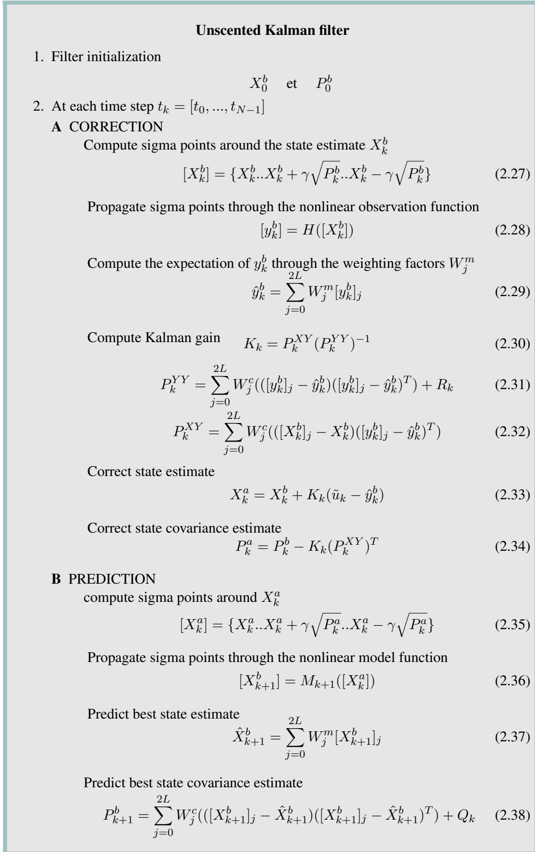
Figure 2.7: Sequential Unscented Kalman filter equations for nonlinear system estimation.
