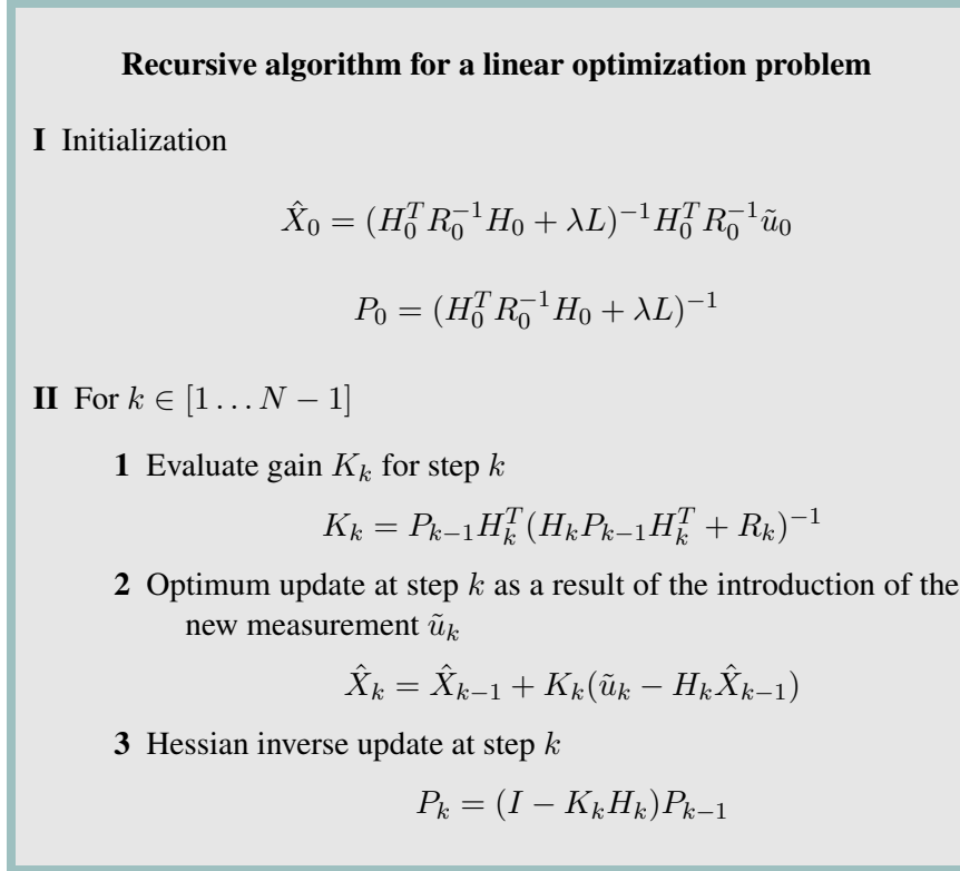
Figure 3.3: Recursive algorithm solving a least square optimization problem for linear systems.
