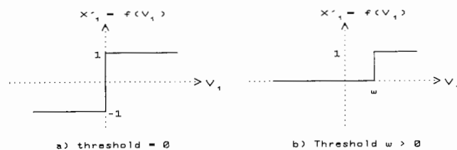
Fig. 3. Transfer function of the thresholding amplifier in the feedback loop of neuron i : (a) zero threshold; (b) positive threshold \omega .
