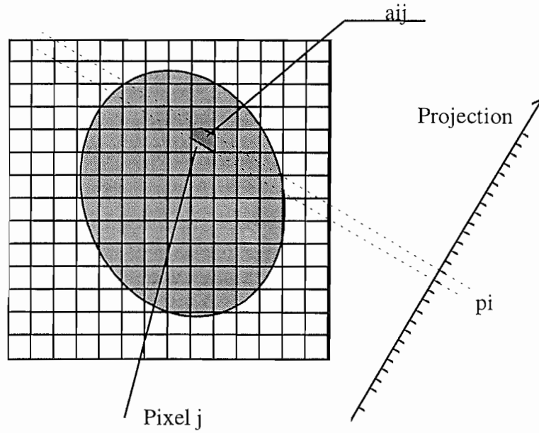
Figure II-15: Champ de reconstruction discret.
