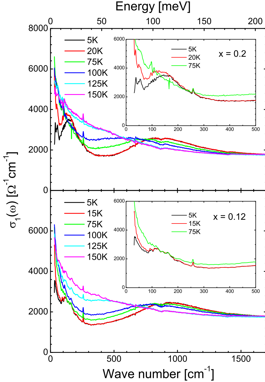
Figure 6.20: The top panel shows the optical conductivity of \text{Ba}_{1-x}\text{K}_x\text{Fe}_2\text{As}_2 ( x = 0.2 ) below 1700\text{ cm}^{-1} at several temperatures. The inset displays the enlarged view of \sigma_1(\omega) at low frequencies. The bottom panel shows the same spectra for the x = 0.12 sample.
