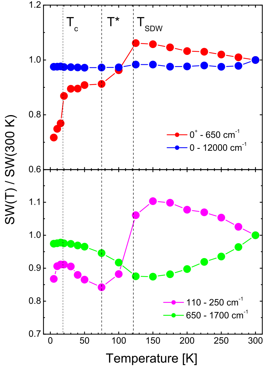
Figure 6.21: Temperature dependence of the spectral weight, SW_a^b = \int_a^b \sigma_1(\omega) d\omega , normalized by its value at 300 K, for Ba_{1-x}K_xFe_2As_2 ( x = 0.2 ) sample. a and b represent the lower and upper cut-off frequencies respectively. The vertical dashed lines denote T_c , T^* and T_{SDW} respectively.
