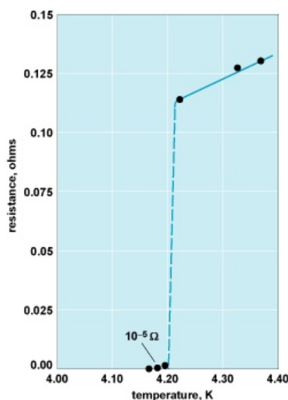
Figure 2.1: The resistance of Hg as a function of temperature measured by Kamerlingh Onnes.
