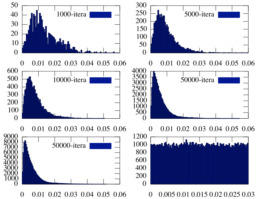
Figure 6.9: Histograms of the distance d(\hat{x}_i, x_i) . The denoising algorithm applied with parameters \delta = 3\varepsilon and \tau = 3 , in all cases. The last histogram shows d(y_i, x_i) .
