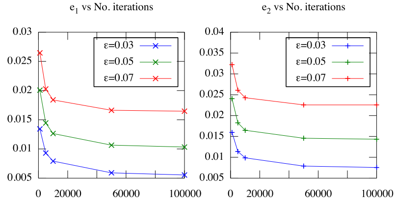
Figure 6.8: Denoising algorithm applied with parameters \delta = 3\varepsilon and \tau = 3 . Left: We plot e_1 versus the number of iterations. Right: The plot shows e_2 versus the number of iterations.
