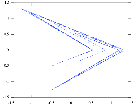
Figure 1.1: Simulation of the Lozi attractor for the parameters a=1.7 and b=0.5 .
