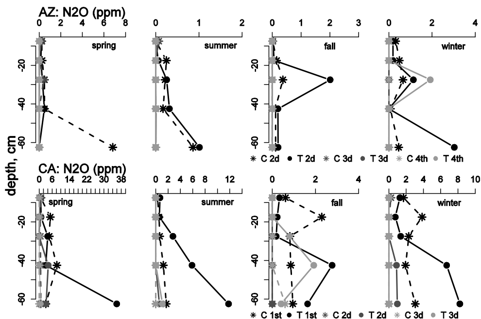
Fig. 3 Averaged soil air \text{N}_2\text{O} contents by depth, treatment, season and number of year after compaction (3 replicates \times about 4 sampling times per season, depth, treatment and number of year after compaction): AZ, Azerailles; CA, Clermont en Argonne; C, control treatment; T, trafficked treatment; 1st, 2d, 3d, 4th, first, second, third and fourth year after compaction
