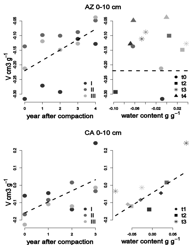
Figure 5 Evolution of the difference in soil V between trafficked (T) and undisturbed (C) soil and selected linear mixed model (dotted lines) explaining it as a function of the number of year after heavy traffic and as a function of the difference in soil water content between T and C. In each panel the second covariate (time after compaction or water content) is held constant at its arithmetic mean. Only the results of the 0-10 cm soil layer are shown as it is the only soil layer where we observed a significant evolution with time for both sites. The different colours correspond to the blocks (I, II and III) and the different symbols to the years after disturbance (t0, t1, t2, t3, t4 relating to immediately, one year, two years, three years and four years following the forwarder traffic respectively).
