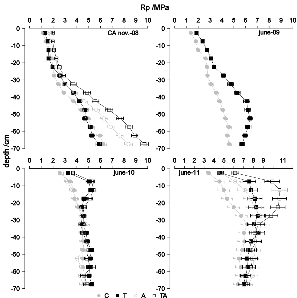
Figure 6 Soil resistance to penetration ( R_p ) as a function of depth, sampling time and treatment (C, control; T, trafficked; A, control amended; TA, trafficked amended), measured at the CA (Clermont en Argonne) site (90 replicates per treatment, except in June 2011 where only 45 profiles were measured per treatment). Mean and standard errors as errors bars
