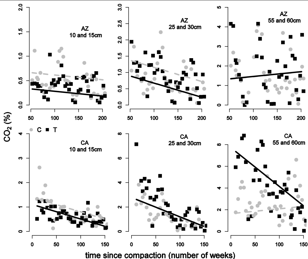
Fig. 5 Evolution of soil air \text{CO}_2 content (dots) at the Azerailles (AZ) and Clermont en Argonne (CA) sites, the lines correspond to the linear models explaining this evolution as a function of time following treatment (C, control; T, trafficked) application, treatment, soil air-filled porosity and soil temperature; each covariate being constant, equal to its arithmetic mean per site and depth (both treatments confounded)
