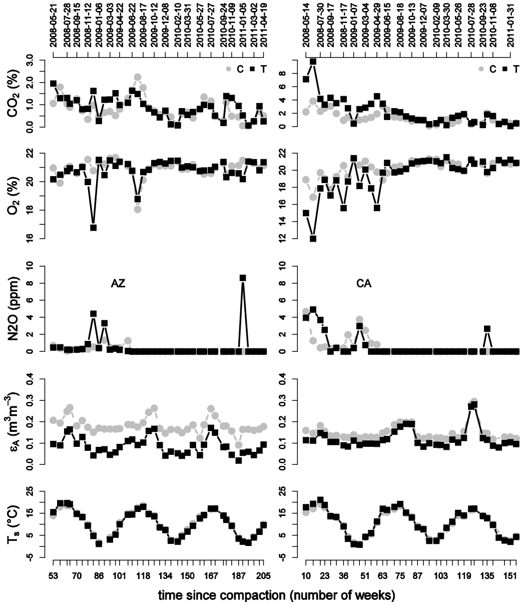
Fig. 4 Concurrent evolution of soil air CO 2 , O 2 , and N 2 O contents (average of the measurements of the three blocks per site), soil air-filled porosity (ε A ) and soil temperature (T s ) at 30 cm in the control (C) treatment and 25 cm depth in the trafficked (T) treatment, in the Azerailles (AZ, left side) and Clermont en Argonne (CA, right side) sites, soil water content and temperature are measured only in one block (five replicates), bulk density (nine replicates) and soil air composition (three replicates) measured in the three blocks
