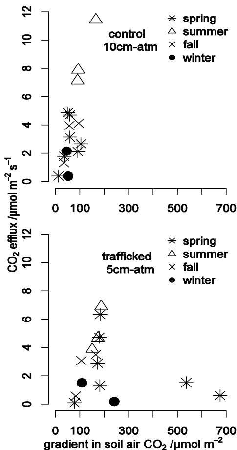
Figure 3 Soil CO 2 efflux of the 'Hauts Bois' forest site from March 2008 to March 2010 as a function of \Delta[\text{CO}_2] : see Equation (2)
