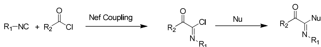
Scheme IV.6: 3-CR involving imidoyl halide from acyl chloride and isocyanides.
