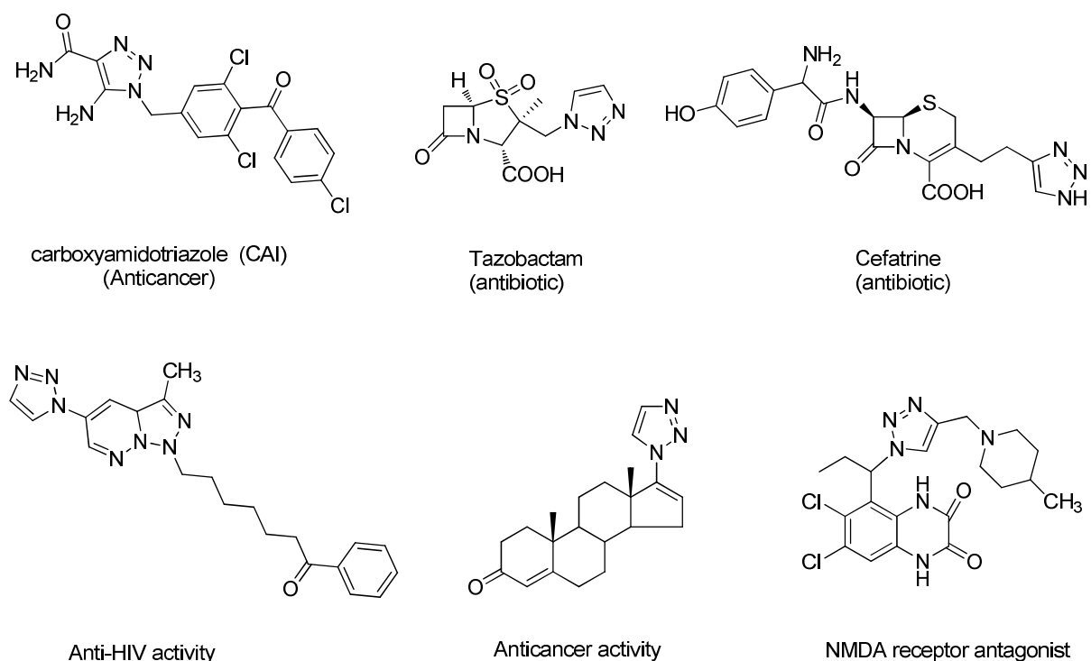
Figure V.1: Potential pharmaceuticals based on 1,2,3-triazoles.
