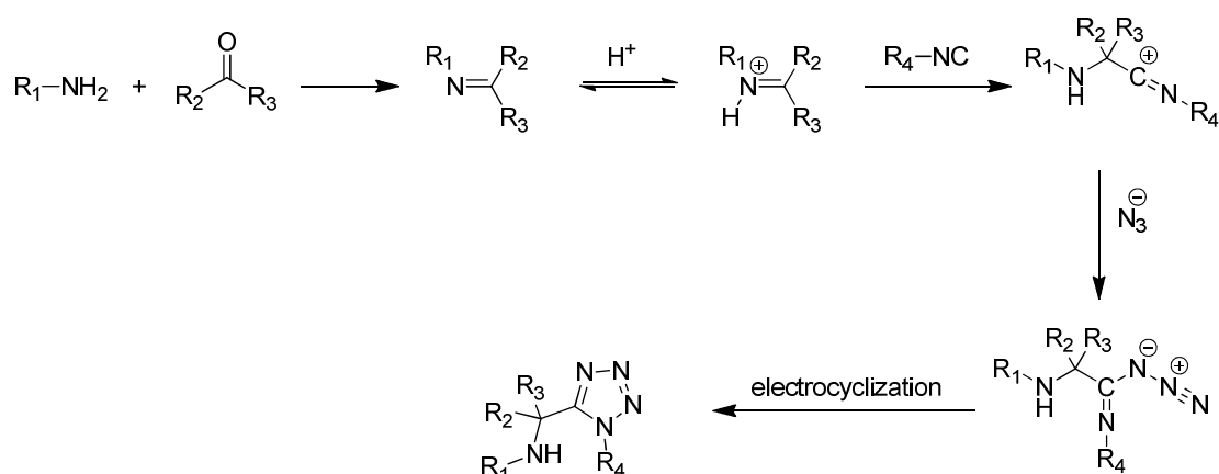
Scheme V.1: Mechanism of the tetrazole-U-4CR.
