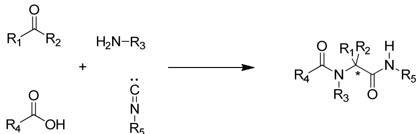
Scheme I.25 : Ugi Reaction.
