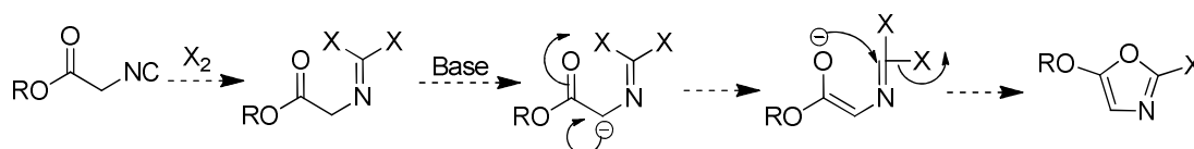
Scheme IV.26: Proposed path for halogeno-oxazole.
