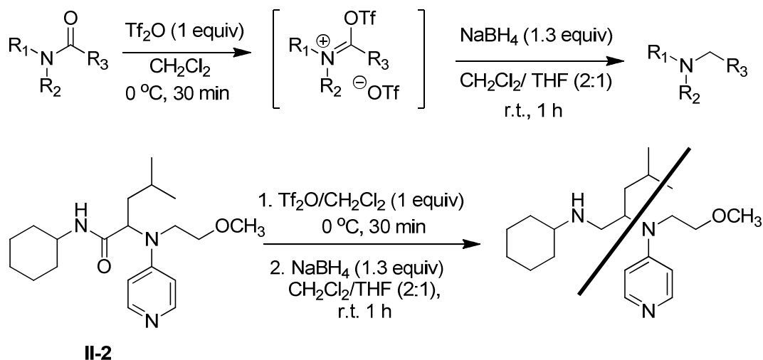
Scheme II.30: Reduction of Ugi-Smiles adduct with Tf 2 O and NaBH 4 .
