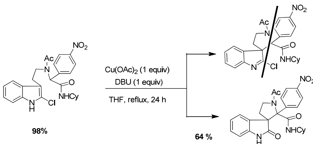
Scheme III.43. Synthesis of spirooxindole from oxidation of Ugi adduct with Cu(II).
