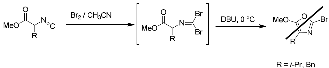
Scheme IV.30: Attempted synthesis of oxazole from valine and phenylalanine derivatives.
