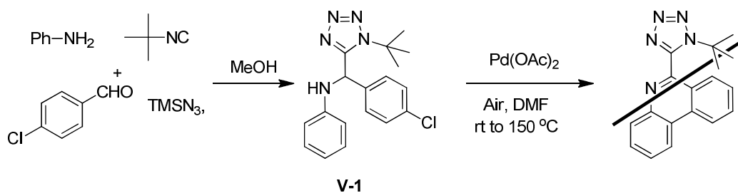
Scheme V.7: First trial of electrocyclization.
