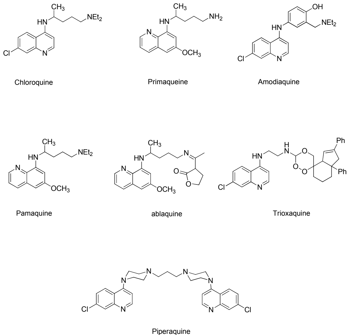
Scheme II.10: The promising antimalarial drugs and active precursors. 69
