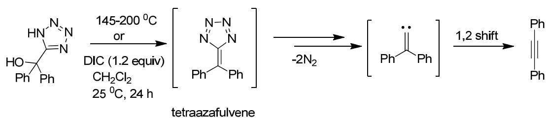
Scheme V.19: Synthesis of alkynes from 5-hydroxyalkyl-1 H -tetrazole by thermolysis.
