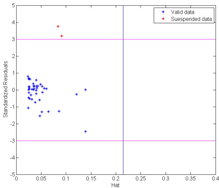
Figure 7.19: Detection of the probable doubtful experimental data 214 and the applicability domain of the applied correlation for the CO 2 + CH 4 clathrate hydrate system in the L w -H-V region. The H* value is 0.214.
