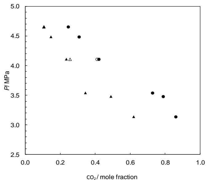
Figure 6.5: Pressure-composition diagram for the methane + carbon dioxide + water system under L_w -H-G equilibrium at 280.2 K. Experimental: y_{CO_2} (▲); 426 This work: z_{CO_2} (●). CSMGem model 2 predictions: y_{CO_2} (Δ); z_{CO_2} (○).
