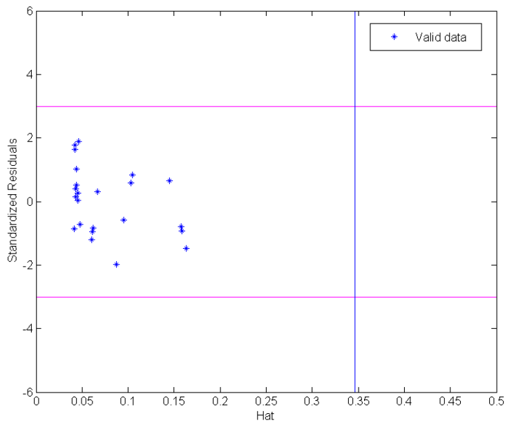
Figure 7.16: Detection of the probable doubtful experimental data 527 and the applicability domain of the applied correlation for the CO 2 + CH 4 clathrate hydrate system in the L w -H-V region. The H* value is 0.346.
