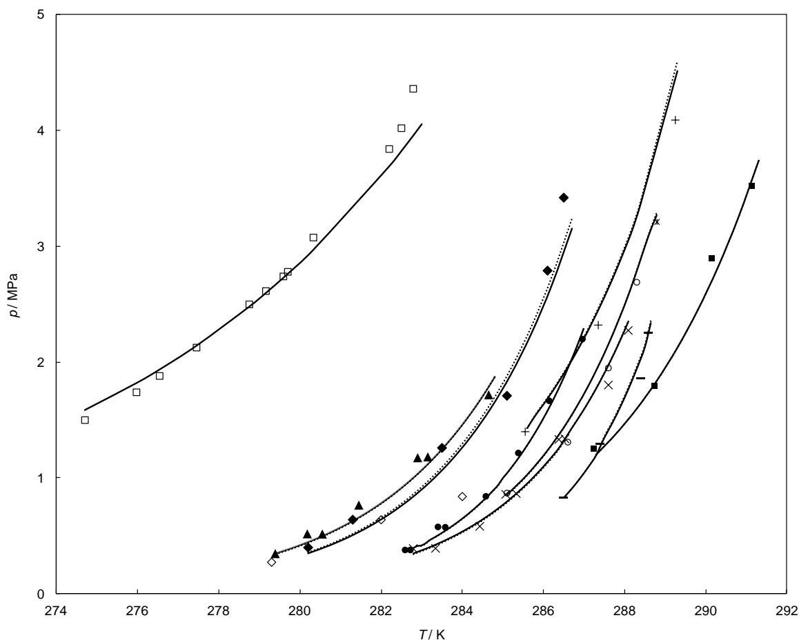
Figure 4.3: Dissociation conditions of clathrate/semi-clathrate hydrates for the carbon dioxide + water/TBAB aqueous solution systems. Symbols stand for experimental data and curves (lines) refer to the predicted values using the developed thermodynamic model. \square , CO 2 + water system; 215,323,418,419 \blacktriangle , CO 2 in the presence of 0.0443 mass fraction TBAB aqueous solution; 392 \blacklozenge , CO 2 in the presence of 0.05 mass fraction TBAB aqueous solution; 420 \diamond , CO 2 in the presence of 0.05 mass fraction TBAB aqueous solution; 204 \bullet , CO 2 in the presence of 0.0702 mass fraction TBAB aqueous solution; 392 \times , CO 2 in the presence of 0.0901 mass fraction TBAB aqueous solution; 392 + , CO 2 in the presence of 0.10 mass fraction TBAB aqueous solution; 421 \circ , CO 2 in the presence of 0.10 mass fraction TBAB aqueous solution; 420 \blacksquare , CO 2 in the presence of 0.427 mass fraction TBAB aqueous solution; 421 - , CO 2 in the presence of 0.40 mass fraction TBAB aqueous solution; 257 Solid curves, model predicted results assuming the formation of type B semi-clathrate hydrates (AARD = 7.7 %); Dashed curves, model predicted results assuming the formation of type A semi-clathrate hydrates (AARD = 8.2 %).
