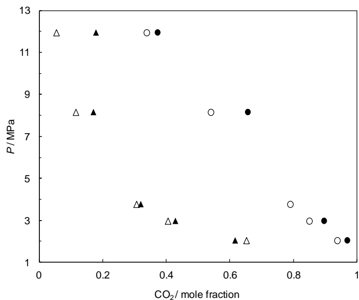
Figure 6.6: Pressure-composition diagram for the nitrogen + carbon dioxide + water system under L_w -H-G equilibrium at 273.6 K. Experimental: y_{CO_2} (▲); 59 This work: z_{CO_2} (●). CSMGem model 2 predictions: y_{CO_2} (Δ); z_{CO_2} (○).
