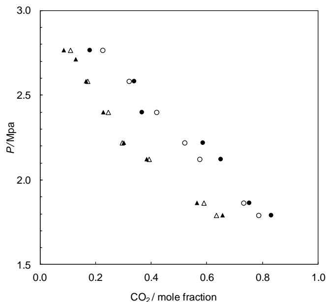
Figure 6.2: Pressure-composition diagram for the methane + carbon dioxide + water system under L_w -H-G equilibrium at 275.2 K. Experimental: yCO_2 ( \blacktriangle ); 426 This work: zCO_2 ( \bullet ). CSMGem model 2 predictions: yCO_2 ( \triangle ); zCO_2 ( \circ ).
