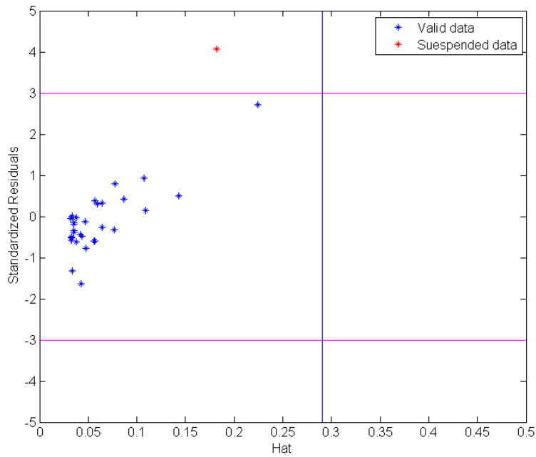
Figure 7.18: Detection of the probable doubtful experimental data 217 and the applicability domain of the applied correlation for the CO 2 + CH 4 clathrate hydrate system in the L w -H-V region. The H* value is 0.290.
