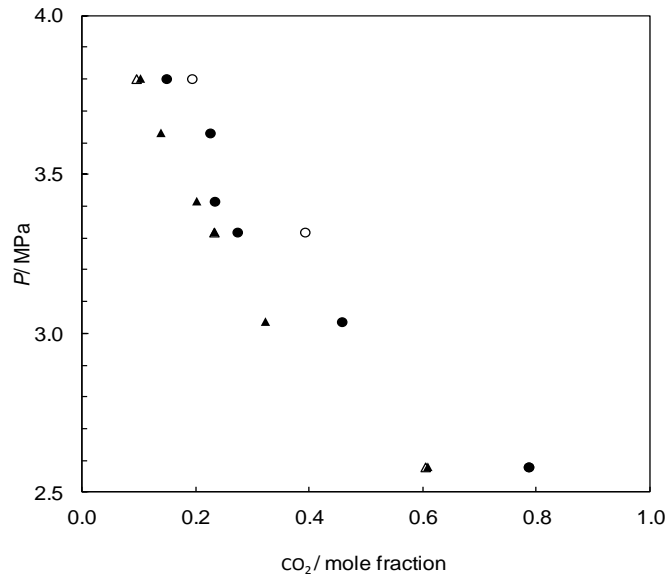
Figure 6.4: Pressure-composition diagram for the methane + carbon dioxide + water system under L w -H-G equilibrium at 278.1 K. Experimental: yCO 2 (▲); 426 This work: zCO 2 (●). CSMGem model 2 predictions: yCO 2 (Δ); zCO 2 (○).
