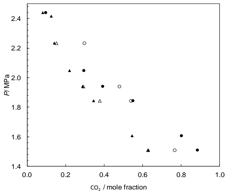
Figure 6.1: Pressure-composition diagram for the methane + carbon dioxide + water system under L_w -H-G equilibrium at 273.6 K. Experimental: yCO_2 ( \blacktriangle ); 426 This work: zCO_2 ( \bullet ). CSMGem model 2 predictions: yCO_2 ( \triangle ); zCO_2 ( \circ ).
