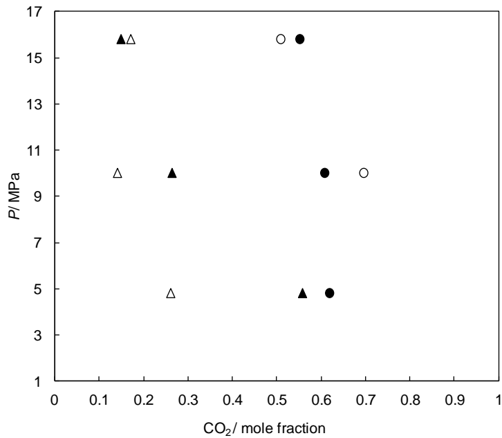
Figure 6.10: Pressure-composition diagram for the nitrogen + carbon dioxide + water system under L w -H-G equilibrium at 279.7 K. Experimental: yCO 2 (▲); 59 This work: zCO 2 (●). CSMGem model 2 predictions: yCO 2 (Δ); zCO 2 (○).
