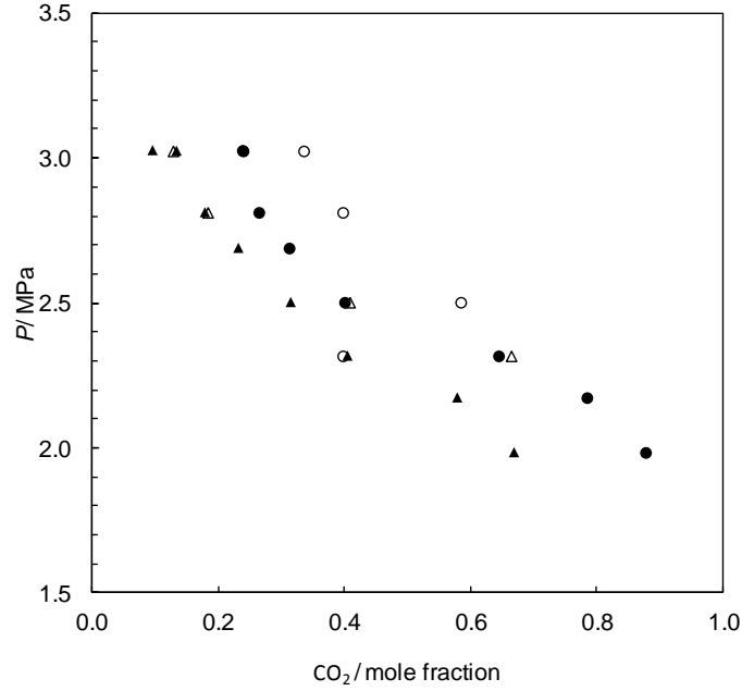
Figure 6.3: Pressure-composition diagram for the methane + carbon dioxide + water system under L w -H-G equilibrium at 276.1 K. Experimental: yCO 2 (▲); 426 This work: zCO 2 (●). CSMGem model 2 predictions: yCO 2 (Δ); zCO 2 (○).
