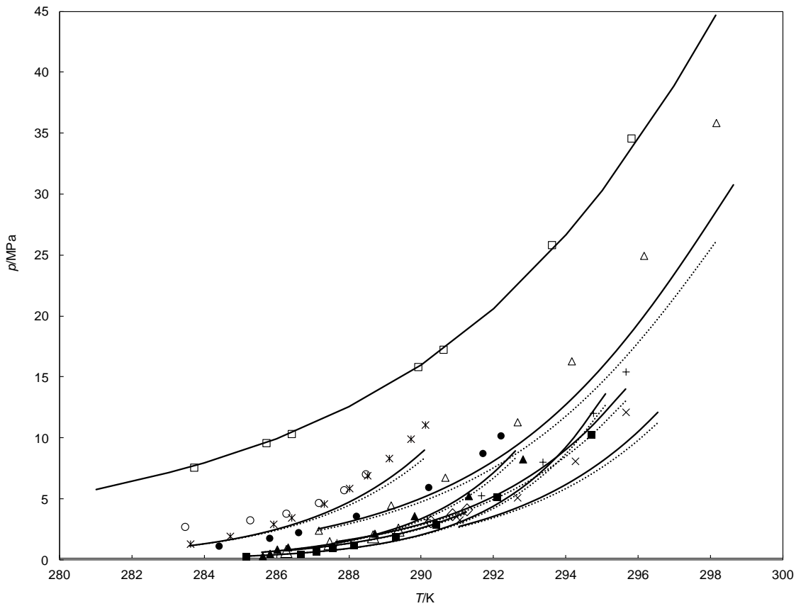
Figure 4.4: Dissociation conditions of clathrate/semi-clathrate hydrates for the methane + water/TBAB aqueous solution systems. Symbols stand for experimental data and curves (lines) refer to the predicted values using the developed thermodynamic model. \square , \text{CH}_4 + water system; 323 * , \text{CH}_4 in the presence of 0.05 mass fraction TBAB aqueous solution; 422 \circ , \text{CH}_4 in the presence of 0.05 mass fraction TBAB aqueous solution; 25 \bullet , \text{CH}_4 in the presence of 0.10 mass fraction TBAB aqueous solution; 58 \Delta , \text{CH}_4 in the presence of 0.10 mass fraction TBAB aqueous solution; 421 \blacktriangle , \text{CH}_4 in the presence of 0.50 mass fraction TBAB aqueous solution; 58 + , \text{CH}_4 in the presence of 0.20 mass fraction TBAB aqueous solution; 421 \diamond , \text{CH}_4 in the presence of 0.45 mass fraction TBAB aqueous solution; 25 \blacksquare , \text{CH}_4 in the presence of 0.25 mass fraction TBAB aqueous solution; 58 \times , \text{CH}_4 in the presence of 0.30 mass fraction TBAB aqueous solution; 421 Solid curves, model predicted results assuming the formation of type B semi-clathrate hydrates (AARD = 5.6 %); Dashed curves, model predicted results assuming the formation of type A semi-clathrate hydrates (AARD = 13 %).
