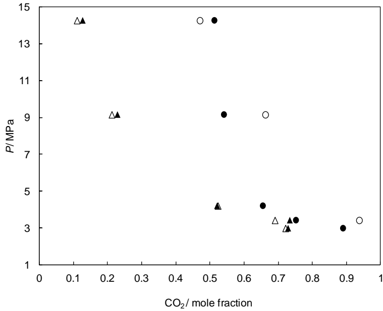
Figure 6.9: Pressure-composition diagram for the nitrogen + carbon dioxide + water system under L w -H-G equilibrium at 278.1 K. Experimental: yCO 2 (▲); 59 This work: zCO 2 (●). CSMGem model 2 predictions: yCO 2 (Δ); zCO 2 (○).
