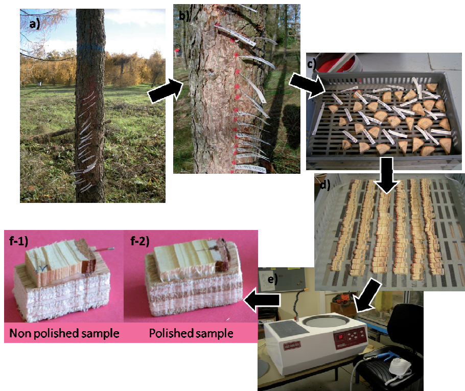
Figure 8.- Sample preparation. a) View of inserted pins on a sampled tree at the end of 2006 growing season. b) Detail of pins. c and d) reduction process of wood samples. e) Machine used to polish wood samples. f-1) view of wood sample ready to polish. f-2) view of polished sample
