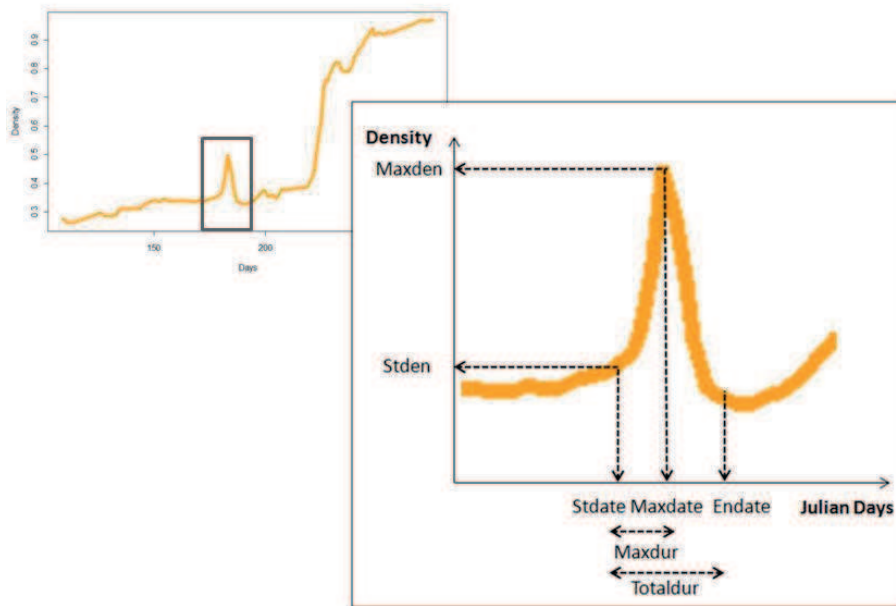
Figure 13.- Detailed measurements on a false ring extracted from a dynamic wood density profile (tree P008 at PEY): Sdate: Julian day when false ring peak started; Maxdate when it reached its maximum density and Endate when it ended; Stdén, Maxden and Enden: corresponding wood densities; Totaldur: total duration of peak and Maxdur: number of days up to the reach of maximum peak density.
