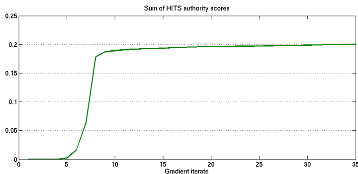
Figure 7.4: Optimization of the sum of HITS authority scores. The figure shows that the objective is increasing during the course of the algorithm. The sum of authority values jumps from 2.1e-6 to 0.19. Of note, the sum of authority values for a clique (all internal links activated) is 4.8e-6 . The algorithm thus gives with a small computational effort a much better solution than what is commonly considered a good strategy [LM00]. However, despite this big progress at the beginning, convergence is slow. This is a typical situation with first order methods and nonconvex optimization.
