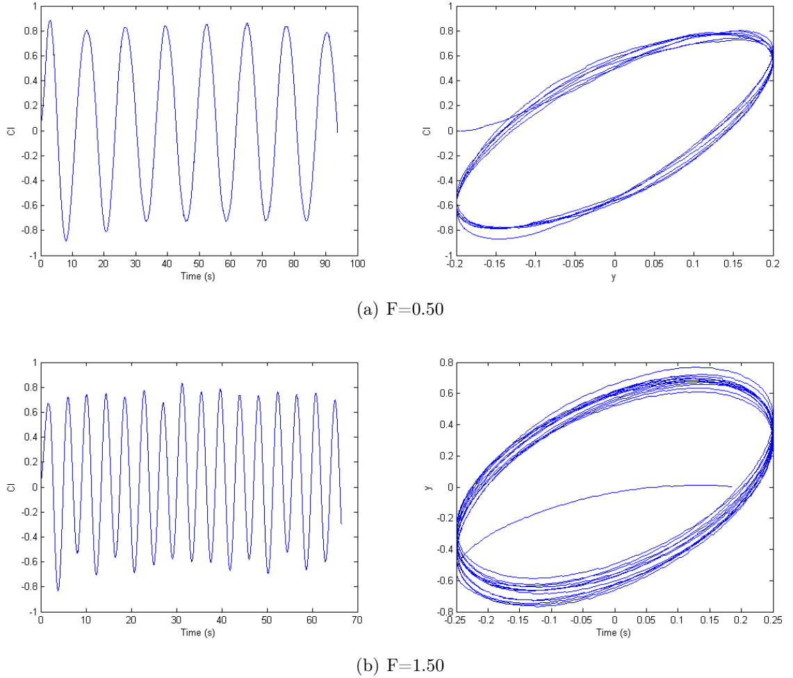
Figure A.12: Time series of fluctuation lift coefficient C'_L , and phase portraits at F = 0.50 F = 1.50
