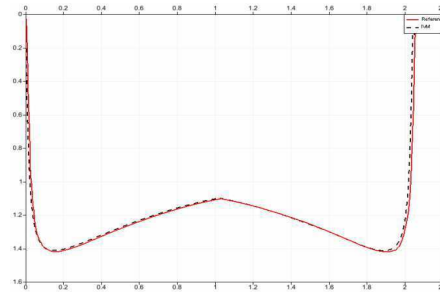
Figure 3.49: Comparisons of the pressure coefficients. (-) reference, (· · ·) present work
