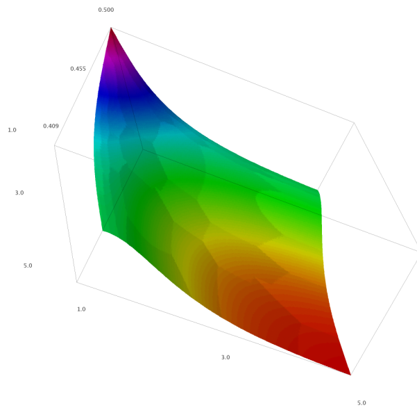
Figure 2.2: Zoom on the graph of f_2(x, y) for 1 \leq x, y \leq 5
