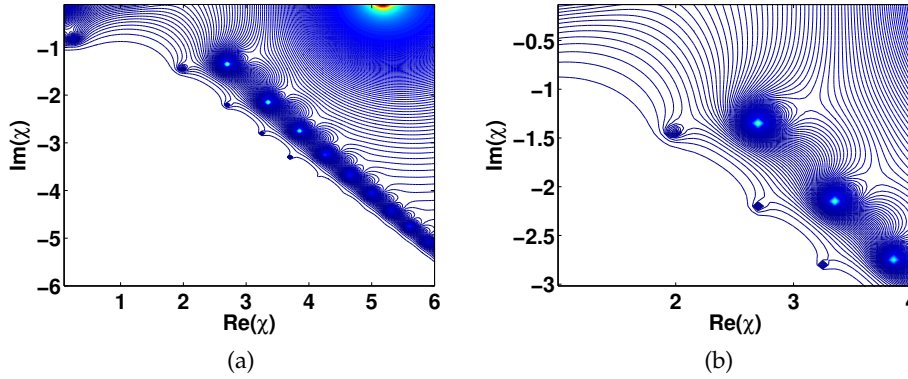
Figure 3.3: (3.3a) Contour plot of |\mathcal{D}|^{-1}(\chi) showing the two branches of isolated poles for \Im(\chi) < 0 . (3.3b) Magnified view showing the lowest frequency damped modes.
