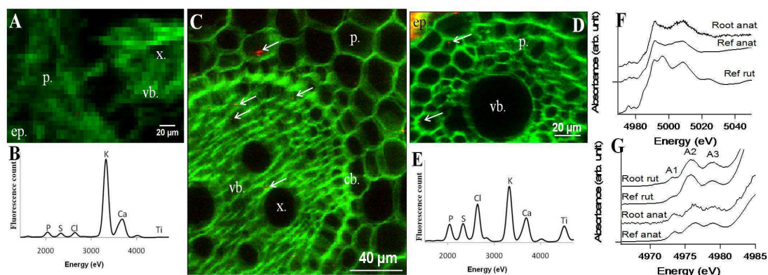
Figure 3. SR- \mu XRF analysis of TiO 2 -NP uptake in plant roots. Roots were grown in water (A-B) or exposed to 100 mg/L anatase TiO 2 -NP suspensions (C-E). Cross sections were analyzed by SR- \mu XRF (B, E: fluorescence spectra; A, C, D: fluorescence maps of K (green) and Ti (red), Ti hot spots are identified by arrows). Image A was acquired on LUCIA beamline (resolution: 5 \mu m 2 ); B and C were acquired on ID21 beamline (resolution: 1 \mu m 2 ). XAS spectra of Ti-enriched zones: whole spectra (F) and enlargement on the pre-edge feature (G) recorded on reference anatase and rutile nanopowders (Ref anat and Ref rut), or on root cross-sections of plants exposed to anatase or rutile NPs (Root anat and Root rut).
