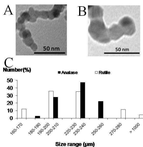
Figure 2. Characterization of TiO 2 -NPs. TiO 2 -NP size and shape were deduced from transmission electron microscope images of anatase (A) and rutile (B) TiO 2 -NPs. Agglomeration state (C) was evaluated after 30 min of pulsed sonication on 100 mg/L TiO 2 -NP suspension in water.
