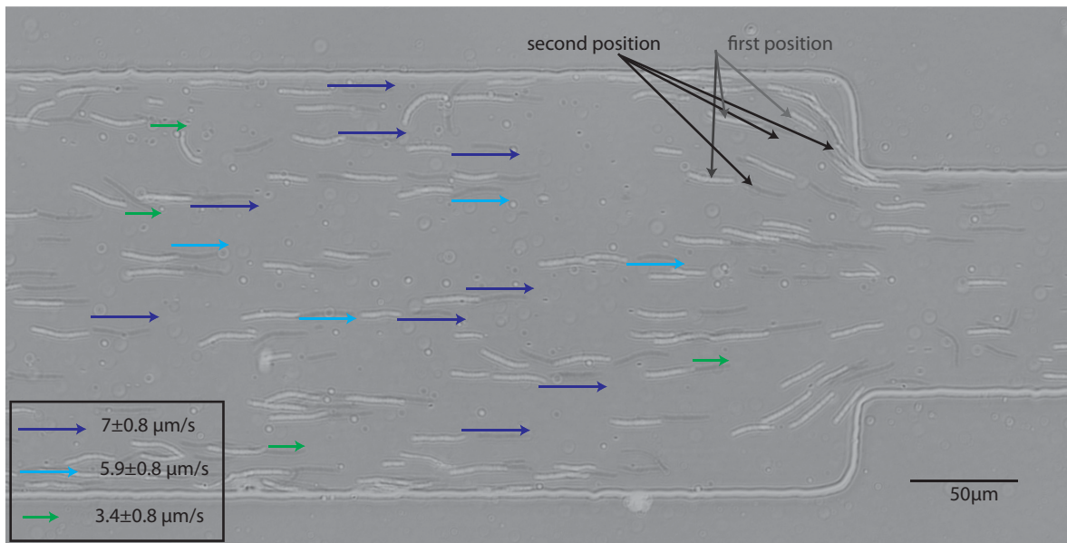
Figure 7.23: Small variations of fiber velocity in the dilute regime. The variations are due to different vertical positions of particles within the Poiseuille velocity profile.
