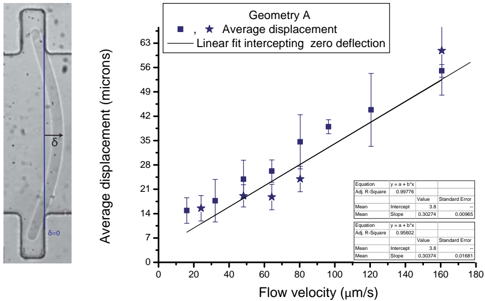
Figure 4.3: Results of fiber deflection reported versus mean flow velocity. Two sets of data points (square and stars) correspond to two different experiments done with the same fiber geometry. They are both linearly fitted with a curve going through the zero deflection point. We find a slope of 0.3 with a 0.3% difference between the two experiments. A picture of a bending fiber is shown left of the graph illustrating how we obtain the deflection data and where the zero is taken.
