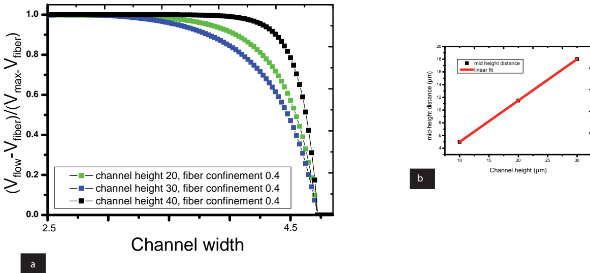
Figure 5.20: Comparison of the velocity profiles for different channel heights, keeping the fiber confinement constant (parallel fiber). a: dimensionless flow profiles along the channel width. b: mid-height distance of flow profiles versus the channel height. The flow perturbation caused by the fiber scales well with the channel height.
