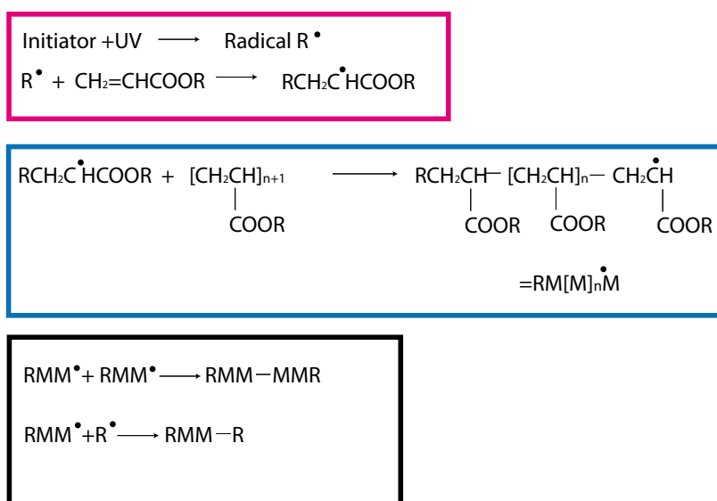
Figure 1.13: radical photopolymerization reaction
