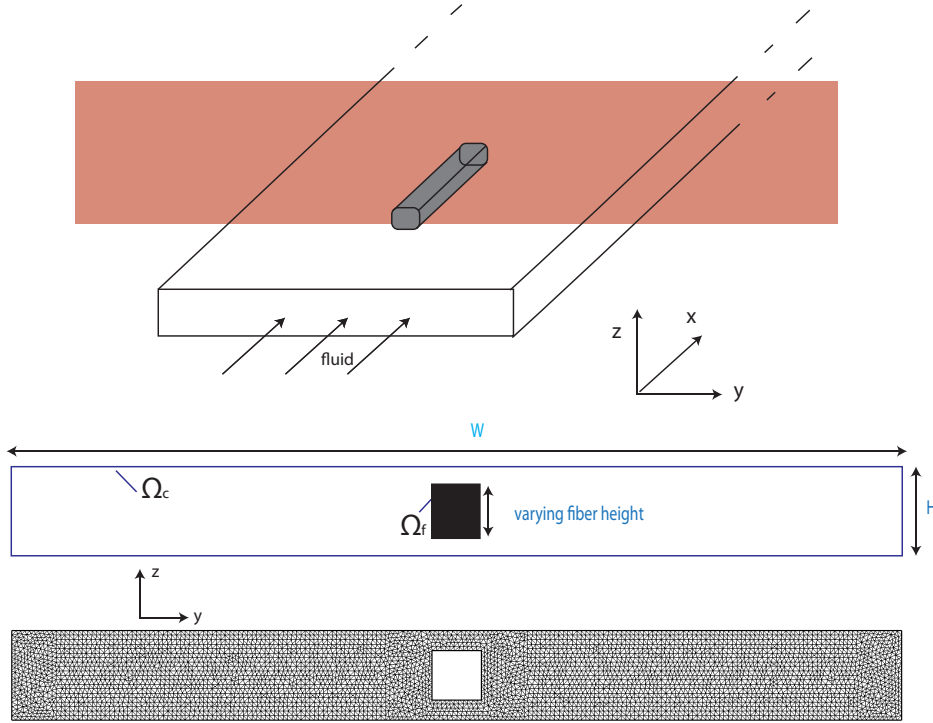
Figure 5.8: Simulations in Oyz plane
