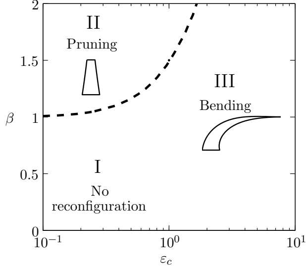
Figure 3.7: Reconfiguration strategy sketched as a function of the two parameters describing the material behavior and the geometry, \varepsilon_c and \beta . The dashed line represents the threshold value \varepsilon_c^{\text{prun}}(\beta) after which only bending occurs.
