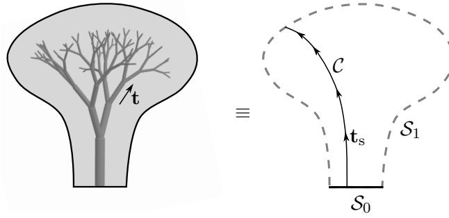
Figure 4.4: Sketch of a characteristic curve used for solving the homogenized problem.
