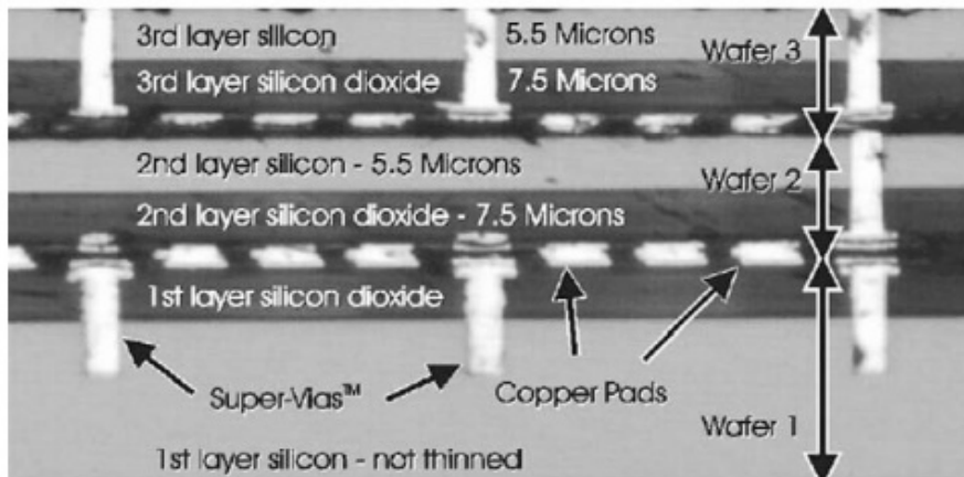
Figure 8.12. Tezzaron metal bonding[62]
