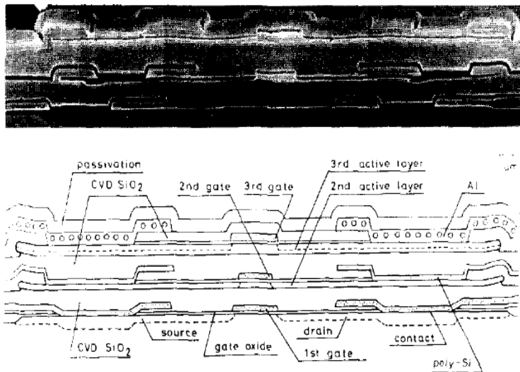
Figure 3.3. Example of 3D Design [42]
