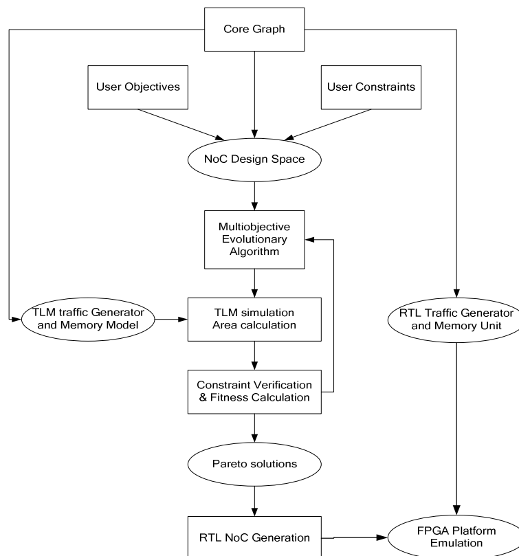
Figure 4.2. 2D NoC synthesis workflow
