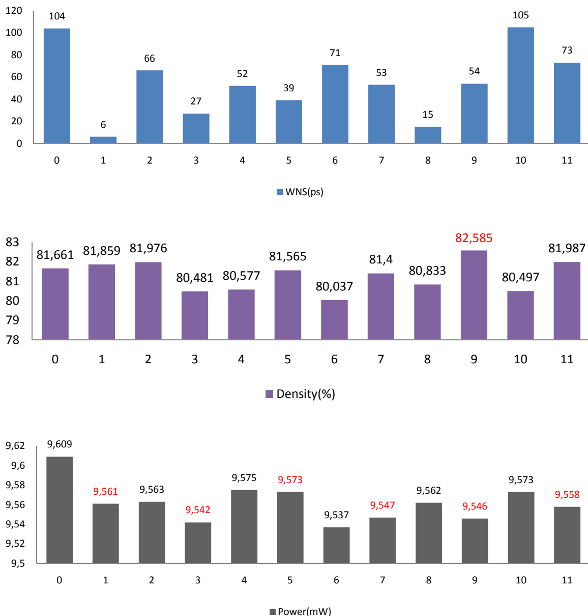
Figure 7.5.. WNS (ps), Density (%) and power (mw) for the different combinations of the DSE (Freq=100MHZ)
