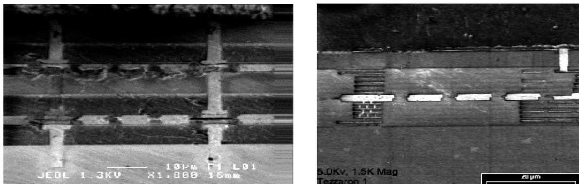
Figure 8.10. Tezzaron 3D Techniques: Super-Via(left), Super Contact(right)[107]
