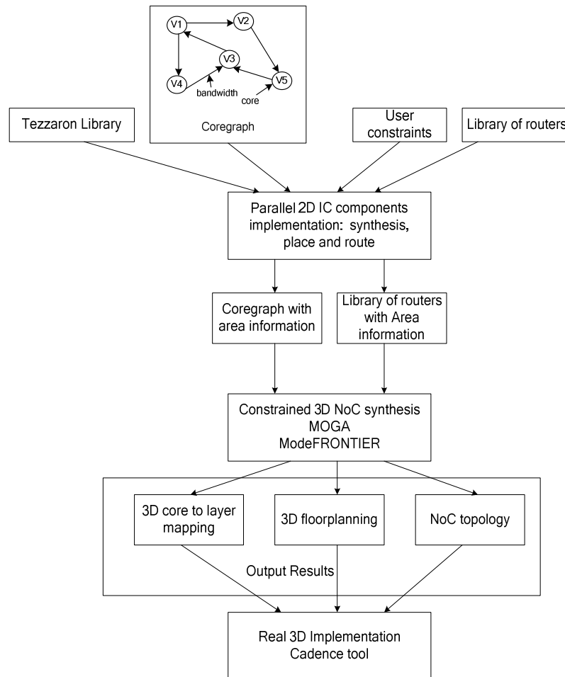
Figure 5.15. Our 3D NoC synthesis workflow
