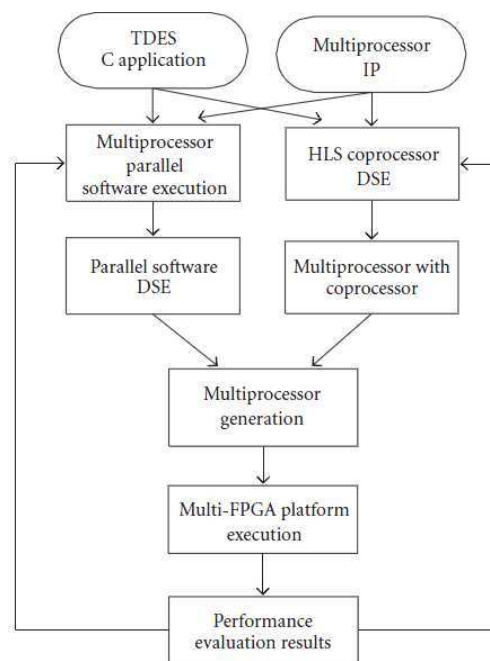
Figure 1.13. Automatic heterogeneous design flow [25]
