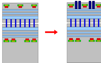
Figure 8.15. Etching for power/Gnd TSV [108]
