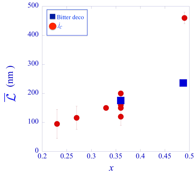
Figure 7.11 Average distance \bar{L} between effective pins versus the P doping level, at T = 5 K (•), and as determined from Bitter decoration (■).
