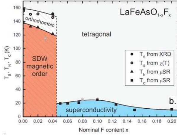
Figure 3.2 Phase diagram of \text{LaFeAsO}_{1-x}\text{F}_x from Ref. [95].
