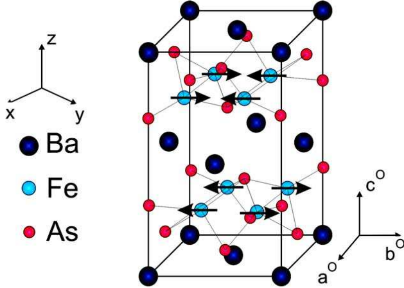
Figure 3.6 SDW order configuration in the parent compound \text{BaFe}_2\text{As}_2 : the spin of Fe atoms are represented by arrows.
