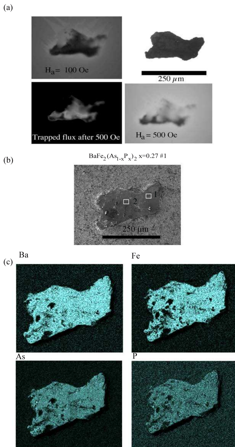
Figure 7.3 (a) DMO images of the crystal that reveal the spatial heterogeneity. (b) SEM image of the crystal with x=0.27 \text{ \#1} . Regions selected for chemical analysis are indicated with squares on the crystal image.(c) Maps of chemical analysis for each element, performed using EDX on the surface of the crystal with x=0.27 \text{ \#1} .
