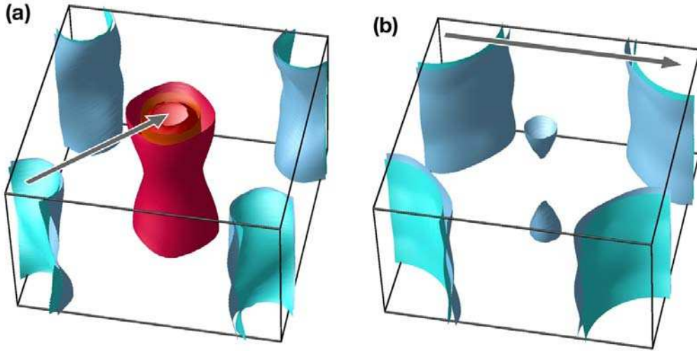
Figure 3.7 (a) Calculated Fermi surfaces for Ba(Fe 1.94 Co 0.06 ) 2 As 2 and (b) K 0.8 Fe 2 Se 2 . Different shades of red denote hole Fermi surfaces, and different shades of blue the electron ones. The arrows show quasineesting vectors. Taken from Ref.[108].
