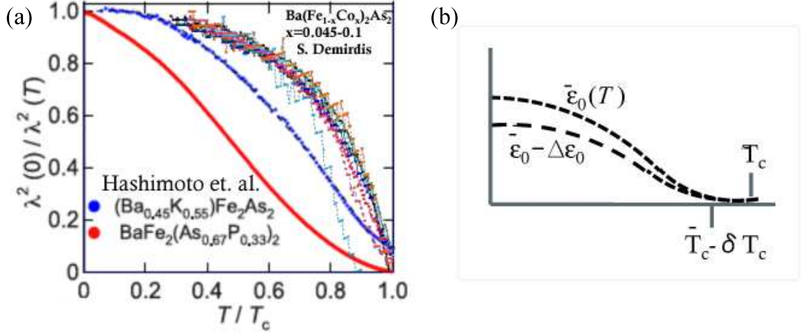
Figure 7.17 (a) Temperature dependence of the superfluid density for \text{BaFe}_2(\text{As}_{1-x}\text{P}_x)_2 and \text{Ba}_{1-x}\text{K}_x\text{Fe}_2\text{As}_2 single crystals from Ref. [135] and \text{Ba}(\text{Fe}_{1-x}\text{Co}_x)_2\text{As}_2 single crystals (see Chapter 8). (b) Sketch of the temperature dependence of mean vortex line energy when approaching T_c .
