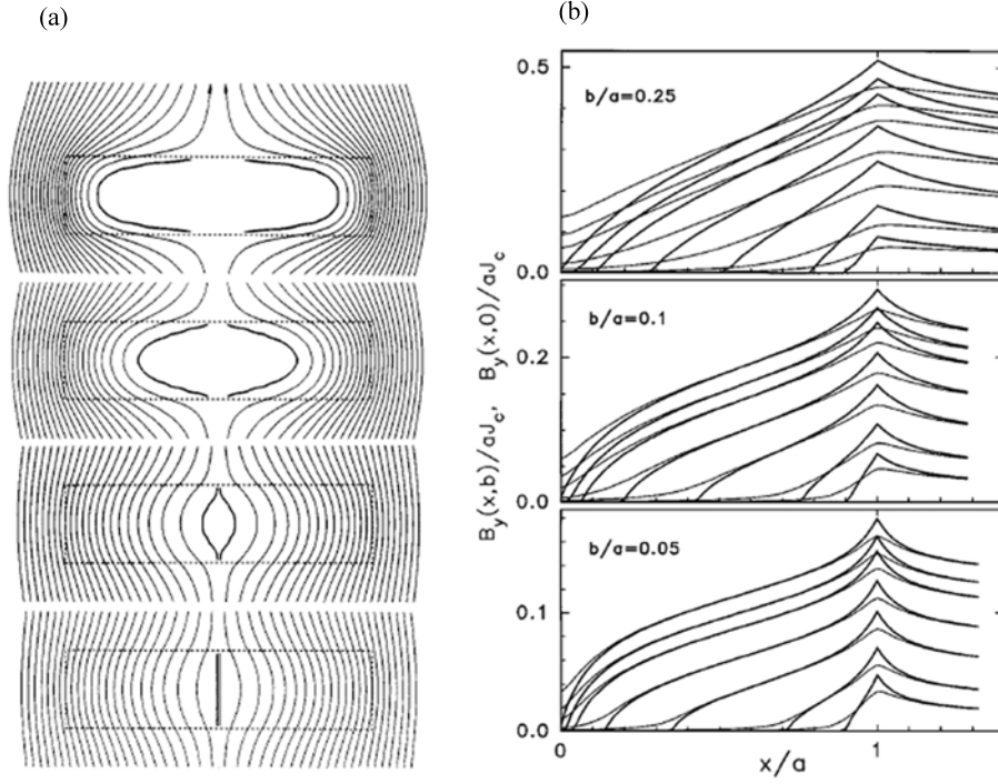
Figure 4.8 (a) Magnetic flux lines during penetration of perpendicular flux into a strip with b/a = 0.25 at applied fields H_a/H_p = 0.2, 0.4, 0.8, \text{ and } 1 . Here, H_p = 0.374 j_{ca} . (b) Profiles of the perpendicular flux density B_y(x, y) at the surface (thin lines, y = \pm b ) and equatorial plane (thick lines, y = 0 ) of bars with side ratio b/a = 0.25, 0.1, 0.05 at applied fields H_a/H_p = 0.1, 0.2, 0.4, 0.6, 0.8, 0.9, \text{ and } 1 . Here for the field at the central plane one has B_x(x, 0) = 0 because of the symmetry. The central field profile for all aspect ratios b/a exhibits a sharp cusp at the sample edges and a sharp flux front inside which B is zero. These features are smeared out into the surface field, but for very thin strips this smearing is weak both fields profiles in the center and at the surface nearly collapse into one curve. From Ref. [62]
