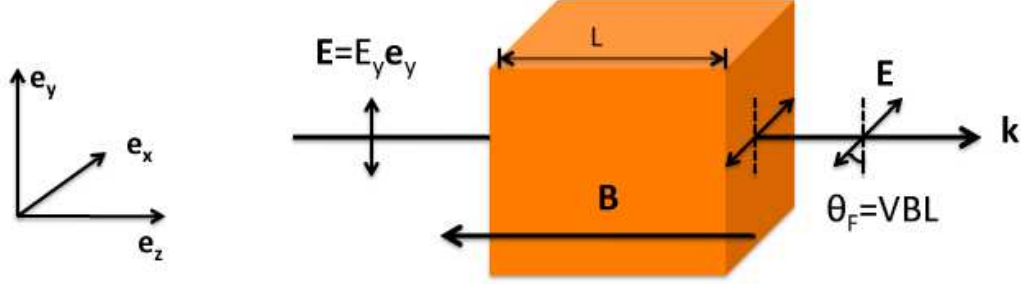
Figure 4.1 Illustration of the Faraday effect: a linearly polarized incident light traverses the medium (from the left to right) in the presence of an axial magnetic field \mathbf{B} (along the z-axis). k denotes the wave vector of the light. Over the path spanning the medium, the direction of the electric field vector \mathbf{E} is rotated over an angle \theta_F = VBL . This effect was discovered by M. Faraday in 1848.
