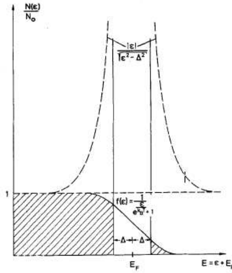
Figure 8.1 The normalized density of states N(\varepsilon) of a superconductor versus the energy \varepsilon referred to the Fermi energy E_F ( \varepsilon = E - E_F ), \Delta = \Delta(T) is the gap parameter. [119]
