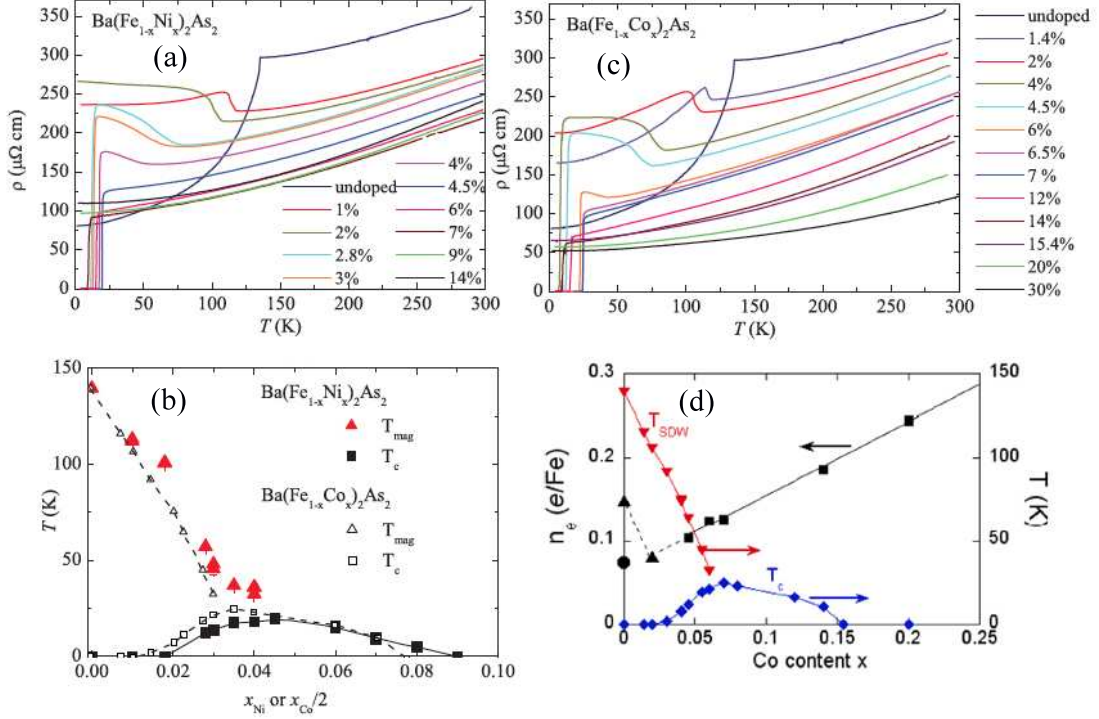
Figure 3.14 (a) Temperature dependence of the resistivity, and (b) Phase diagram indicating T_{\text{mag}} and T_c for both \text{Ba}(\text{Fe}_{1-x}\text{Ni}_x)_2\text{As}_2 and \text{Ba}(\text{Fe}_{1-x}\text{Co}_x)_2\text{As}_2 single crystals. In order to allow a comparison between the two families, the Co content was divided by 2. Lines are guides for the eye from Ref. [11]. (c) Resistivity as a function of temperature and (d) phase diagram for \text{Ba}(\text{Fe}_{1-x}\text{Co}_x)_2\text{As}_2 single crystals (from Ref. [77]).
