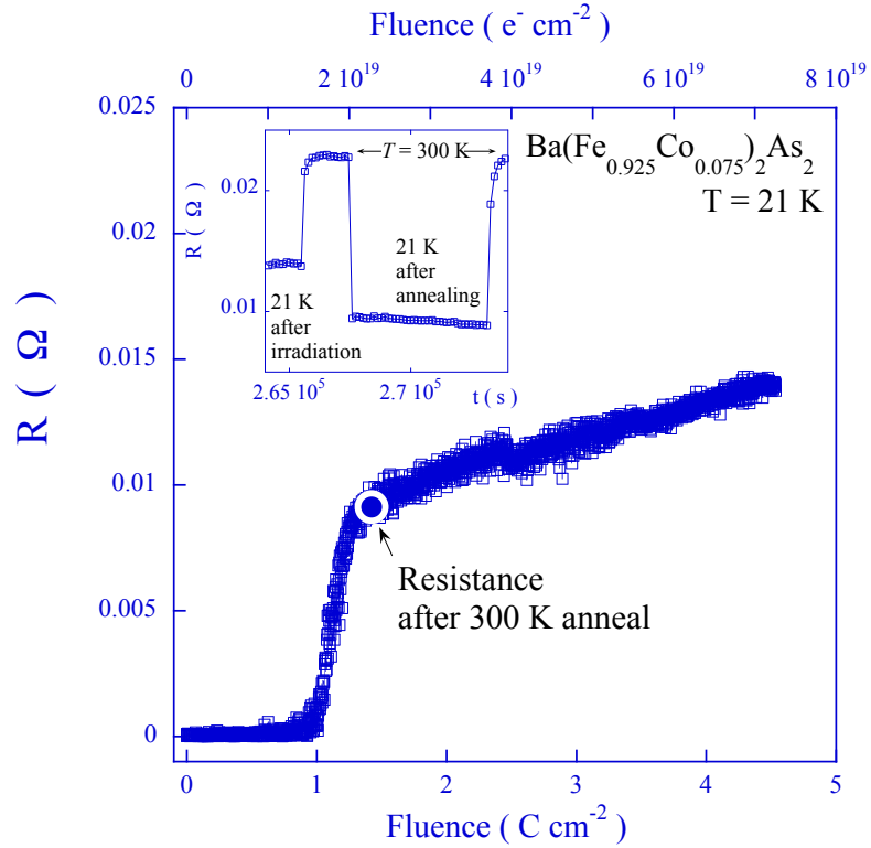
Figure 9.4 \text{Ba}(\text{Fe}_{0.925}\text{Co}_{0.075})_2\text{As}_2 : Resistance as function of dose of 2.5 MeV electrons, measured at 21 K. The sample transits to the normal state after a dose of 1.2 \text{ C cm}^{-2} , after which the resistance increases at a rate of \Delta R/R = 0.14[\text{C cm}^{-2}]^{-1} . The Inset shows the effect of annealing. The resistance of the crystal is represented as function of time. The protocol comprises initial measurements at 21 K following irradiation with 4.6 \text{ C cm}^{-2} 2.5 MeV electrons. The crystal is then warmed to 300 K, cooled to 21 K, and heated once again to 300 K. After the first anneal at 300 K, the resistance drops back to the value reached after low-temperature irradiation with only 1.4 \text{ C cm}^{-2} (white circle on the curve in the main panel).
