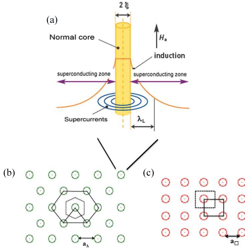
Figure 2.10 (a) Schematic representation of a vortex. The superconducting order parameter vanishes in the core of the vortex which is in the normal state, through where the magnetic field penetrate the superconductor and decreases exponentially over a distance of \lambda_L . (b) The hexagonal perfect lattice configuration of vortices with lattice parameter a_\Delta = 1.075 (\Phi_0/B)^{1/2} , (c) square lattice configuration of vortices with lattice parameter a_\square = (\Phi_0/B)^{1/2}
