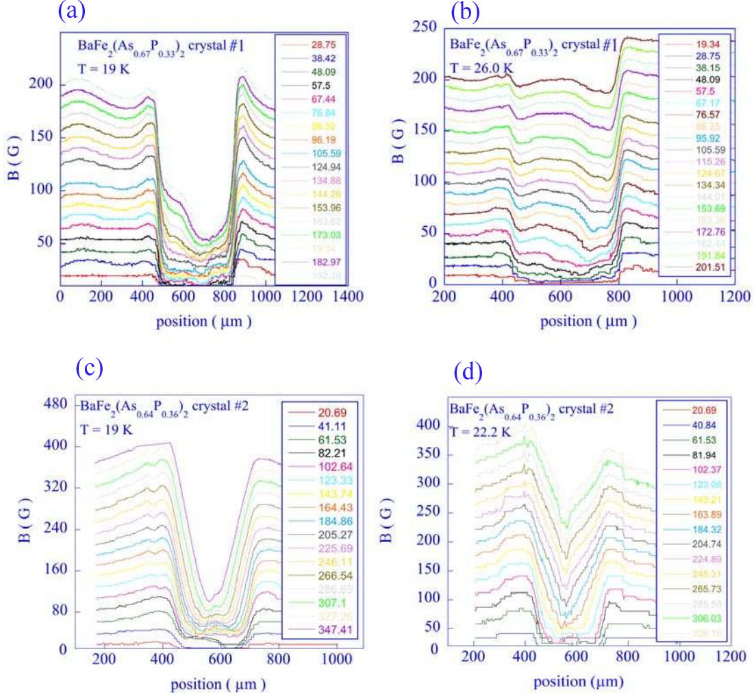
Figure 7.6 Magnetic flux profiles in \text{BaFe}_2(\text{As}_{1-x}\text{P}_x)_2 single crystals ( x = 0.33 #1) at T = 19 K and 26 K (a,b), and ( x = 0.36 #2) at T = 19 K and 22.2 K (c,d). The Bean-like profiles in (c,d) are obtained from the MOI images of Figure 7.5 (b). The profiles presented in (a,b) are influenced by a surface barrier and are obtained from images on the crystal in Fig. 7.5 (a).
