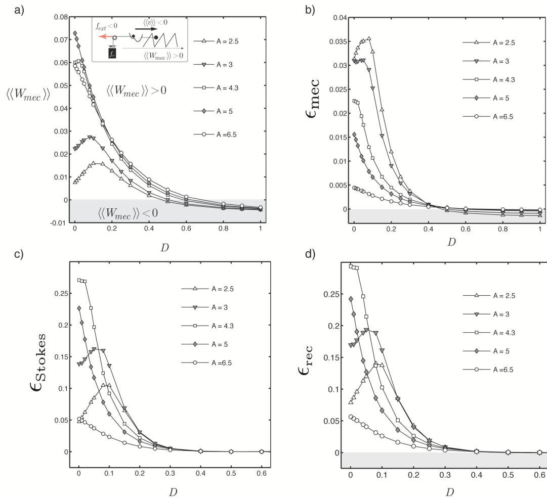
Figure 6.10. The X-tilted model in soft device configuration with the conservative load f_{ext} = -0.1 . a) The variation of the mechanical work W_{mec} with the increasing temperature D for different amplitudes A . b) The variation of the mechanical efficiency \epsilon_{mec} with the increasing temperature D for different amplitudes A . In the regime of small amplitude A we observe a maximum of efficiency at finite temperature. c) The variation of the Stokes efficiency with the increasing temperature D . By definition, this is always positive function. For high values of D the Stokes efficiency is increasing function of D , because we are in regime there the motor follows the direction imposed by cargo. d) The variation of the rectifying efficiency with the increasing temperature D . The shape of this function is dominated by the quadratic Stokes term. The relevant parameters k_0 = 1.5 , k_1 = 0.43 , l = 0.22 , a = 1 , L = 1 , \lambda_1 = 0.7 , V_{max} = 1.5 , \alpha = 1 with time period T = 30 of the rocking force.
