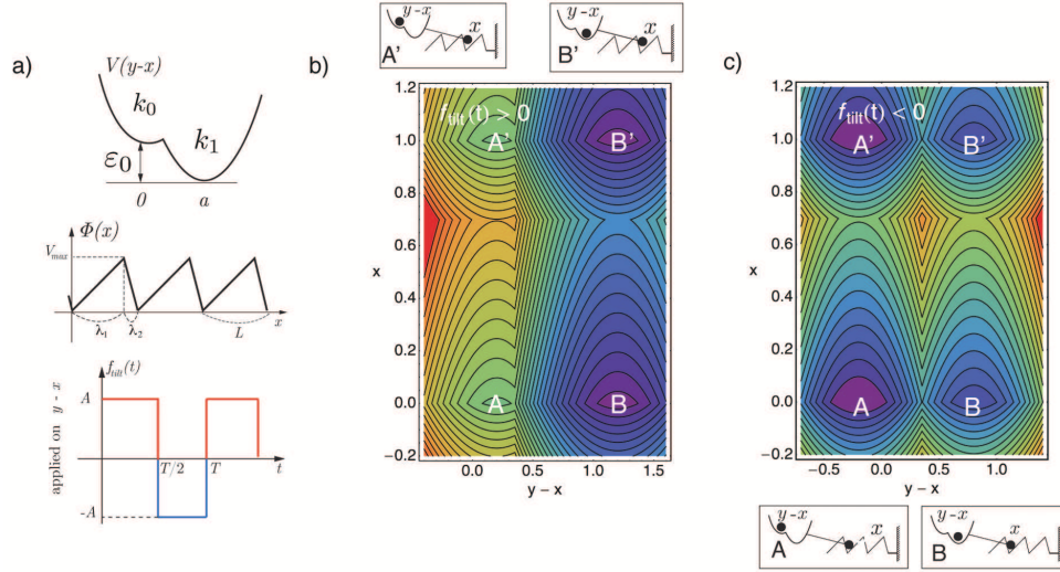
Figure 8.2. The XY-tilted ratchet. a) The sketch of potentials used in numeric applications. b) The picture illustrates the action of f_{\text{tilt}}(t) on two-dimensional energy landscape in plane [y-x, x] . The increasing energy level scale graduated from cold color to hot colors. a) We show unbiased landscape in soft device configuration we identify the occupancy motor state, is intrinsic energy potential. b) The landscape corresponds to positive phase of f_{\text{tilt}}(t) = A . c) The landscape corresponded to the negative phase of f_{\text{tilt}}(t) = -A .
