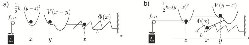
Figure B.1. The sketch of simple 3D soft device, the model of one single cross-bridge adopted as element of collective model used a big number of coupled cross-bridges.
