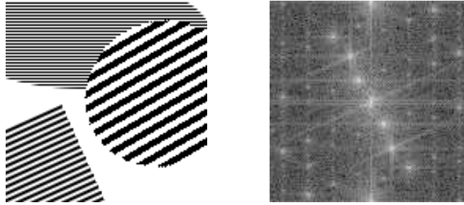
Figure 4.11: Image g_0 and its spectrum \log |\mathcal{F}(g_0)| ,
