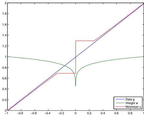
Figure 2.5: Hölder continuous weight w(x) = |x|^{1/10}
