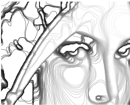
Figure 2.11: Level lines for the TV-minimizer of the Lena image
