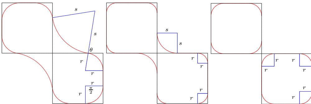
Figure 2.13: F_{r,s} .
