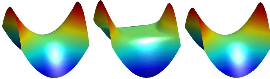
Figure 3.6: Graph of g , the TV -minimizer and the \tilde{J} -minimizer, respectively. One kept \lambda = 100 .
