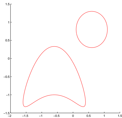
Figure 4.2: Scatterer D .
