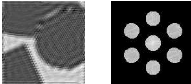
Figure 4.12: Image g and its spectrum \log |\mathcal{F}(g)| .
