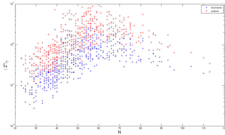
Figure 3.6: g(S_T) = (S_T^1 - K)_+ , K = 120 . "+" and "+" correspond respectively to " \langle Z^n \rangle_{T,\text{uniform}} " and " \langle Z^n \rangle_{T,\text{stochastic}} ".
