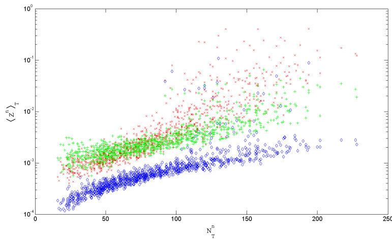
Figure 3.2: "x", "+" and "◇" correspond respectively to " \langle Z^n \rangle_{T,\text{uniform}} ", " \langle Z^n \rangle_{T,\text{fractional}} " and " \langle Z^n \rangle_{T,\text{stochastic}} ".
