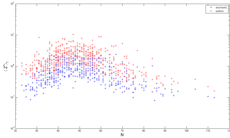
Figure 3.5: g(S_T) = (S_T^1 - K)_+ , K = 100 . "+" and "+" correspond respectively to " \langle Z^n \rangle_{T,\text{uniform}} " and " \langle Z^n \rangle_{T,\text{stochastic}} ".
