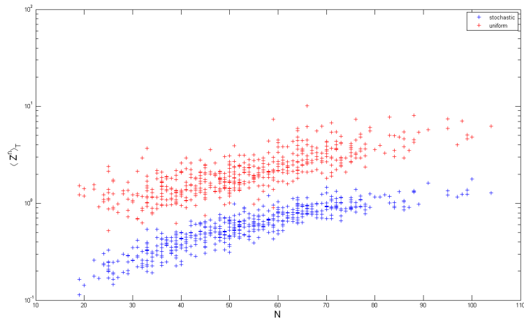
Figure 3.3: g(S_T) = (S_T^1 - S_T^2)_+ , "+" and "+" correspond respectively to " \langle Z^n \rangle_{T,\text{uniform}} " and " \langle Z^n \rangle_{T,\text{stochastic}} ".
