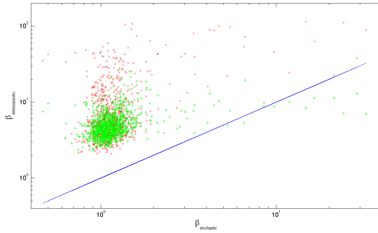
Figure 3.1: "x", "+" and the blue line correspond respectively to " (\beta_{\text{stochastic}}, \beta_{\text{uniform}}) ", " (\beta_{\text{stochastic}}, \beta_{\text{fractional}}) " and the identity function.
