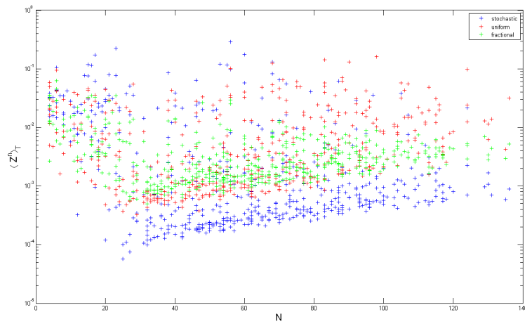
Figure 3.8: g(S_T) = 1_{S_T^1 \geq K} , K = 100 . "+", "+" and "+" correspond respectively to " \langle Z^n \rangle_{T,\text{uniform}} ", " \langle Z^n \rangle_{T,\text{fractional}} " and " \langle Z^n \rangle_{T,\text{stochastic}} ".
