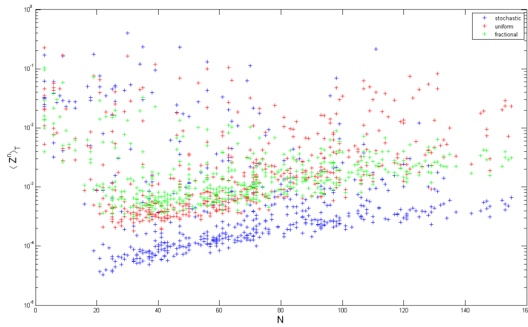
Figure 3.9: g(S_T) = 1_{S_T \geq K} , K = 120 . "+", "+" and "+" correspond respectively to " \langle Z^n \rangle_{T,\text{uniform}} ", " \langle Z^n \rangle_{T,\text{fractional}} " and " \langle Z^n \rangle_{T,\text{stochastic}} ".
