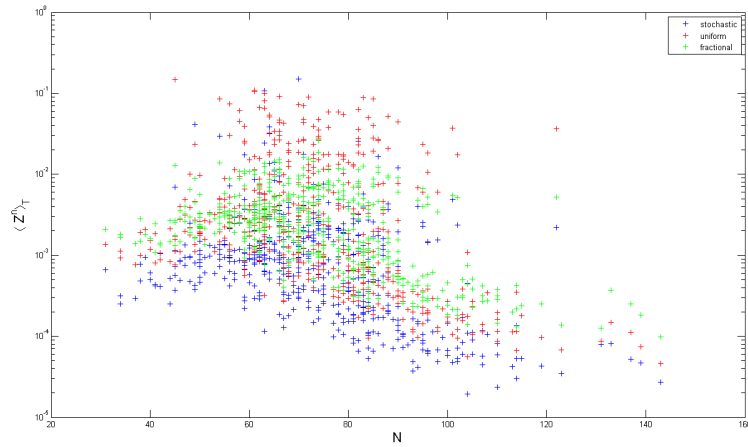
Figure 3.7: g(S_T) = 1_{S_T^1 \geq K} , K = 80 . "+", "+" and "+" correspond respectively to " \langle Z^n \rangle_{T,\text{uniform}} ", " \langle Z^n \rangle_{T,\text{fractional}} " and " \langle Z^n \rangle_{T,\text{stochastic}} ".
