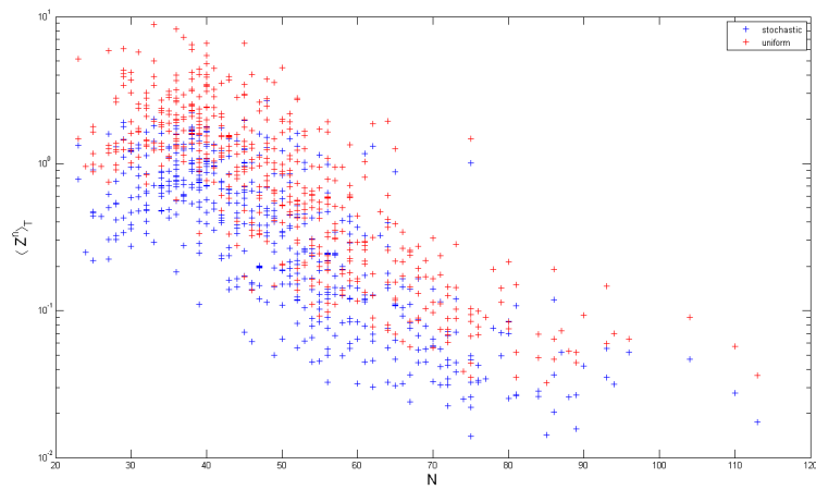
Figure 3.4: g(S_T) = (S_T^1 - K)_+ , K = 80 . "+" and "+" correspond respectively to " \langle Z^n \rangle_{T,\text{uniform}} " and " \langle Z^n \rangle_{T,\text{stochastic}} ".
