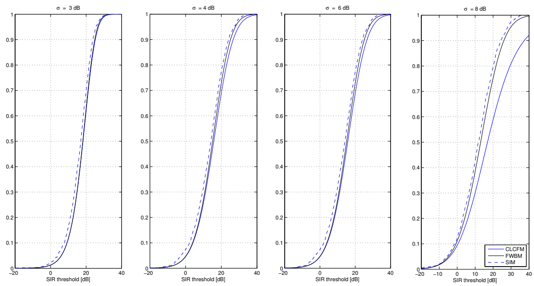
Figure 4.1: Influence of the shadowing standard deviation \sigma [dB] with r = 0.2 Km and \eta = 3.0 .
