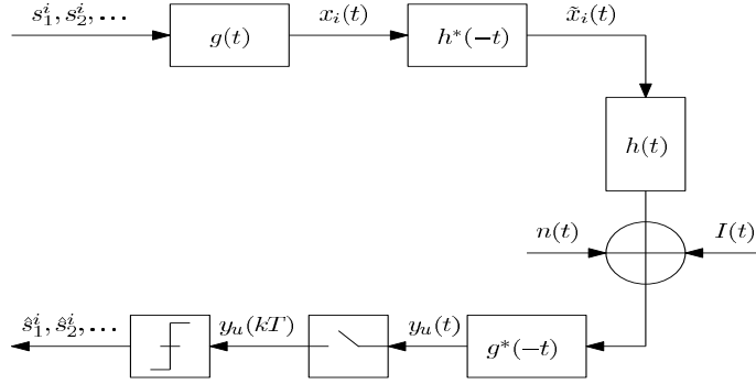
Figure 5.1: Transmission scheme.
