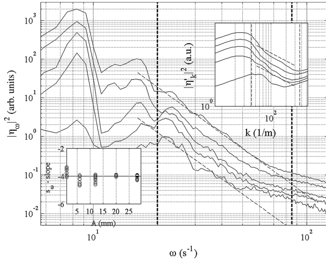
FIG. 5. Experiments II: Spectra |\eta_\omega|^2 . Same representation as in Fig. 3 (only the gravity regime is accessible in these experiments).
