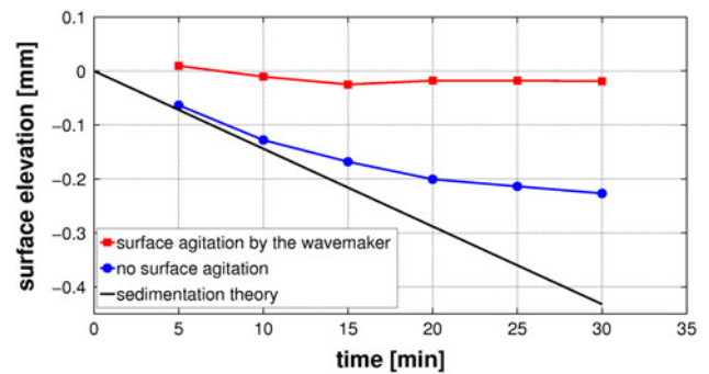
Fig. 4 The apparent surface position, as measured by FTP, as a function of time for two cases: no liquid shaking ( blue curve ), the liquid was excited by waves produced by a wavemaker during a short time between two measurements ( red curve ). Black curve shows the theoretical prediction for the sedimentation (Eq. 2, using the mean size of the particles). The dispersion used here is the anatase with a concentration of 4 g/l. The real position of the free surface is at zero (the errorbar is 0.02 mm)
