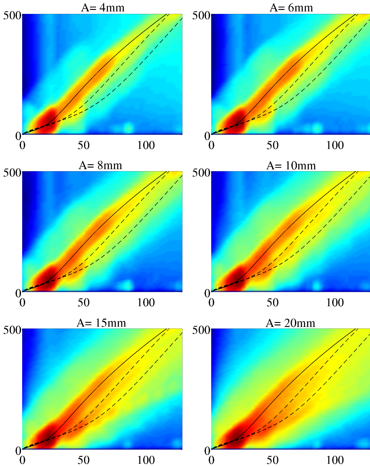
Figure 4.4: Spectra |\eta_{k,\omega}|^2 for narrowband forcing for different forcing amplitudes A . Solid line shows the linear dispersion relation and the dashed lines the dispersion relation for slave modes (2,3). Horizontal axis show frequency \omega (rad/s) and vertical axis - wavenumber k (1/m).
