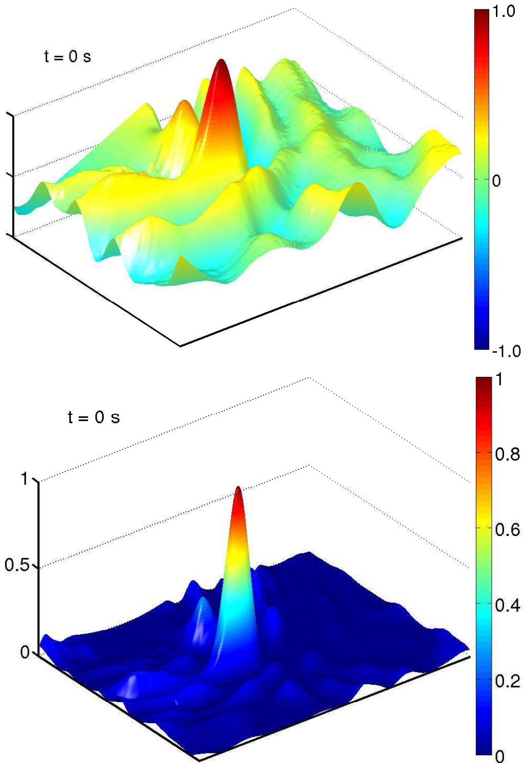
FIG. 3. (Color online). Measured amplitude ( \eta(\mathbf{r}, t = 0) ) and intensity ( (\eta(\mathbf{r}, t = 0))^2 ) of the time reversed wave around the initial source position (point A) where the wave is refocused at the recompression time ( t = 0 ) in a one channel TR experiment ( N = 1 ). The spatial range around the refocusing point A is 34 \times 26 \text{ cm}^2 .
