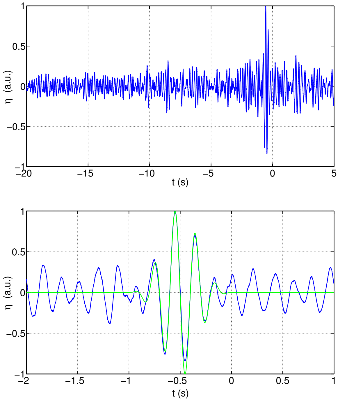
Figure 3.4: Blue line: Surface elevation measurement during the time reversed step in the source position (top) and its close-up around the recompression time t = 0 s (bottom). Green line indicates an excitation function used in the first step of the experiment. The undone time evolution of the reversed signal is similar to the excitation function.
