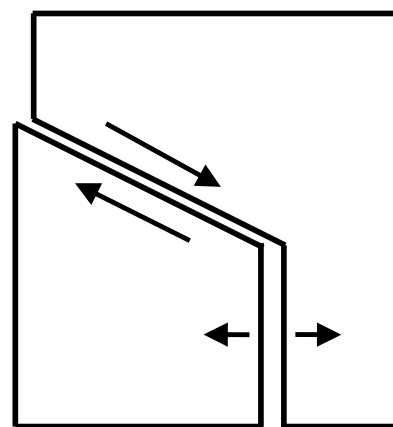
Tensile cracks at the tip of shear band
