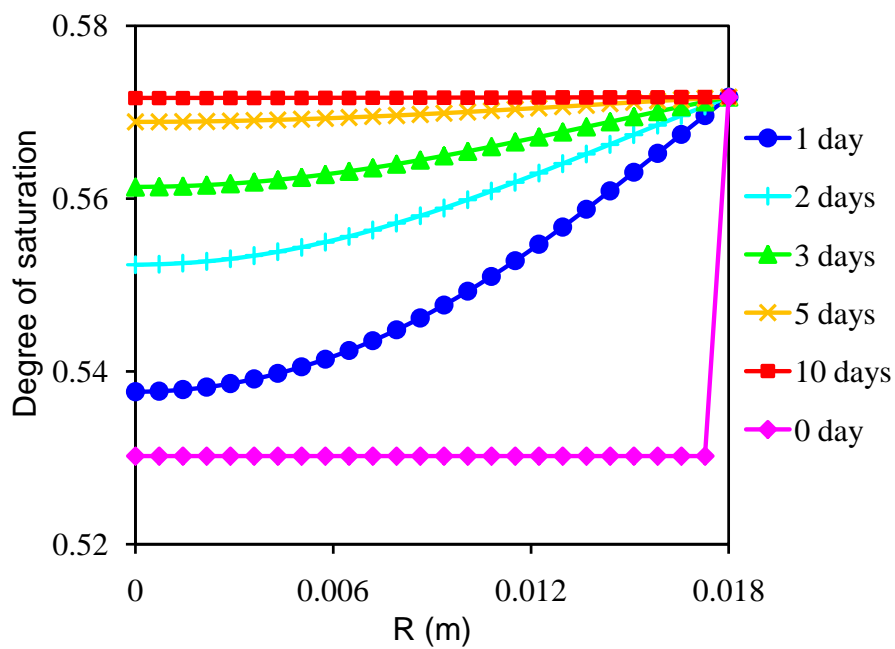
Figure A.4: Saturation profiles within the specimen at different times.
