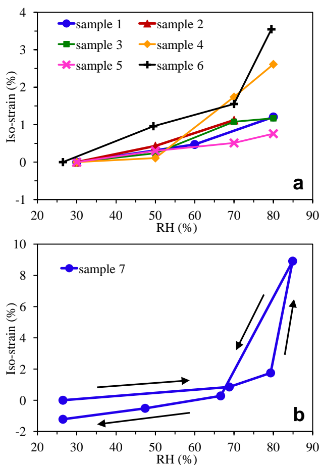
Figure B.4: Steady-state iso-strains measured during monotonic swelling (a) and swelling-drying cycle (b).
