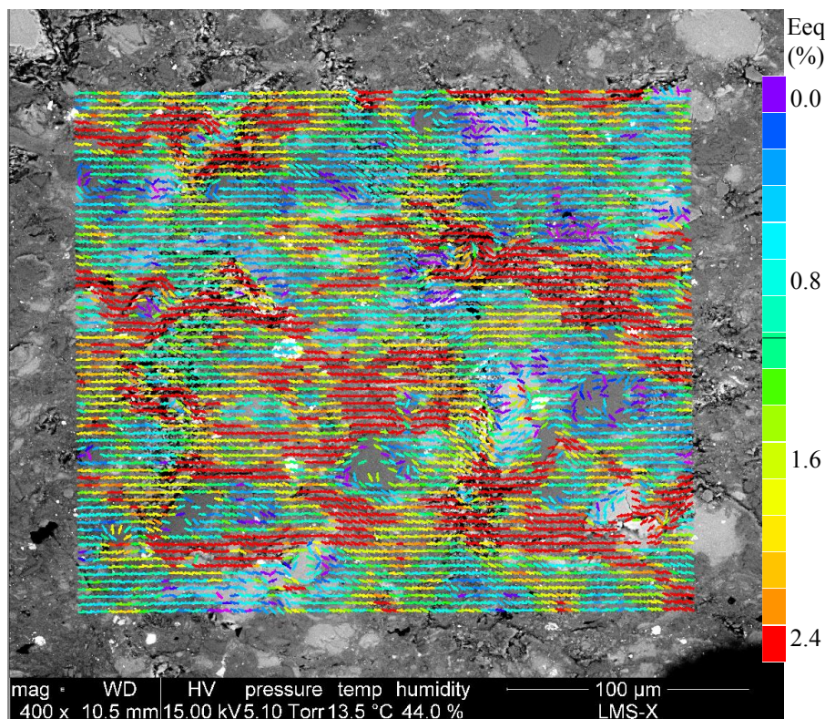
Figure 4.24: Strain field of zone 3 in test #3 (17.4 MPa).
