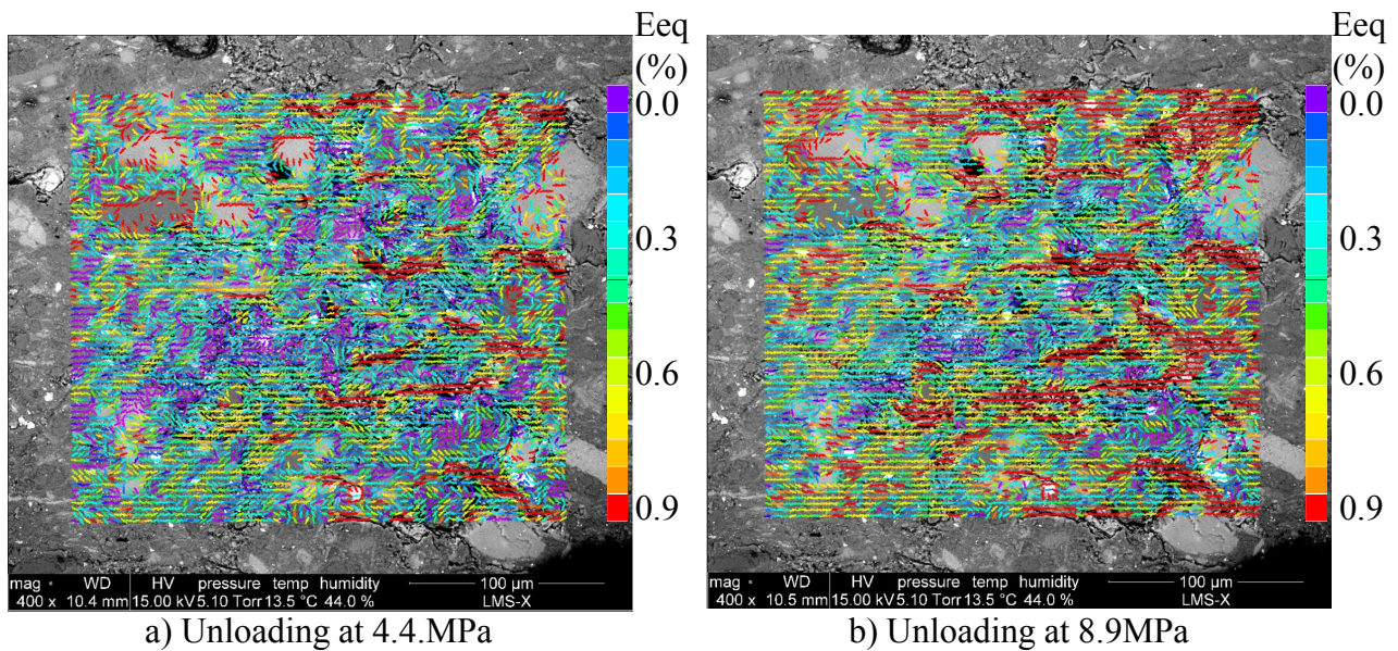
Figure 4.28: Plastic equivalent deformations evolution in zone 1.
