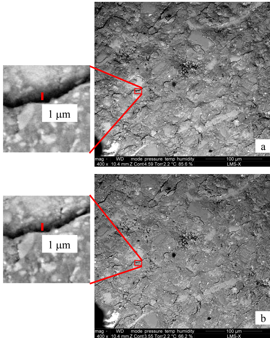
Figure 3.34: Evolution of microcracking due to humidification in test #6: a) 90%RH, b) 66%RH in case of desiccation.
