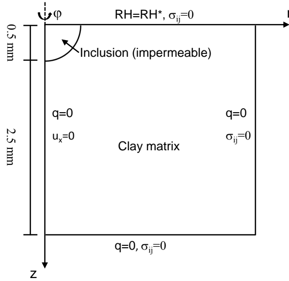
Figure 5.8: Geometry of the specimen and boundary conditions.
