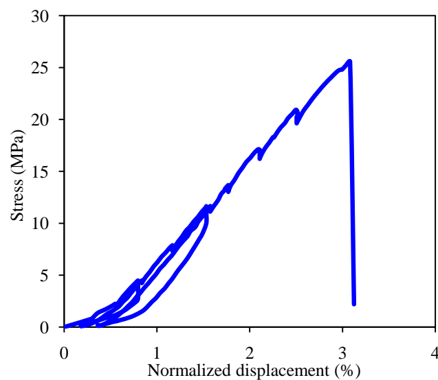
Figure 4.32: Stress vs. normalized displacement (LVDT) in test #4.
