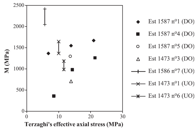
Figure 1.39: Biot's modulus as a function of Terzaghi's effective axial stress (Bemer et al., 2004).
