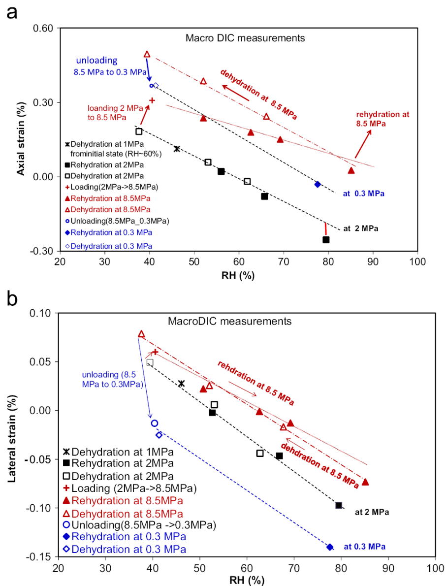
Figure 1.29: (a) axial strain,(b)lateral strain, versus relative humidity at each moisture equilibrium state during three cycles of rehydration and dehydration at the different applied uniaxial stress (2 MPa,8.5 MPa,0.3 MPa) (Yang et al., 2012).
