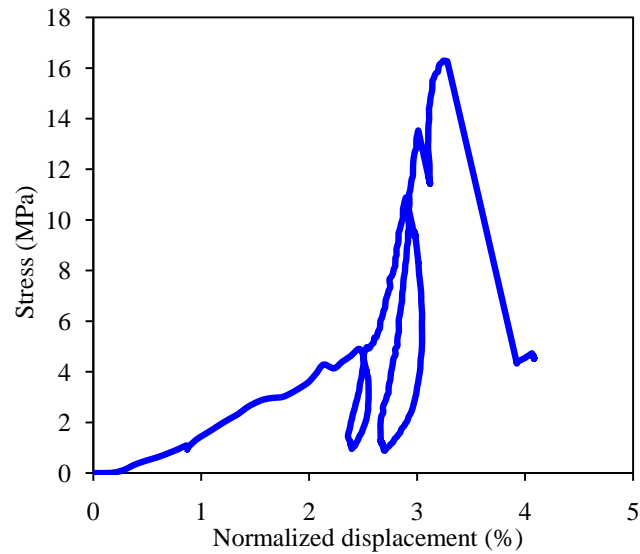
Figure 4.52: Stress vs. normalized displacement (LVDT) in test #6.
