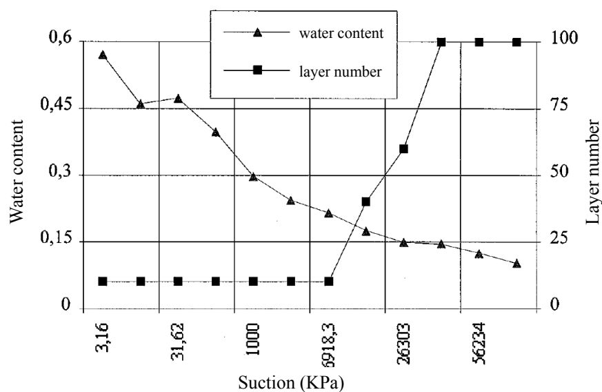
Figure 1.17: Number of layers per particle and water content versus suction (Saiyur et al., 2000).
