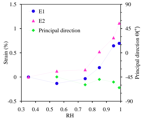
Figure 3.13: Overall strain of zone 2 in test #4.
