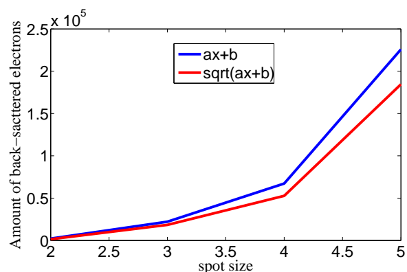
Figure 2.19: Evolution of the amount of electrons received with spot size (SEM units). Image acquisition conditions: BSE mode, 10keV, Dwell time = 30\mu\text{s}/\text{pixel} , Magnification \times 2000 , Pressure = 35Pa.
