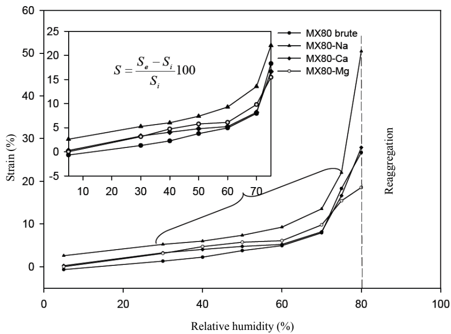
Figure 1.11: Swelling-shrinking of clay aggregate (Montes-H, 2002).
