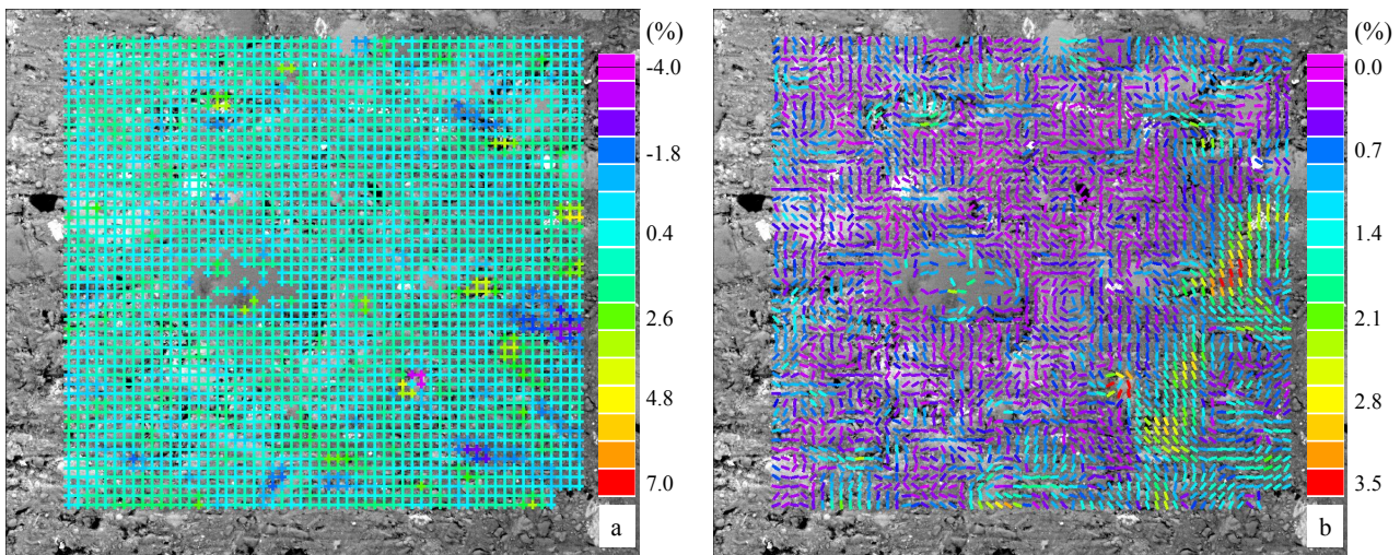
Figure 3.40: Residual deformations at the end of humidification-desiccation cycle (RH=65%) in test #7: a) mean strain, b) equivalent strain.
