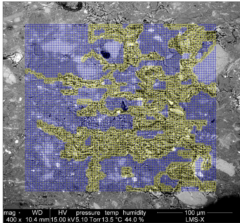
Figure 4.26: Phase definition in zone 1. Yellow color represents macropore-rich domain 1, while blue color represents domain 2.
