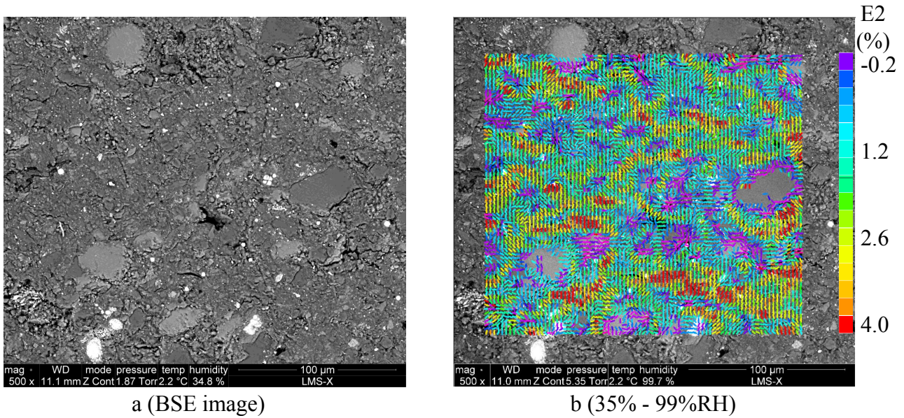
Figure 3.28: BSE image (a) and \varepsilon_2 strain map (b) of zone 3 in test #5.
