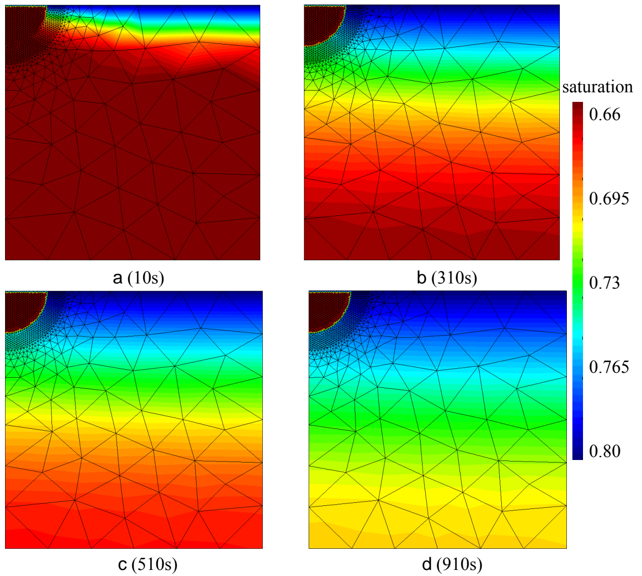
Figure 5.9: Evolution of saturation within the specimen.
