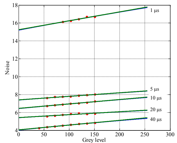
Figure 2.21: Influence of dwell time on ESEM image noise. Image acquisition conditions: BSE mode, 15 keV, Spot size = 5, ESEM (4.05 Torr = 539 Pa), WD = 10.0 mm. Diaphragm = 4.
