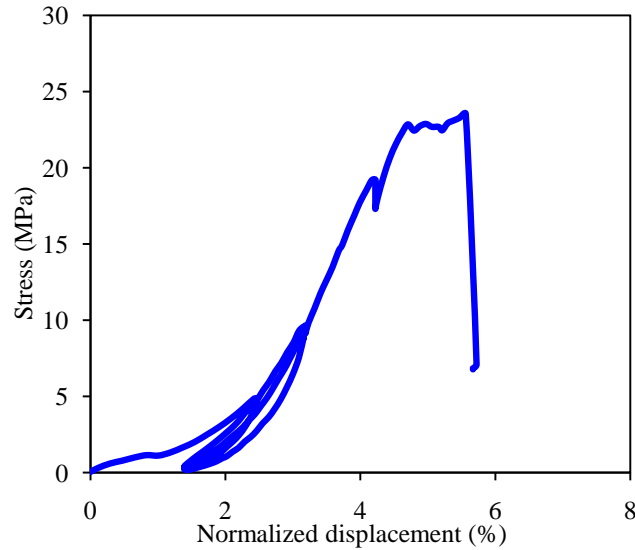
Figure 4.18: Stress vs. normalized displacement (LVDT) in test #3.
