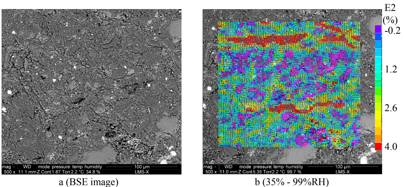
Figure 3.29: BSE image (a) and \varepsilon_2 strain map (b) of zone 4 in test #5.
