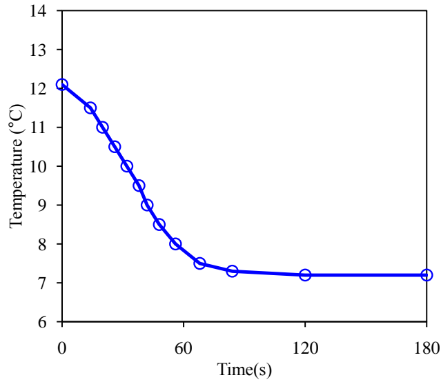
Figure 4.5: Equilibrium time for cooling the sample surface.
