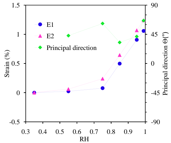
Figure 3.15: Overall strain of zone 4 in test #4.
