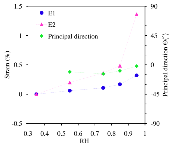
Figure 3.23: Overall strain of zone 2 in test #5.
