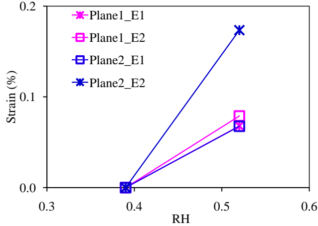
Figure 3.10: Anisotropic deformation of argillaceous rocks under humidification.
