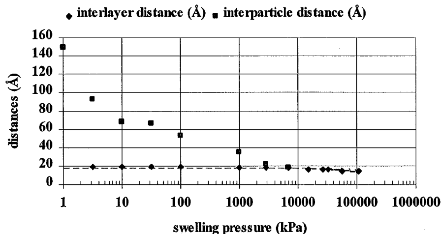
Figure 1.15: Interlayer and inter-particle separation versus suction (Saiyoun et al., 2000).
