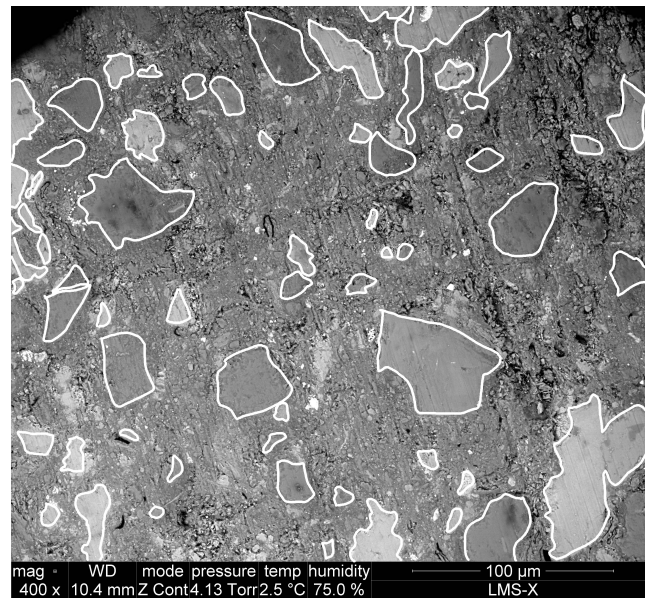
Figure 1.5: Microstructure of argillaceous rocks by ESEM observation: backscattered electron imaging, environmental mode. Argillaceous rocks can be described as a composite structure made of continuous clay matrix scattered by some mineral inclusions (mostly carbonate and quartz). The contours of some big inclusions, appearing in relatively homogeneous grey, are marked in white lines. Besides the three principal components, some pyrites (the brightest domains in the ESEM image) can also be found, as well as some pores principally around big grains or in clay matrix.
