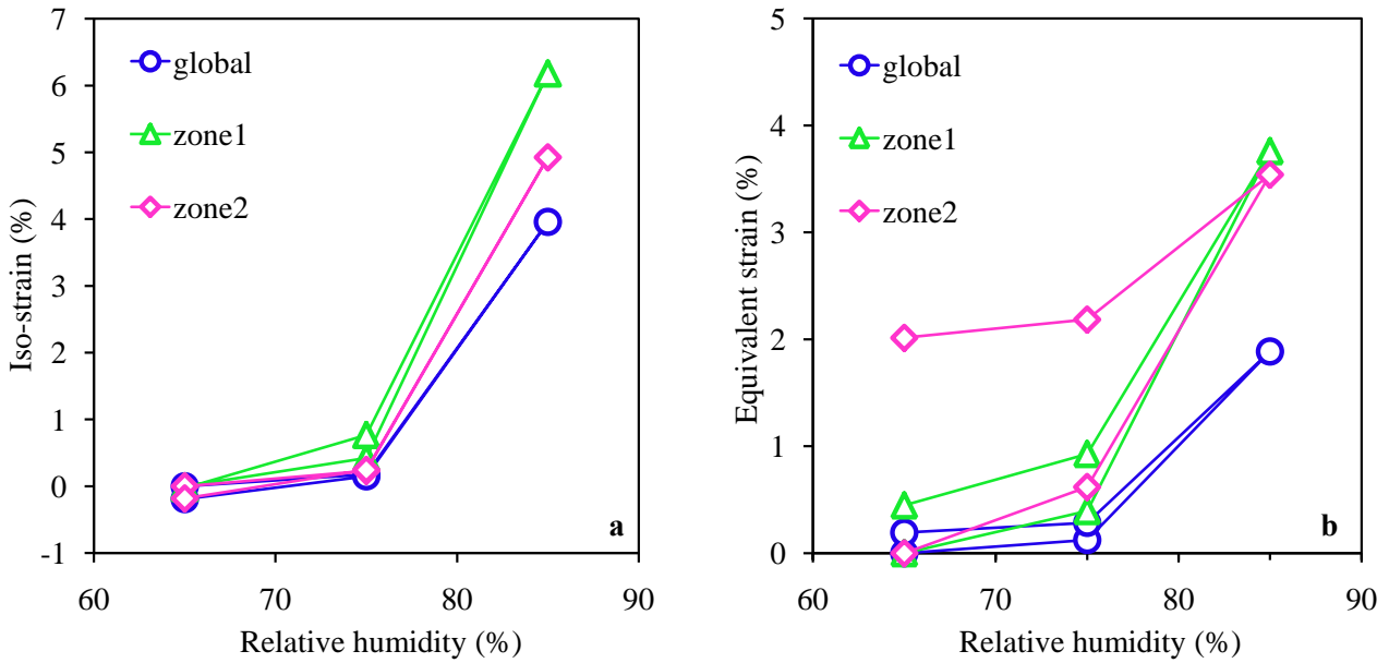
Figure 3.42: Strain curves in different zones in test #7.
