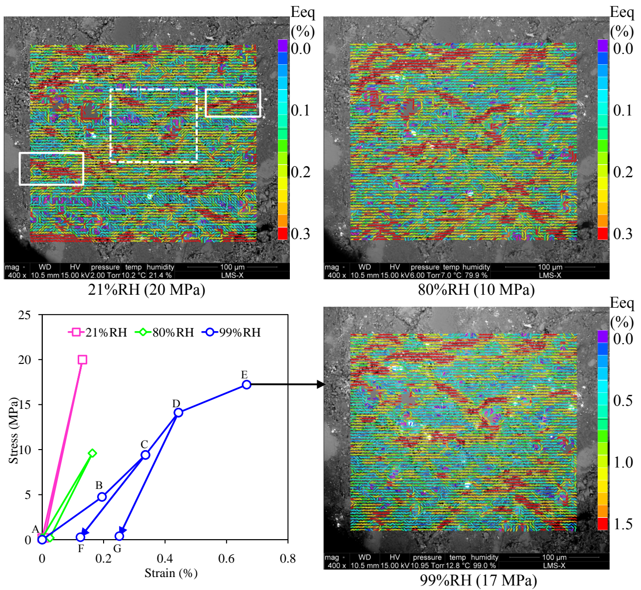
Figure 4.74: Stress-strain curve and strain fields of zone 2 in test #7 measured by DIC. Dashed rectangle would be zoomed on in Fig.4.77.
