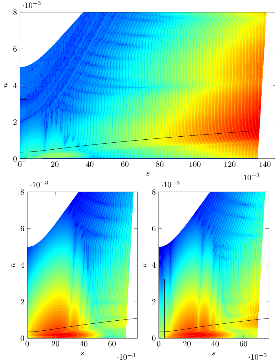
Figure 5.14: Eigenvectors A1 (top), S2 (bottom left) and A2 (bottom right) in the (s, n) -plane, visualized by the \Re(\hat{u}) -velocity component, logarithmic scale. The computational domain used for the S2 and the A2 eigenvectors has a chordwise extent equivalent to approximately half the computational domain used for the S1 and A1 eigenvectors. In all eigenvectors, an attachment-line structure is clearly visible, followed by a transition region and crossflow vortices structures growing exponentially in the s -direction. The peak of the attachment-line structure moves downstream when descending to smaller growth rates.
