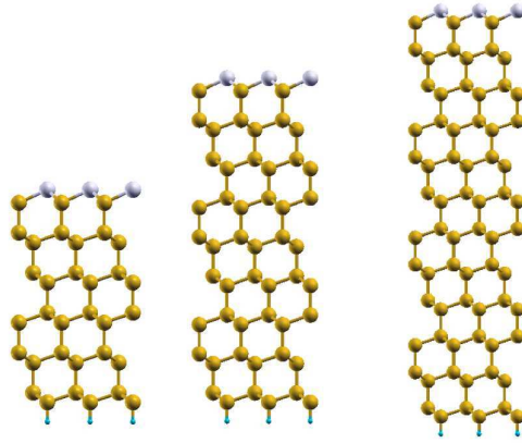
Figure 6.30: H/Si(111)(6dl)/As (left) H/Si(111)(9dl)/As (center) and H/Si(111)(12dl)/As (right) systems. The silicon (yellow) thickness is increased. The bottom surface is terminatd with hydrogen atoms (light-blue) while the upper surface is terminated with As atoms (white).
