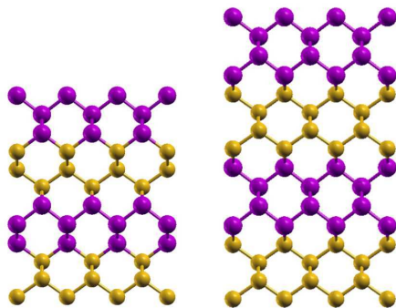
Figure 7.3: Ball and stick representation of the \text{Si}_3/\text{Ge}_3 (left) and \text{Si}_4/\text{Ge}_4 system (right), silicon is represented by yellow-balls and Ge by violet ones.
