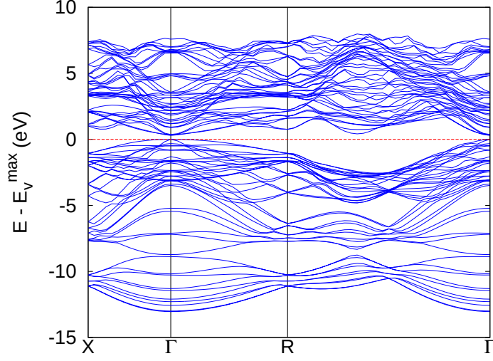
Figure 7.5: Band structure of the Si 5 /Ge 5 superlattice along the X - \Gamma - R - \Gamma path. The zero has been taken as the valence maximum.
