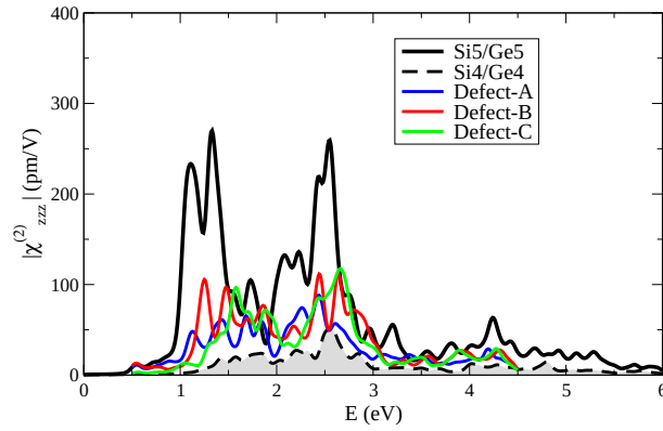
Figure 7.10: Second-harmonics generation spectra ( \chi_{zzz}^{(2)} ) calculated in the independent particle approximation for the substitutional defects of Figs. (7.7-7.9). The \text{Si}_5/\text{Ge}_5 (black continuous line) and the \text{Si}_4/\text{Ge}_4 (black dashed line) systems have been reported for comparison. The defects stay in-between the two perfect systems.
