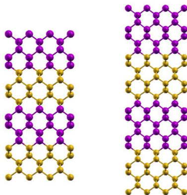
Figure 7.4: Ball and stick representation of the \text{Si}_5/\text{Ge}_5 (left) and \text{Si}_7/\text{Ge}_7 system (right), silicon is represented by yellow-balls and Ge by violet ones.
