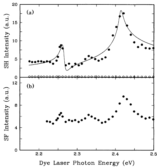
Figure 6.2: Resonant three-wave-mixing signals associated with \chi_{M\ zzz}^{(2)} as a function of the energy of a photon from the tunable dye laser. (a) Results for the SHG process and (b) the SF generation mixing the dye laser output with a photon of fixed energy (1.17 eV). The filled symbols refer to signals from the Si(111)/CaF 2 sample. The open symbols refers to a Si(111) surface covered by native oxide showing the contribution of the underlying Si surface being negligible. The solid curve in (a) is a fit to theory presented in [82] (Reproduced from [82], Copyright ©1989 by The American Physical Society).
