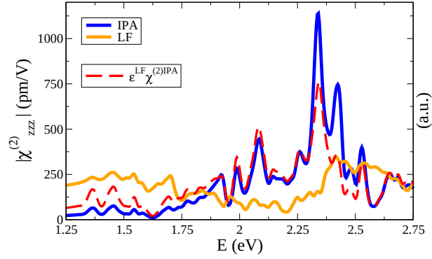
Figure 6.48: Comparison of the SHG ( \chi_{M\ zzz}^{(2)} ) spectra obtained within the IPA (blue line), including LF (orange line), and combining the LF dielectric function \epsilon_{M\ zz} and the IPA- \chi_{\rho\rho\rho}^{(2)} (red dashed line) in Eq. (4.126). The latter curve is reported in arbitrary units (right hand-side scale). The curve recovers with good agreement the IPA spectrum.
