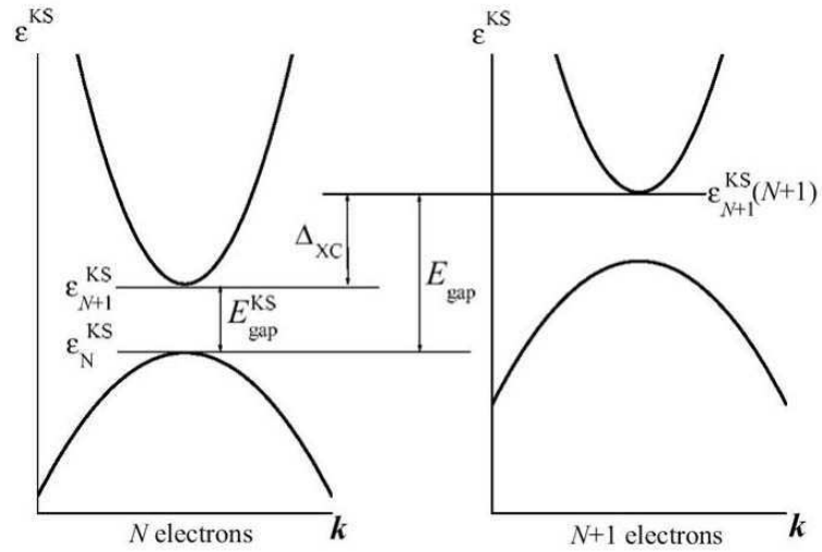
Figure 2.3: On the left: Kohn-Sham band structure (HOMO and LUMO states) of a N particles semiconductor; on the right: Kohn-Sham band structure of the N + 1 particles system. The shift \Delta_{\text{XC}} due to the addition of an electron to the conduction band is shown through the comparison of their energetic levels.
