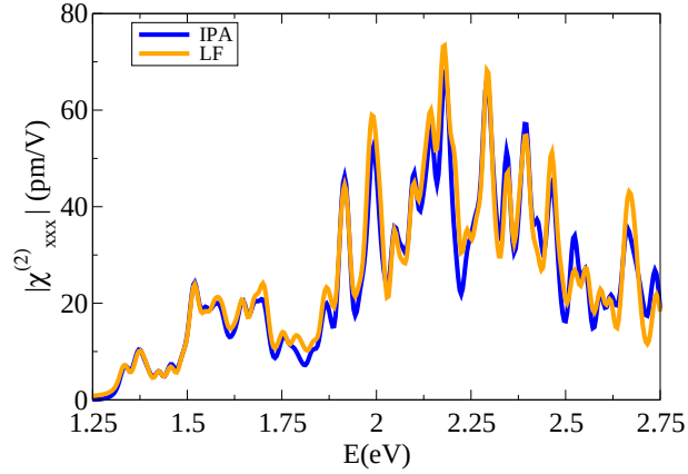
Figure 6.44: SHG spectra of the (\chi_M^{(2)} xxx) component calculated in the independent particle (IPA, blue line) and local fields (LF, orange line) approximations. LF effects are negligible along the homogeneous \mathbf{x} , \mathbf{y} directions.
