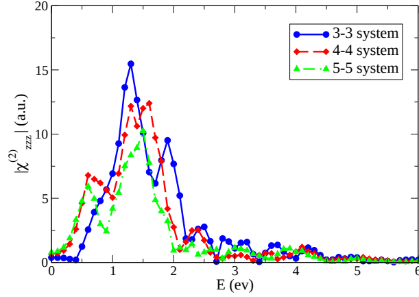
Figure G.7: Second-harmonic generation spectra of the Si surface composed of an equal amount of Si and vacuum ( n - n system). The IPA \chi_{zzz}^{(2)} component has been reported for the 3-3 (blue straight line), 4-4 (red dashed line) and 5-5 (green dotted-dashed line) systems. Contrary to the bulk response, the intensity decreases proportionally to the cell volume although the ratio \frac{V_{vac}}{V_{sys}} is constant, being characteristic of the surface. The spectrum converges in the 5-5 system, showing the larger amount of underlying Si required by the nonlinear optical process with respect to the linear one.
