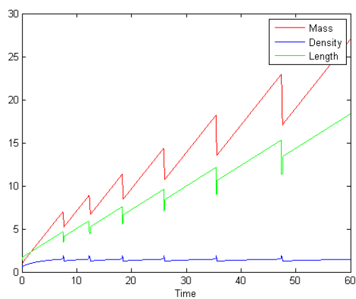
Figure 6.4: Mass, density and length oscillatory behavior for \gamma = 1.5 , q = 0 , \rho_{max} = 1.5 , \hat{\rho} = 1 , \rho_0 = 1 , K = 1 , E = 2 , \dot{m} = 1 , \alpha = 0.2
