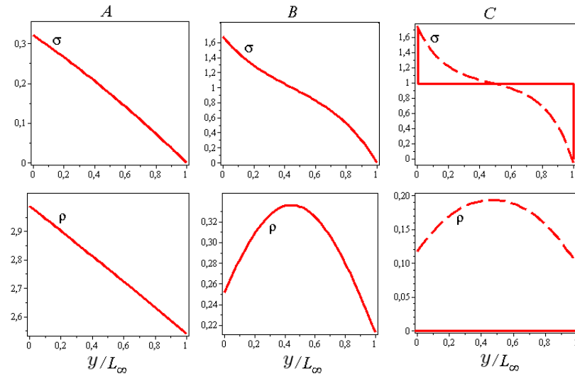
Figure 4.3: Stress and density distribution inside a moving cell in the regimes indicated as A, B and C in Fig.4.2. Dashed line shows elasticity-regularized profiles corresponding to point C' in Fig.4.15.
