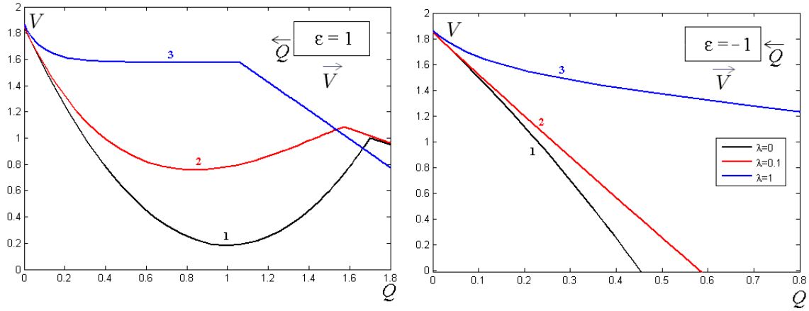
Figure 4.17: Force-velocity curves for the Maxwell model with \lambda_{1,2,3} = \{0, 0.1, 1\} . Experimental data suggest that \lambda = 0.02 - 0.2 [95, 122, 137, 156, 189]. Other parameters are \rho_0 = 1 , v_- = 1.7 and v_+ = 2 .
