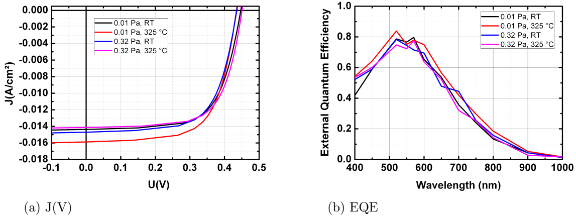
Figure 5.13: Illuminated current density voltage measurements and external quantum efficiency for \mu\text{c-Si:H} on ZnO:Al front contact deposited at various substrate temperatures and working pressures. The characteristics are measured after annealing of the solar cell at 150\text{ }^\circ\text{C} , during 30 minutes.
