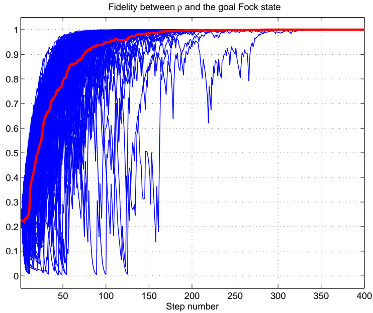
Figure 3.4: \text{Tr}(\rho_k \bar{\rho}) = \langle 3 | \rho_k | 3 \rangle versus k \in \{0, \dots, 400\} for 100 realizations of the closed-loop Markov process (3.12) with feedback (3.11) (blue fine curves) starting from the same state \chi_0 = (\mathbb{D}_{\sqrt{3}}(|0\rangle\langle 0|), 0, \dots, 0) and with 5-step delay ( \tau = 5 ). The ensemble average over these realizations corresponds to the thick red curve.
