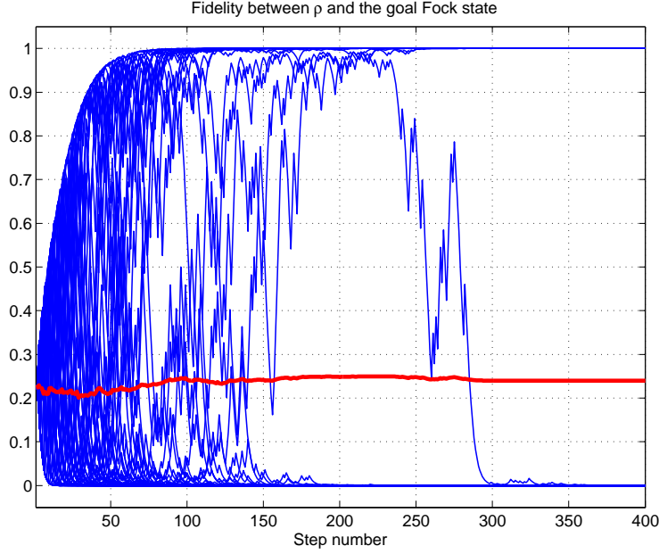
Figure 3.2: Fidelity with respect to the 3-photon state \langle 3 | \rho_k | 3 \rangle versus the number of passing atoms k \in \{0, \dots, 400\} for 100 realizations of the open-loop Markov process (3.6) (blue fine curves) starting from the same coherent state \rho_0 = \mathbb{D}_{\sqrt{3}}(|0\rangle\langle 0|) . The ensemble average over these realizations corresponds to the thick red curve.
