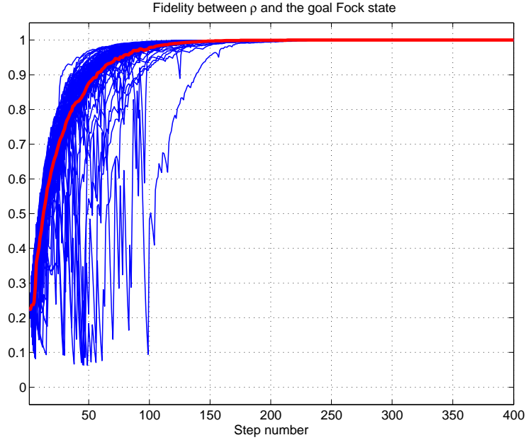
Figure 3.3: Fidelity with respect to the 3-photon state \text{Tr}(\rho_k \bar{\rho}) = \langle 3 | \rho_k | 3 \rangle versus k \in \{0, \dots, 400\} for 100 realizations of the closed-loop Markov process (3.2) with feedback (3.10) (blue fine curves) starting from the same state \rho_0 = \mathbb{D}_{\sqrt{3}}(|0\rangle\langle 0|) (no delay, \tau = 0 ). The ensemble average over these realizations corresponds to the thick red curve.
