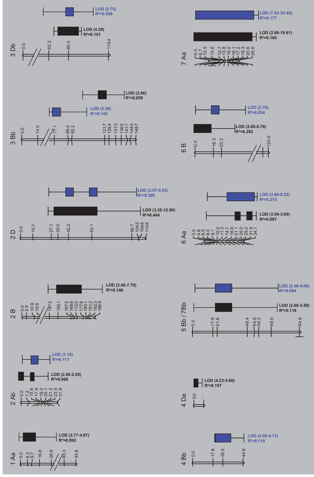
Figure 5. QTLs of quantitative resistance to wheat leaf rust identified in the Apache x Balance DH population, against isolate P5 (black bars) and isolate P3 (blue bars). The minimal and maximal LOD value (when LOD value was higher than 2), and the R^2 value are given. The bars include linkage group regions containing markers, which LOD value exceed the LOD threshold value of 1000 permutations. For QTLs with LOD rank 1, bars represent linkage group regions containing markers with \text{LOD} > 2.5 . For each QTL, the confidence interval figured result from the superposition of the different confidence intervals obtained from the different analyses. Genetic positions (in centimorgans) of the markers are indicated on the right side of the chromosome bars.
