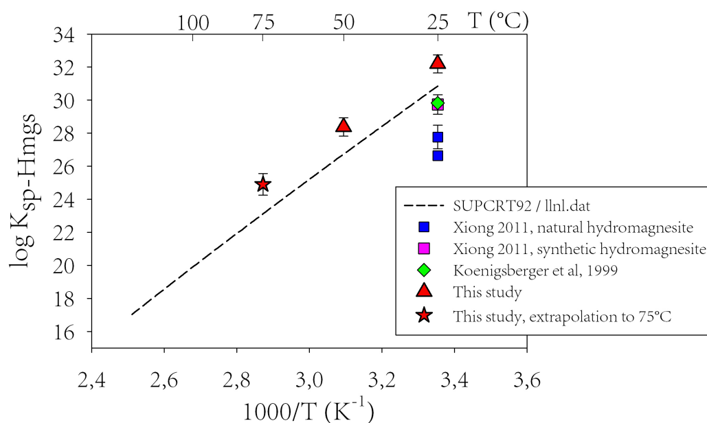
Figure 6.6 – Logarithm of the solubility product of hydromagnesite obtained in this study versus reciprocal temperature, and comparison to literature values.
