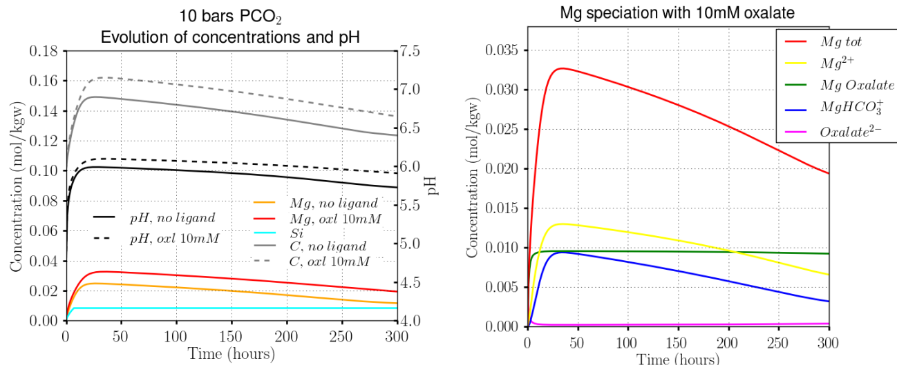
Figure 4.14 – (Left) Evolution of pH, and Mg and Si concentration during carbonation of 10g of forsterite in 1kg of water under a CO 2 pressure of 10 bars, in the absence and in presence of 10 mM oxalate. For Si, the introduction of oxalate did not have significant consequences. Thus, only one curve has been represented. (Right) Corresponding evolution of magnesium and oxalate chemical speciation in the presence of 10 mM oxalate. Only the main species have been represented. In conditions where Mg is in large excess compared to oxalate, a substantial proportion of the total Mg is present under the free Mg 2+ form.
