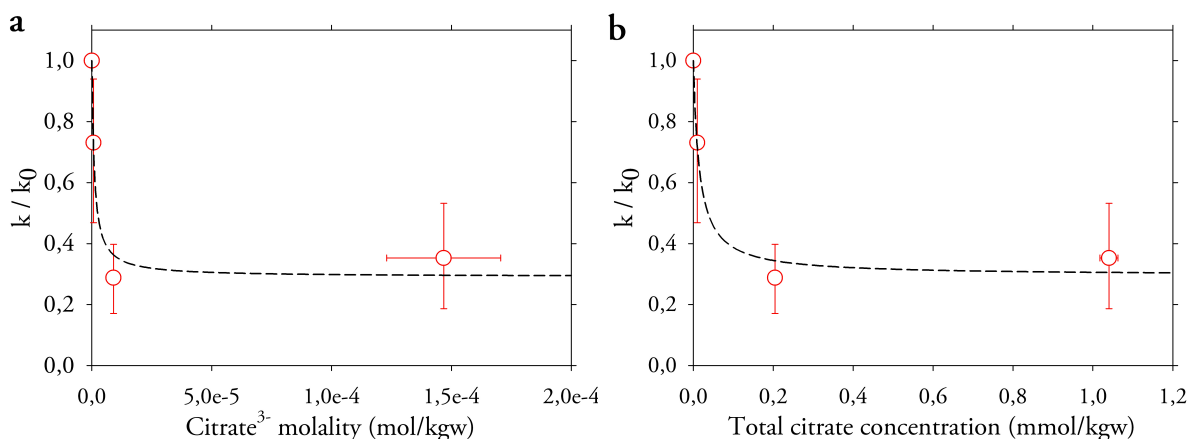
Figure 4.11 – Magnesite growth rate constants at 120°C normalized to the ligand-free constant k_0 , plotted as a function of (a) the free Citrate 3- molality and (b) the total citrate concentration. Black dashed lines are best fits of the data according to eq. 4.11. Datapoints corresponding to 0.1 mM citrate concentration (exp. Cit2 and Cit9) have been voluntarily omitted from these graphs due to important uncertainties on the rate constant.
