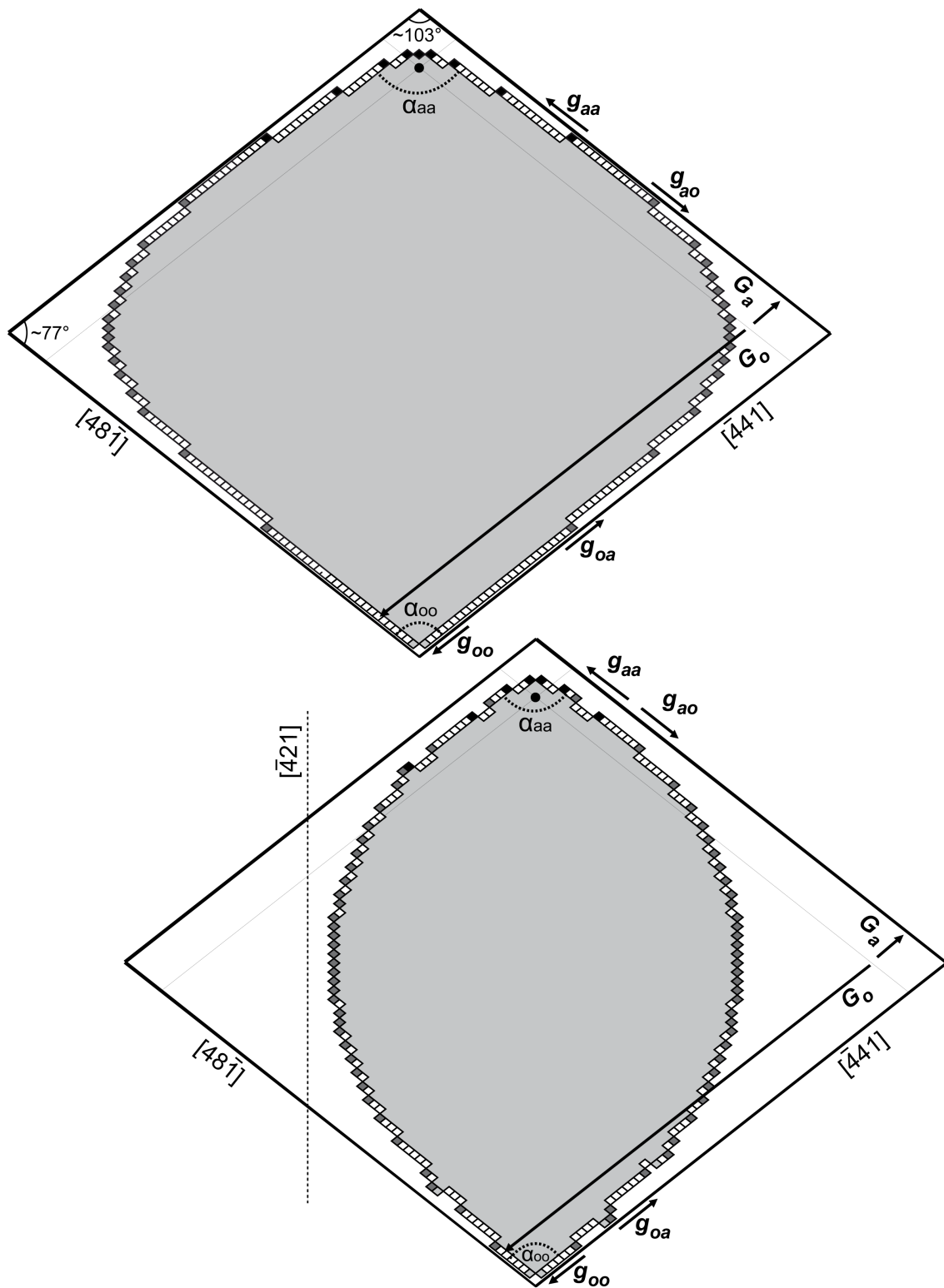
Figure 5.10 – Interpretative sketches of the shape of magnesite hillocks grown at 100°C, ( top ) in the absence of ligands at \Omega = 40 , and ( down ) in the presence of 10 mM citrate at 30 < \Omega < 50 . The different kink-sites are color-coded: g_{oo} , black; g_{oa} = g_{ao} , dark grey; g_{aa} , pale grey; white = no kink-site. The black circle represents the origin of the island, and the enveloping rhombus corresponds to an ideal magnesite hillock with g_{oo} \approx g_{oa} \approx g_{aa} . Its size is a measure of the step velocity of acute ( G_a ) and obtuse ( G_o ) steps with respect to the origin of the island.
