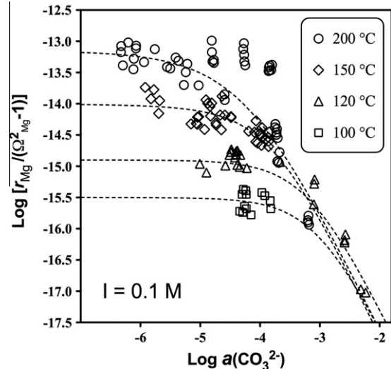
Fig. 6. Logarithmic plot of magnesite precipitation rates divided by (\Omega_{Mg} - 1) as a function of reactive fluid aqueous \text{CO}_3^{2-} activity from 100 to 200 °C. Symbols represent experimental data, whereas the dashed curves were calculated using Eq. (10) and the parameters listed in Table 7. Note that only rates obtained in 0.1 mol/kg aqueous NaCl solution are shown in this graph.
