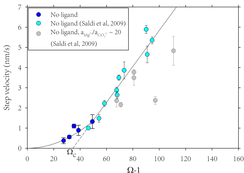
Figure 5.7 – Obtuse step velocity as a function of saturation state, without organic ligands. The fit is linear above \Omega \sim 50 , in accordance with equation 5.4. The fit crosses the x axis at \Omega_c . For \Omega < 50 , the data have been fitted with an empirical second-order rate law.
