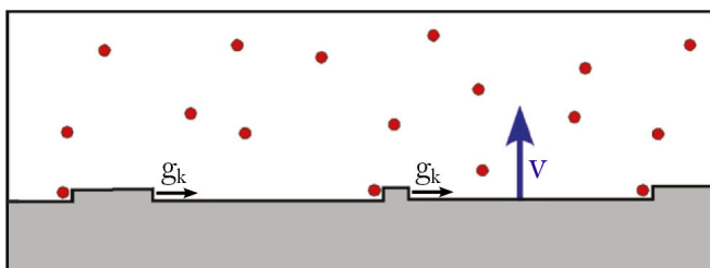
Figure 5.12 – Illustration of the kink-blocking model in the case of smooth steps (modified from De Yoreo et al. , 2009). Kinks propagate at the g_k rate, unless they are blocked by an impurity. The step may advance at its impurity-free velocity v as long as one kink orientation is free of impurity. This would ultimately result in a change of step orientation.
