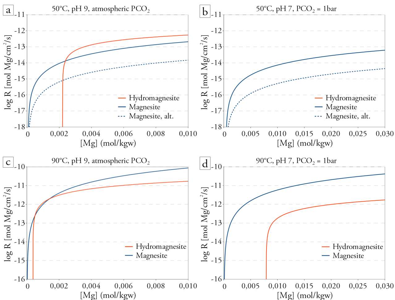
Figure 6.12 – Hydromagnesite and magnesite growth rates as a function of Mg concentration for different case studies (see text). The absence of hydromagnesite curve in graph (b) reveals that hydromagnesite always remains undersaturated in this simulation. The dotted lines in graphs (a) and (b) are magnesite growth rates predicted with a rate constant of 10^{-18} \text{mol/cm}^2/\text{s} , and materialize the impact of a lower-than-extrapolated magnesite growth rate constant at 50°C.
