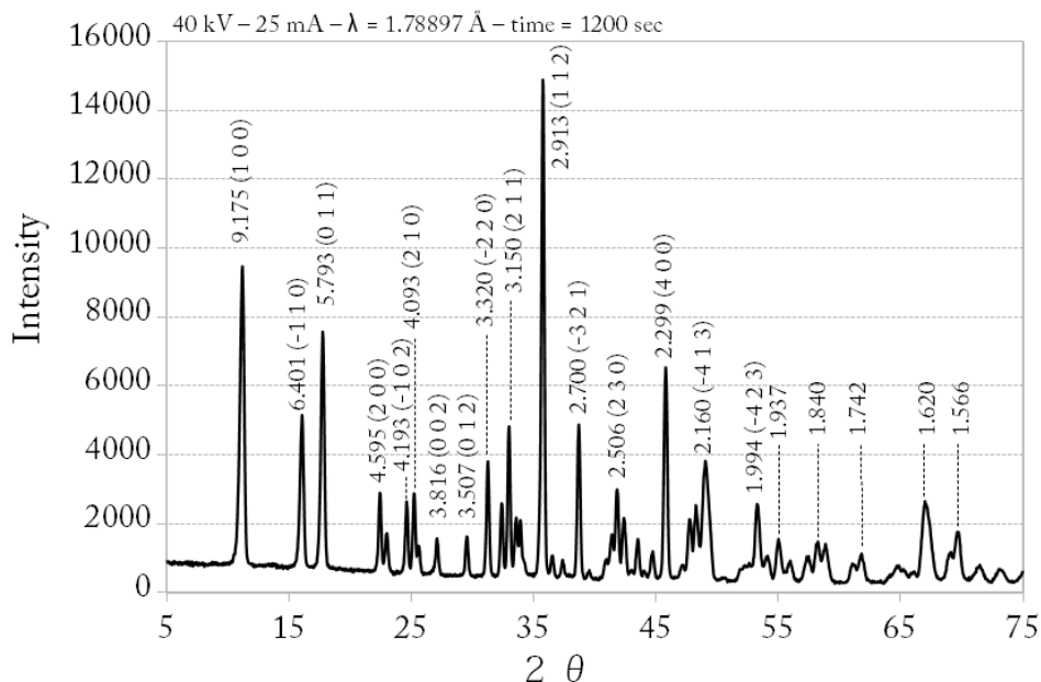
Figure 6.2 – Diffractogram of the powdered seed material with crystallographic indexation of the main peaks. All peaks correspond to hydromagnesite.
