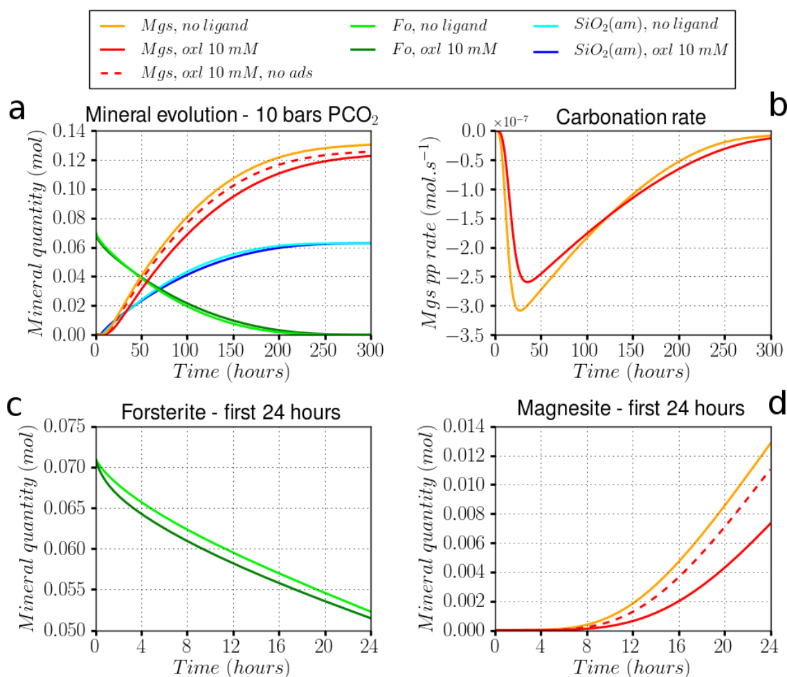
Figure 4.12 – Simulation of the carbonation of 10g of forsterite in one kilogram of water under a 10 bars CO 2 pressure, in the absence of any ligands and in the presence of 10 mM of oxalate: (a) Evolution of the quantity of forsterite, magnesite, and amorphous silica during a 300h carbonation simulation. The dashed line represents the evolution of precipitated magnesite in the presence of 10 mM oxalate, when the inhibiting influence of oxalate on magnesite precipitation due to adsorption at the mineral surface is not taken into account. (b) Carbonation rate (rate of magnesite formation) as a function of time. (c) and (d) Detail of the evolution of forsterite and magnesite during the first 24h of the simulation.
