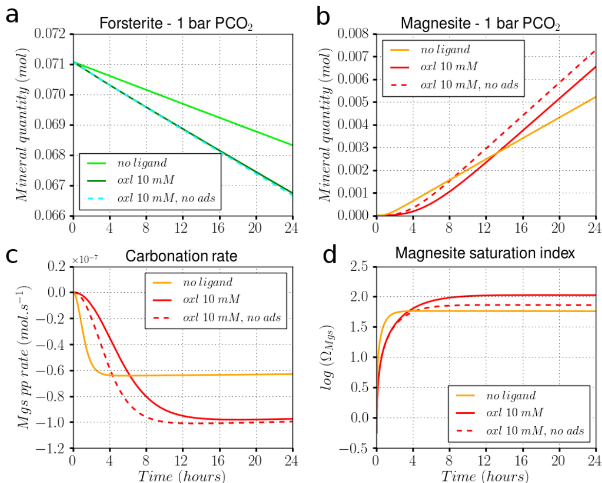
Figure 4.13 – Simulation of the carbonation of 10g of forsterite in one kg of water under a 1 bar \text{CO}_2 pressure, with and without 10 mM of oxalate, with an initial pH fixed to 7.5: (a) and (b) Evolution of the quantity of forsterite and magnesite during the first 24h of the simulation. Amorphous silica did not form within this time frame. Dashed lines represent the evolution of minerals amounts in the presence of 10 mM oxalate, when the inhibiting influence of oxalate on magnesite precipitation is not taken into account. (c) Carbonation rate, with and without oxalate. (d) Corresponding evolution of magnesite saturation index ( SI = \log \Omega_{\text{Mgs}} ).
