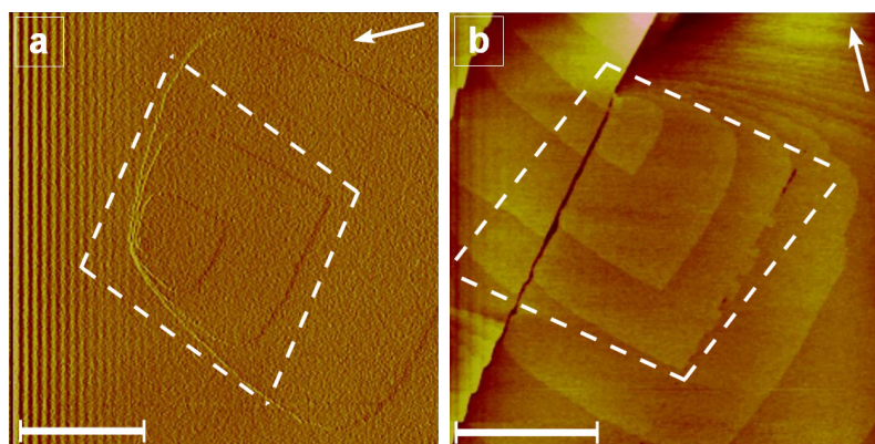
Figure 5.6 – HAFM images of magnesite hillocks at 100^\circ\text{C} in the presence of 10 mM EDTA. The scale bars corresponds to 1 \mu\text{m} .
