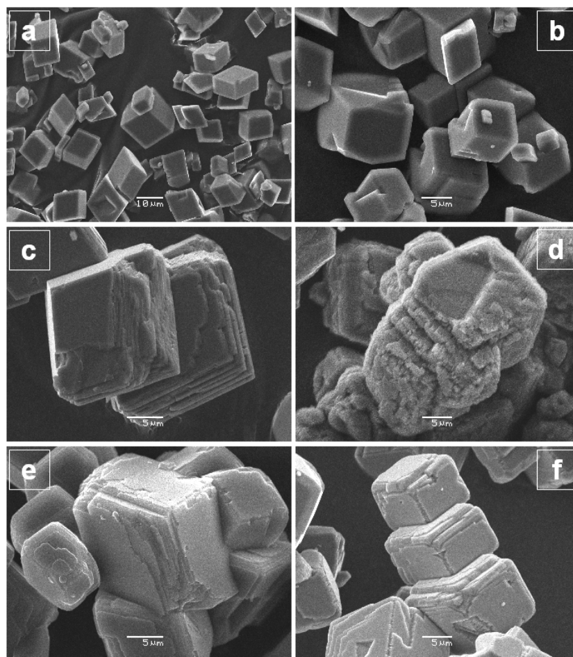
Figure 4.1 – Secondary electron SEM pictures of [a] & [b] synthesized magnesite seeds, [c] crystals grown at 120°C in the absence of ligands (exp. M24), [d] crystals grown at 120°C in the presence of 1 mM of citrate (exp. Cit8), [e] crystals grown at 146°C in the absence of ligands (exp. M28), and [f] crystals grown at 146°C in the presence of 10 mM of oxalate (exp. M9). Note the highly serrated aspect of the overgrown layers in the presence of citrate, whereas oxalate does not strongly affect the shape of precipitated layers.
