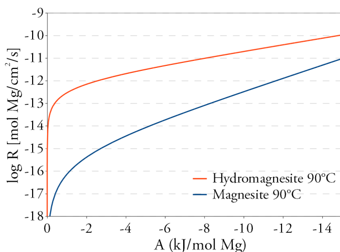
Figure 6.11 – Comparison of surface area-normalized hydromagnesite and magnesite growth rates at 90°C as a function of chemical affinity, normalized to one mole of Mg.
