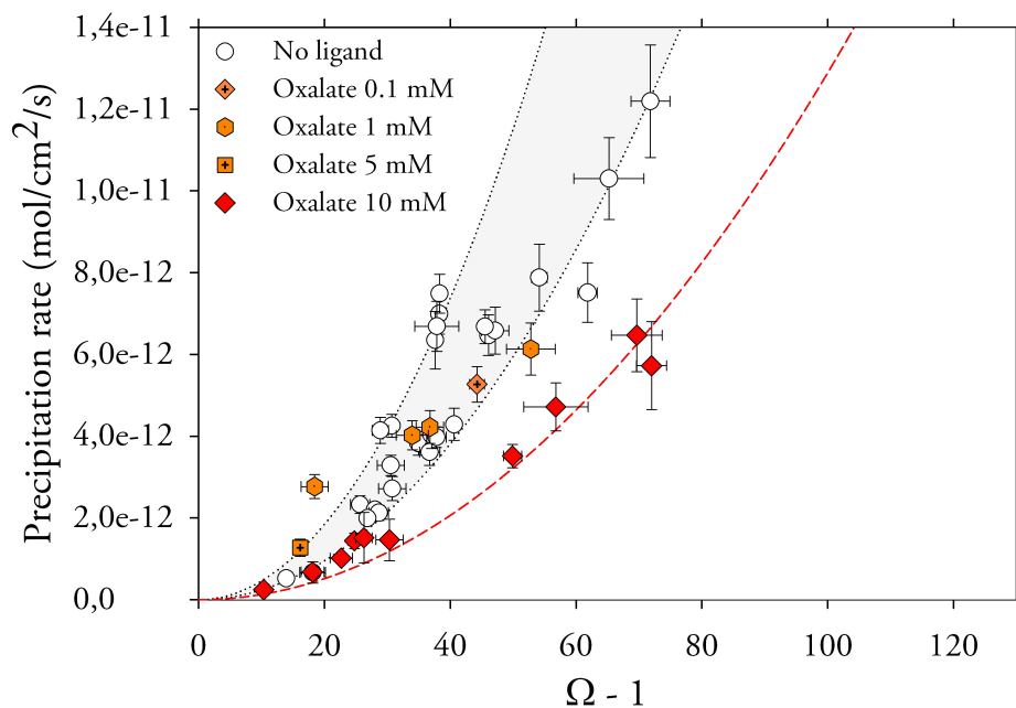
Figure 4.7 – Magnesite growth rates as a function of the degree of supersaturation at 120°C in the absence of ligands, and in presence of various concentrations of oxalate. The grey shaded area represents the range of variability of inorganic rates, while the red dashed line is a best fit according to rate law 4.8 of rates measured in the presence of 10 mM oxalate.
