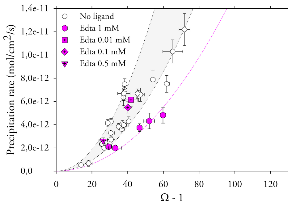
Figure 4.8 – Magnesite growth rates at 120°C in the absence of ligands, and in presence of various concentrations of EDTA. Growth rates measured in the presence of 1 mM EDTA are satisfyingly fitted by rate law 4.8, as shown by the pink dashed line.
