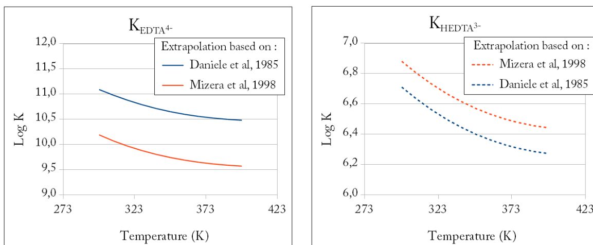
Figure 3.7 – First and second protonation constants of EDTA as a function of temperature.
