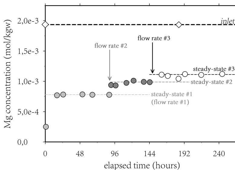
Figure 4.2 – Evolution of Mg concentration in the outlet fluid during experiments Cit5A to Cit5C. White rhombs represent the inlet solution Mg concentration. Inlet flow rate is modified after achievement of steady-state, which is verified with a minimum of 3 successive samples with identical concentrations over several residence times. In the present examples, flow rate # 1 is 0.5 mL/min, # 2 is 1.0 mL/min, and # 3 is 1.5 mL/min. The analytical uncertainty is less than the symbol size.
