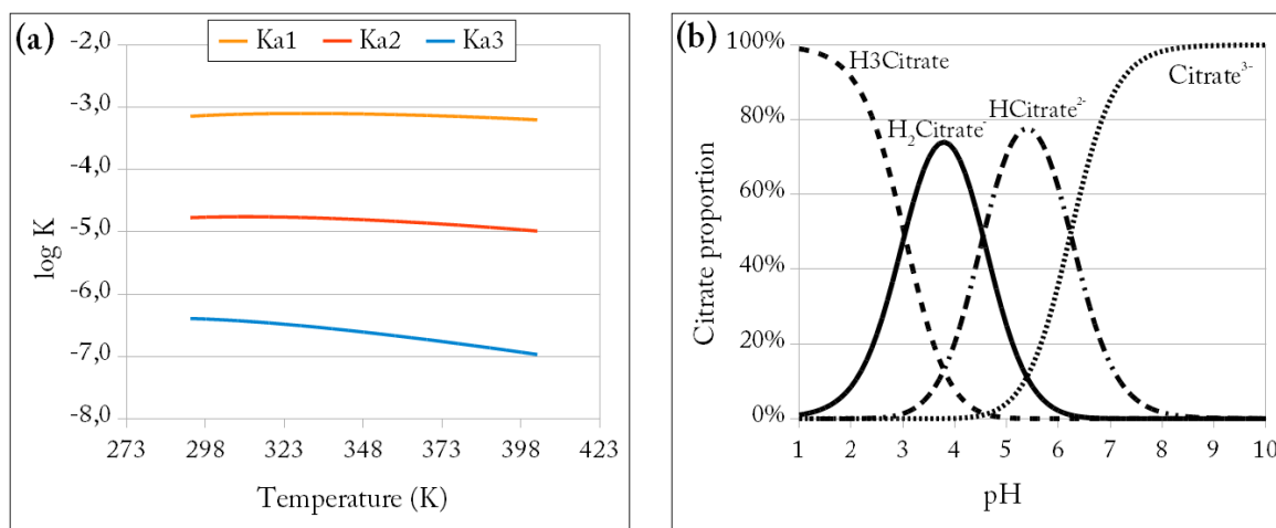
Figure 3.11 – (a) Dissociation constants of citric acid as a function of temperature, from Bénézeth et al. (1997) . (b) Citric acid speciation diagram at 120°C in a 0.1M ionic strength solution. There is little difference with the speciation diagram at 100°C.
