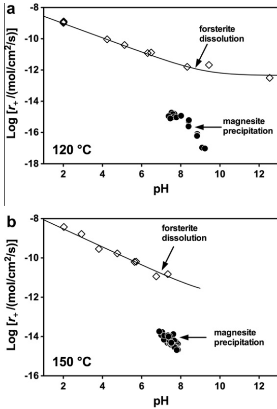
Fig. 11. Comparison of far from equilibrium forsterite dissolution rates reported by Hänchen et al. (2006) with corresponding r_+ values generated from magnesite precipitation rates determined in the present study as a function of pH (see text).
