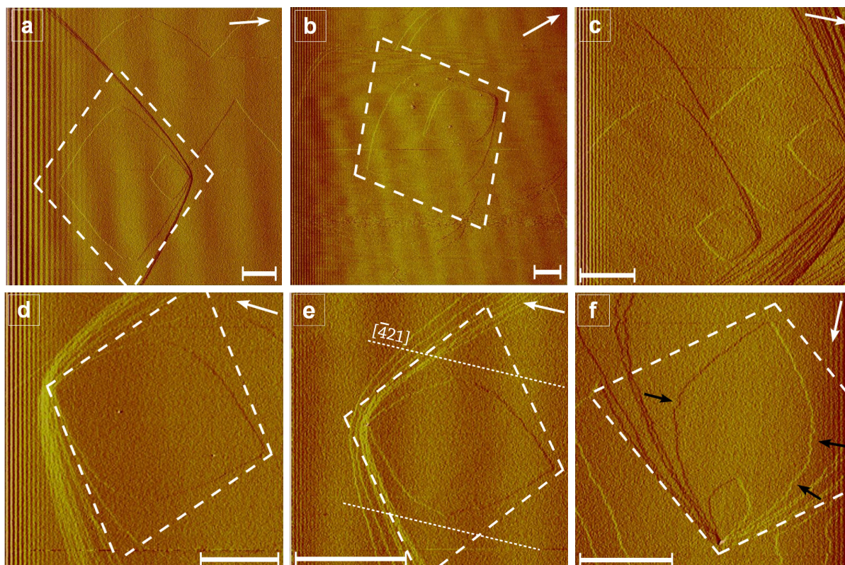
Figure 5.5 – HAFM deflection images of magnesite hillocks in the presence of various concentrations of citrate. The white arrows represent the orientation of the c-axis [001] plunging downward into the plane of the page. The scale bars correspond to 1 \mu\text{m} . The rhombus materialized by the dashed white lines represent the shape of an ideal magnesite rhombus and has been drawn for comparison with the actual hillock shape.
