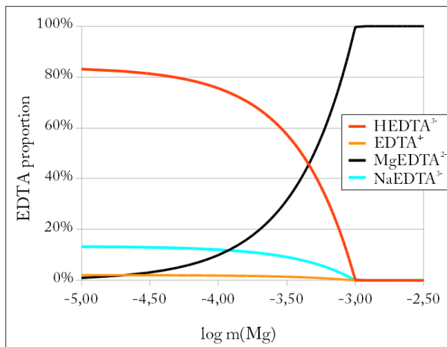
Figure 3.10 – Speciation of 1mM of EDTA at 120°C as a function of total magnesium molality (in \text{mol}\cdot\text{kgw}^{-1} ). The present example was drawn at pH 8, with 90mM of NaCl as background electrolyte. Ionic strength is close to 0.1M. The proportion of \text{MgEDTA}^{2-} increases linearly with the Mg molality, leading to a complete domination of \text{MgEDTA}^{2-} on EDTA speciation in solution supersaturated with respect to magnesite.
