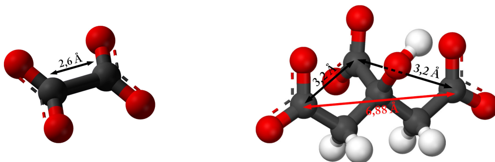
Figure 5.13 – Structure of oxalate (left) and citrate (right), with black spheres representing carbons, red spheres, oxygen, and white spheres, hydrogen. Arrows indicate the distances between carboxylic groups (in Å).
