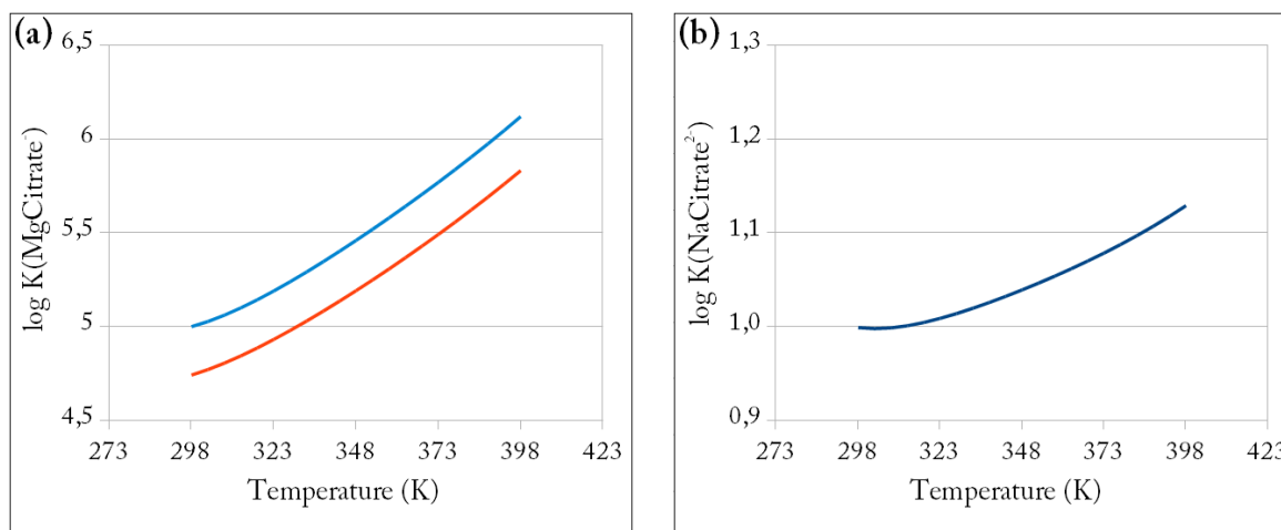
Figure 3.12 – (a) Calculated evolution of K_{\text{MgCitrate}^-} as a function of temperature. The two extrapolations represent a range of plausible values for the complexation constant. (b) Calculated evolution of K_{\text{NaCitrate}^{2-}} as a function of temperature, based on Zelenina & Zelenin (2005) .
