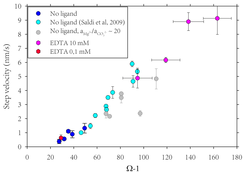
Figure 5.9 – Obtuse step velocity as a function of saturation state, in the presence of various concentrations of EDTA. EDTA does not visibly affect obtuse step advancement rate.
