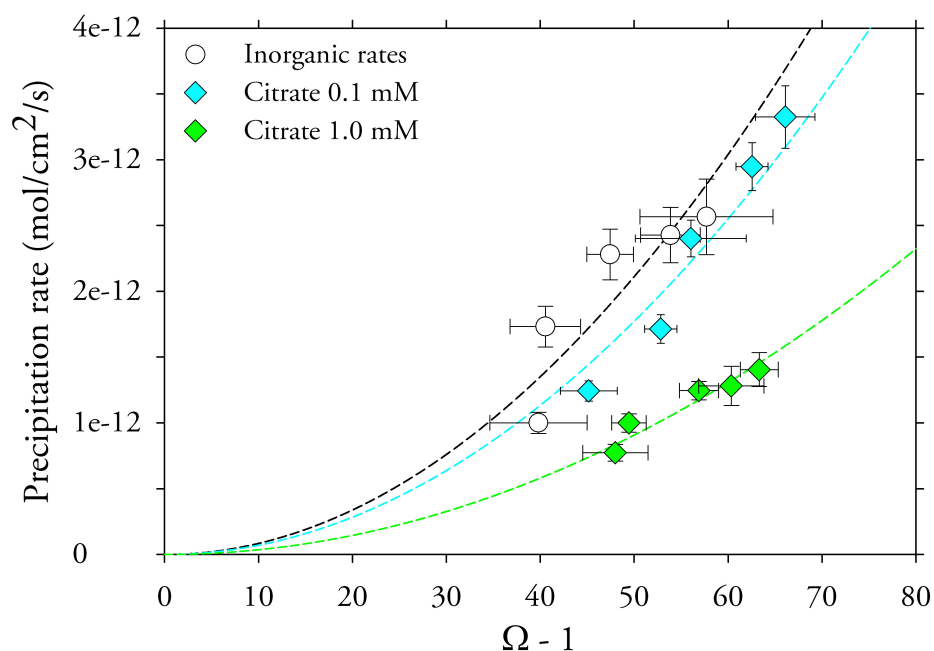
Figure 4.9 – Magnesite growth rates at 100°C in the absence and presence of citrate at concentrations 0.1 and 1 mM. Dashed lines are best fits of the results according to rate law 4.8. The apparent kinetic rate constant k'_{Mgs} is significantly decreased in the presence of citrate.
