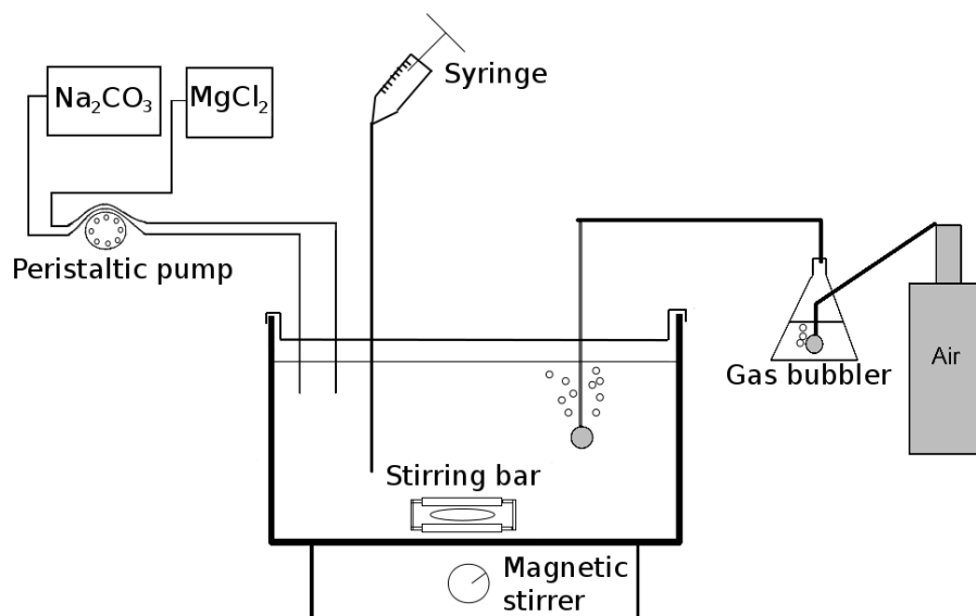
Figure 6.4 – Discontinuous mixed-flow reactor setting used for low temperature hydromagnesite growth experiments. Note that air bubbling was only used in a few preliminary experiments.
