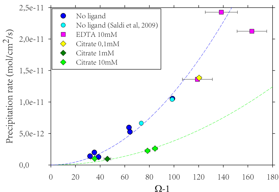
Figure 5.1 – HAFM-based magnesite growth rates at 100°C, plotted as a function of saturation state, in the absence and presence of organic ligands (citrate and EDTA). Experiments with citrate at concentrations of 1 mM or higher show a reduced growth rate of magnesite compared to the ligand-free case, whereas EDTA at a concentration of 10 mM does not affect growth rates. The dotted lines are best fits of the HAFM rates without ligand (blue), and with 1 mM citrate (green), according to equation (5.3).
