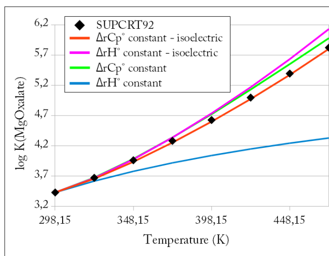
Figure 3.5 – Complexation constant of Oxalate 2- with \text{Mg}^{2+} , from SUPCRT92 (black rhombs). The results of the different temperature extrapolation methods outlined in Section 3.2 have been drawn for comparison. The constant heat capacity approximation obtained via isoelectric writing of reaction (3.24) gives the best results (see text).
