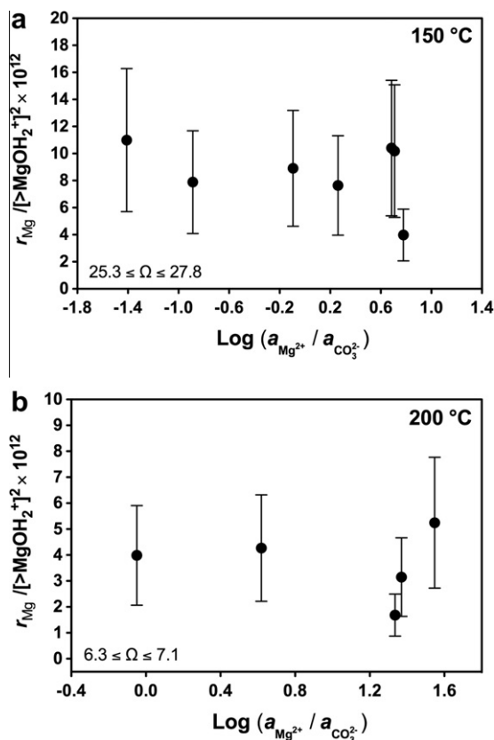
Fig. 9. Magnesite precipitation rates normalized to the square of the corresponding concentration of the rate-controlling species ( >\text{MgOH}_2^+ ) plotted against the logarithm of the aqueous \text{Mg}^{2+}/\text{CO}_3^{2-} activity ratio at 150 (a) and 200 °C (b) for the indicated constant degree of supersaturation. Both plots show that magnesite precipitation rates are essentially independent of \text{Mg}^{2+} to \text{CO}_3^{2-} activity ratio at the considered conditions.
