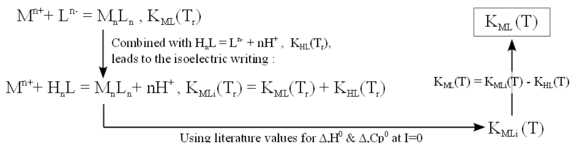
Figure 3.1 – General procedure for extrapolation of equilibrium constants to higher temperatures. K_{ML} is the equilibrium constant of the given complexation reaction, K_{HL} is the constant of the dissociation reaction used to write the isoelectric form of the complexation reaction, K_{MLi} is the equilibrium constant of the isoelectric reaction.
