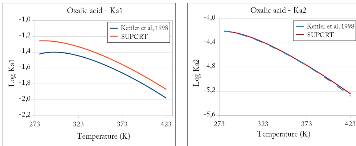
Figure 3.3 – First and second dissociation constants of oxalic acid as a function of temperature. The agreement between Kettler et al. (1998) data and SUPCRT92 estimates is good for K_{a2} , but some differences exist for K_{a1} .
