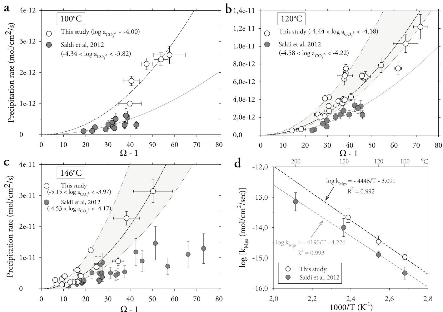
Figure 4.3 – (a) to (c): Magnesite growth rate as a function of the degree of supersaturation ( \Omega - 1 ) at (a) 100, (b) 120, (c) 146°C. Dashed lines are best fits according to eq. 4.8. Grey-shaded areas limited by dotted lines in (b) and (c) highlight the observed variability. Rates measured by Saldi et al. (2012) in comparable chemical conditions are represented as dark grey circles. Fig. (d) represents an Arrhenius plot of retrieved rate constants as a function of reciprocal temperature. Dashed lines are linear least square fits of the rate constants. The slopes are consistent with an activation energy of 85.1 \pm 7.7 kJ/mol in the present study, 80.1 kJ/mol in the study by Saldi et al. (2012).
