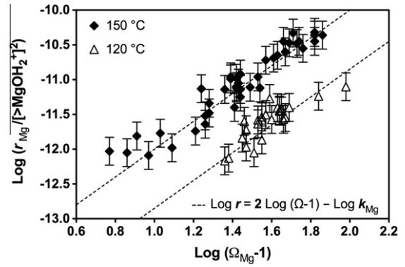
Fig. 8. Logarithmic plot of magnesite precipitation rates measured in fluids containing 0.1 mol/kg NaCl normalized to the square of the concentration of the rate controlling surface species, [>\text{MgOH}_2^+] , versus (\Omega_{\text{Mg}} - 1) . The dashed lines were calculated using Eq. (10), n = 2 and parameters listed in Table 7 for the corresponding T . Error bars correspond to 0.2 log units.
