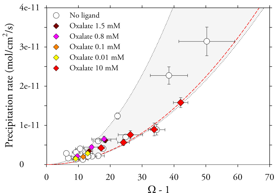
Figure 4.6 – Magnesite growth rates as a function of the degree of supersaturation at 146°C in the absence of ligands, and in presence of various concentrations of oxalate. The grey shaded area represents the range of variability of inorganic rates, while the red dashed line is a best fit according to rate law 4.8 of rates measured in the presence of 10 mM oxalate.
