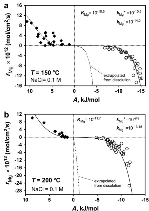
Fig. 10. Comparison of magnesite precipitation rates measured in this study with corresponding dissolution rates reported by Saldi et al. (2010). All rates were measured in 0.1 mol/kg NaCl solutions. The symbols in these plots represent measured rates, but the curves were computed using Eq. (10) together with the parameters reported in Table 7 and Saldi et al. (2010). The curves for precipitation at 150 and 200 °C were generated for a pH equal to 8.0 and 7.0, respectively, and assuming a constant total carbon concentration of 0.01 mol/kg, but those for dissolution were generated by adjusting pH for a solution containing 0.001 mol/kg of total carbon and 1 \times 10^{-5} mol/kg of Mg. The dotted-dashed curves on both plots represent the precipitation rates extrapolated from the dissolution data using Eq. (10) with the parameters provided by Saldi et al. (2010), for solution compositions representative of those used in this study.
