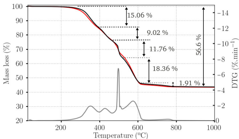
Figure 6.3 – Results of thermo-gravimetric analysis performed on the initial seed material (black curve) as well as on the precipitated material at 25^{\circ}\text{C} (exp. H11, red). The grey curve is the differential thermo-gravimetry (DTG), corresponding to the rate of weight loss. Four main decomposition steps are visible, at 353^{\circ}\text{C} , 428^{\circ}\text{C} , 498^{\circ}\text{C} and 575^{\circ}\text{C} , respectively. The first DTG peak corresponds to loss of four molecules of crystalline water, while the other peaks correspond to non-stoichiometric losses of \text{CO}_2 and \text{H}_2\text{O} .
