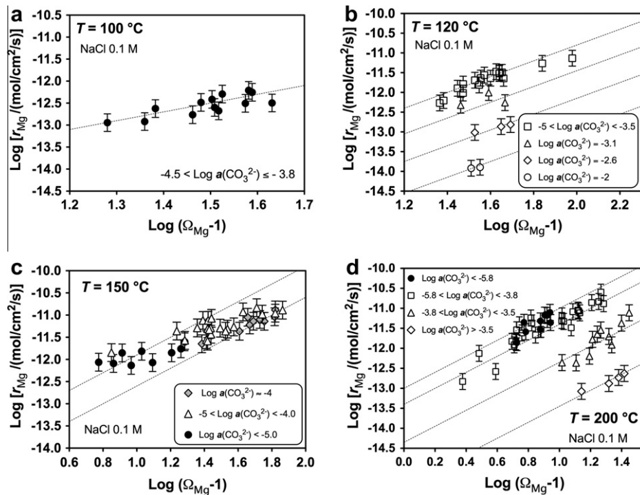
Fig. 4. Logarithmic plots of magnesite precipitation rates measured in fluids containing 0.1 mol/kg NaCl at (a) 100, (b) 120, (c) 150 and (d) 200 °C versus the degree of supersaturation ( \Omega_{Mg} - 1 ). The reactive fluid aqueous \text{CO}_3^{2-} activity of the experiment is indicated by the symbol as defined in the plots. Dashed lines have a slope consistent with n = 2 . Error bars correspond to an uncertainty of \pm 0.2 logarithmic units.
