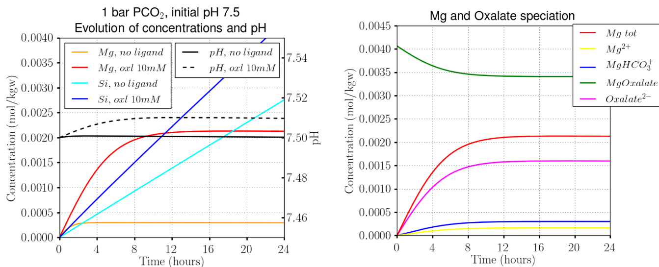
Figure 4.15 – (Left) Evolution of pH, Mg and Si concentration during carbonation of 10g of forsterite in 1kg of water under a CO 2 pressure of 1 bar, in the absence and in presence of 10 mM oxalate, at an initial pH of 7.5. Only the first 24h are represented here, corresponding to the results shown in Fig. 4.13.
