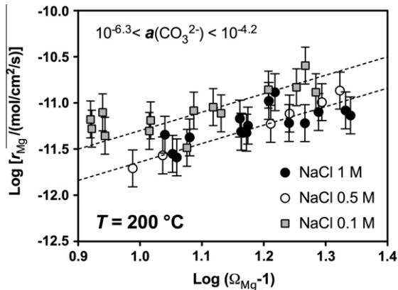
Fig. 5. Logarithmic plot of magnesite precipitation rates measured at 200 °C and in solution having a log aqueous \text{CO}_3^{2-} activity between -6.3 and -4.2 as a function of the degree of fluid supersaturation ( \Omega_{Mg} - 1 ). The dashed lines have a slope consistent with n = 2 . The grey squares, open circles, and filled circles correspond to precipitation rates measured in reactive fluids containing 0.1, 0.5, and 1.0 mol/kg NaCl, respectively. Error bars correspond to a \pm 0.2 log units uncertainty in measured rates.
