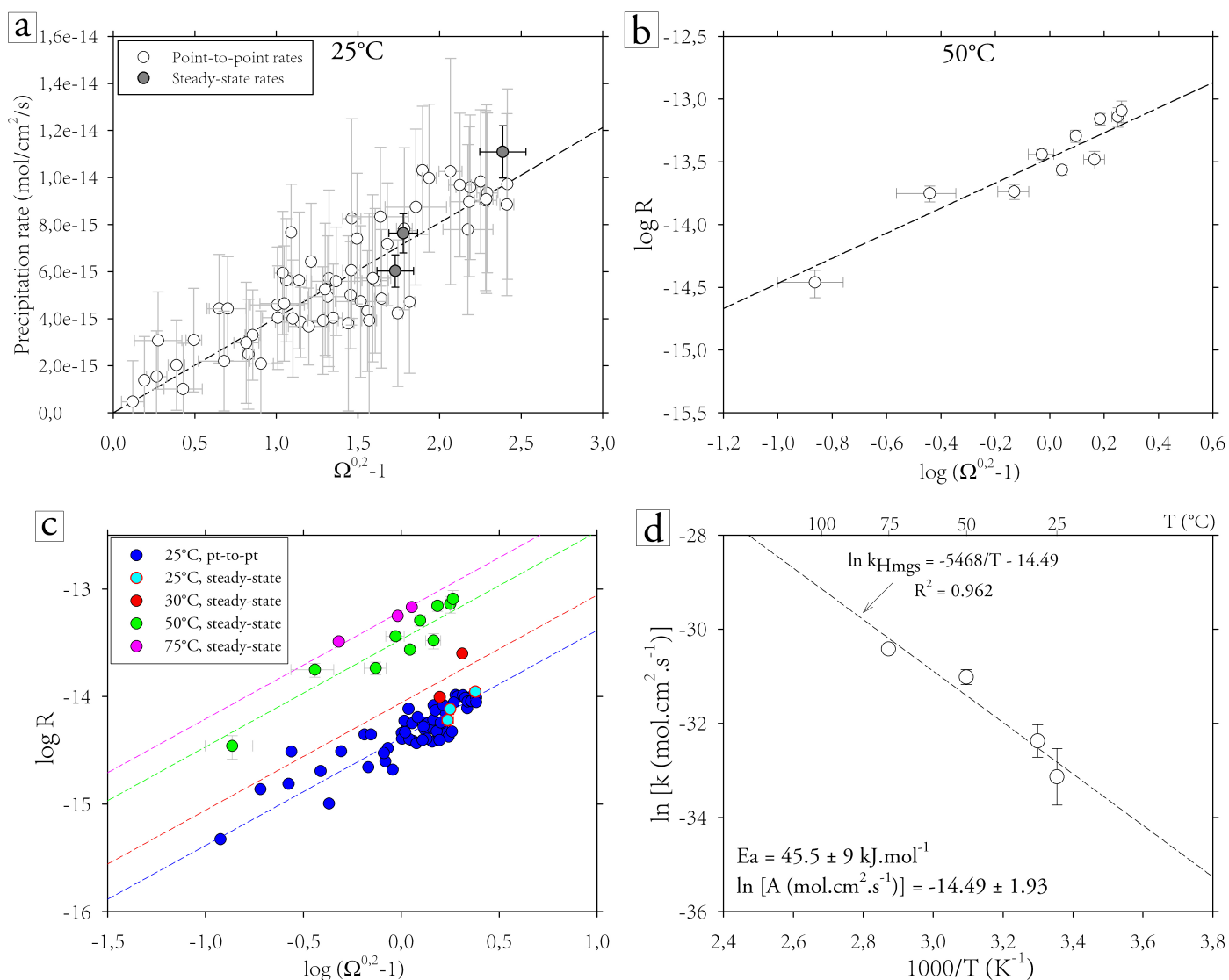
Figure 6.9 – (a) to (c) Plots of measured hydromagnesite growth rates versus supersaturation. Dashed lines slopes correspond to unit rate order. Error bars on "point-to-point" rates at 25°C have been omitted for clarity sake. Unless represented, error bars on "steady-state" rates are smaller than the symbol size. (d) Arrhenius plot of the rate constants obtained for n = 1 .
