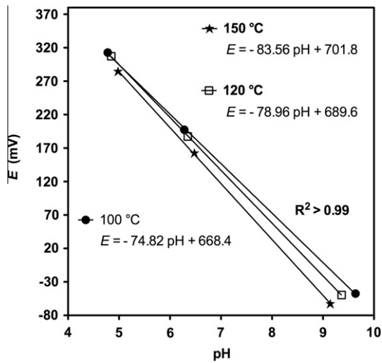
Fig. 2. Examples of the solid contact pH electrode coupled with a Na-selective reference electrode calibration at 100, 120, and 150 °C in aqueous 0.1 M NaCl solutions.
