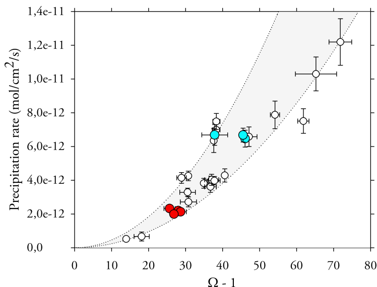
Figure 4.4 – Magnesite growth rates at 120°C, as a function of the degree of supersaturation. Blue: test experiments M27, M37 and M41. Red: test experiments M32A, M33A, M35A and M39A.
