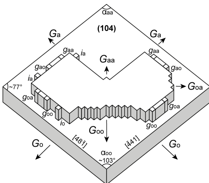
Figure 5.3 – Sketch of a magnesite growth hillock on the [104] surface. The upper step is built out of two merging hillocks in order to illustrate the different "rough" steps that may develop on the [104] surface (see Section 5.3.4). Abbreviations: G = step; g = kink site; i = kink-nucleation site; o = obtuse; a = acute. In the text, g_{xy} is used indistinctly to designate a given kink orientation, or its propagation rate.
