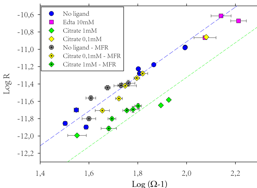
Figure 5.2 – Comparison between HAFM and MFR-based magnesite growth rates at 100°C in the absence and presence of organic ligands. MFR data were presented in Chapter 4. There is a good agreement between MFR rates normalized to geometrical surface area, and HAFM rates. In both cases, experiments with 1 mM citrate exhibit a reduced growth rate compared to ligand-free experiments. The dotted lines are best fits of the HAFM rates in ligand-free solutions (blue), and in the presence of 1 mM citrate (green), according to the log version of equation 5.3. The fits are consistent with a second-order rate law.
