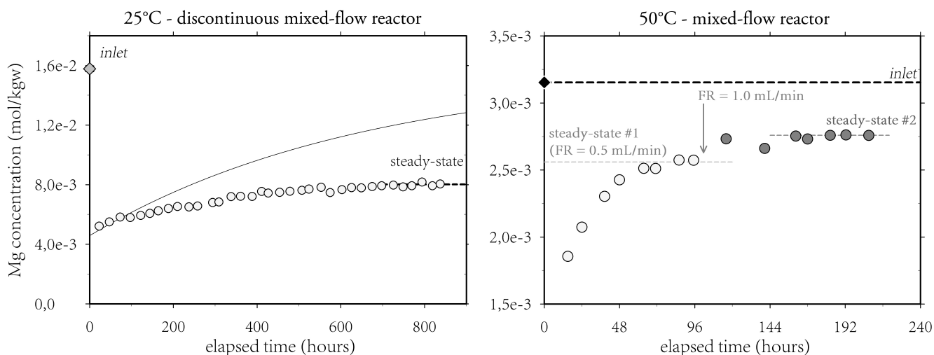
Figure 6.8 – Representative evolution of Mg concentration in the outlet fluid as a function of time during growth experiments performed at 25°C (exp. H10), and at 50°C (exp. H505). At left, the solid line represents the theoretical evolution of Mg concentration if no precipitation was taking place. At right, the graph presents a series of two experiments with different flow rates performed on the same mineral seeds. Analytical uncertainty is smaller than the symbol size.
