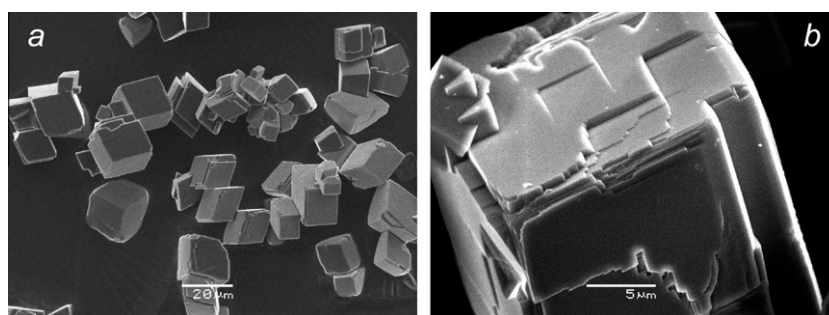
Fig. 1. SEM photomicrographs of synthetic magnesite used in the present study. (a) Example of magnesite powder after synthesis at 200 °C and a CO 2 pressure of 50 bar. (b) Detail of a magnesite crystal after a precipitation experiment performed in a mixed-flow reactor.
