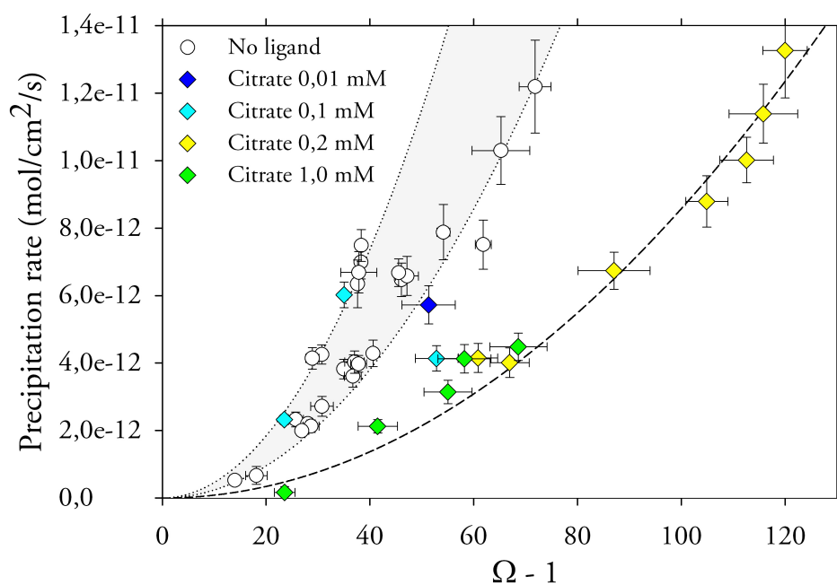
Figure 4.10 – Magnesite growth rates as a function of the degree of supersaturation at 120°C in the absence of ligands, and in presence of various concentrations of citrate. The dashed line is a best fit according to rate law 4.8 of rates measured in the presence of 0.2 mM citrate, and satisfyingly fits the rates obtained with 1 mM citrate.
