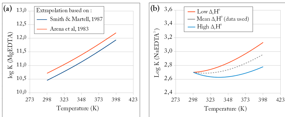
Figure 3.9 – (a) Stability constant of the \text{MgEDTA}^{2-} complex as a function of temperature (reaction 3.26). The two estimations are based on different initial \log K at 25°C, but uncertainty on reaction enthalpy and heat capacity was not taken into account. (b) Stability constant of the \text{NaEDTA}^{3-} complex as a function of temperature (reaction 3.27). Only one estimate at 25°C was selected, but the important uncertainty on reaction enthalpy was considered.
