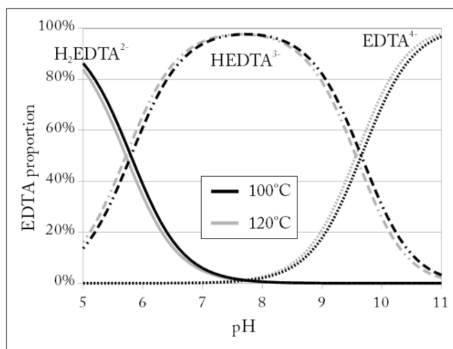
Figure 3.8 – Speciation diagram of EDTA at 100 and 120°C, at I \simeq 0.1 M, using the data from Daniele et al. (1985) for K_{\text{EDTA}^{4-}} and Thakur et al. (2007) for K_{\text{HEDTA}^{3-}} . In our chemical conditions, the speciation is largely dominated by HEDTA 3- .
