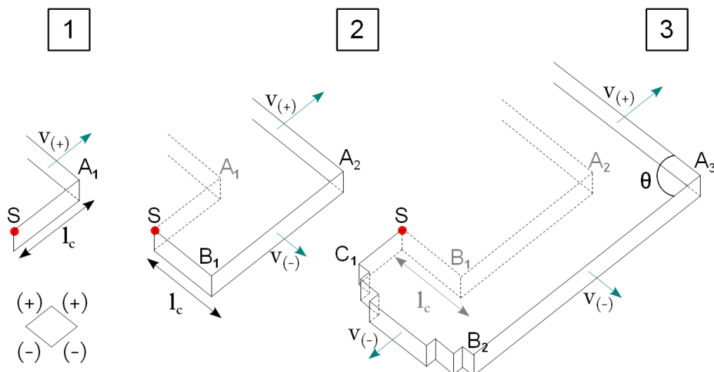
Figure 5.14 – Illustration of the spiral growth process on magnesite [104] surface. The rhombus in the lower left corner represents an ideal magnesite rhombus, and gives the orientation of the sketch. S is the source dislocation giving birth to the spiral (immobile).
