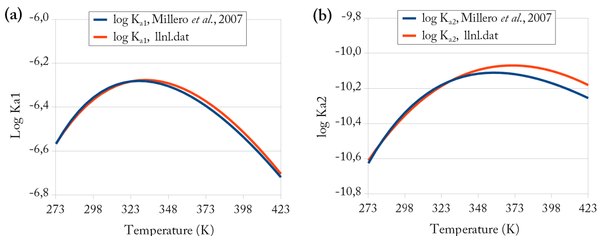
Figure 3.15 – (a) Carbonic acid first dissociation constant as a function of temperature. The data of the l1n1.dat database are in good agreement with Millero et al. (2007) . (b) Carbonic acid second dissociation constant as a function of temperature. There are substantial differences between the l1n1.dat data and Millero et al. (2007) , reaching up to 0.07 log units at 120°C.
