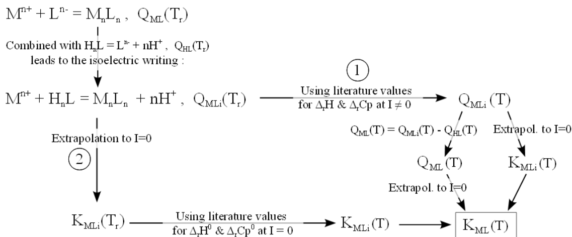
Figure 3.2 – Extrapolation procedure when thermodynamic data are only available at a given ionic strength I \neq 0 . Q designates the concentration quotients at equilibrium. If reaction enthalpy and heat capacity are only available at the same ionic strength, then the temperature extrapolation needs to be done on the concentration quotients, and extrapolation to infinite dilution is done afterwards (pathway 1). If reaction enthalpy and heat capacity have been reported at infinite dilution, then the extrapolation of the equilibrium constant to infinite dilution is done first, either on the initial concentration quotient Q_{ML} , or on the isoelectric quotient Q_{MLi} . Temperature extrapolation is done afterwards (pathway 2).
