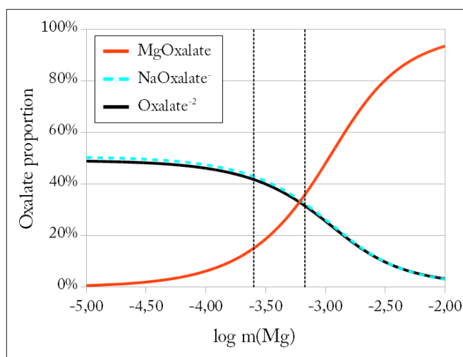
Figure 3.6 – Speciation of 1mM of oxalic acid at 120°C as a function of total magnesium molality (in \text{mol}\cdot\text{kgw}^{-1} ). The present example was drawn at pH 8, with 90mM of NaCl as background electrolyte. Ionic strength is close to 0.1M. \text{H}_2\text{Oxalate} and \text{HOxalate}^- are present in negligibly small quantities. Vertical dashed lines indicate the range of \text{Mg}^{2+} molality in our experiments with 1mM oxalate.
