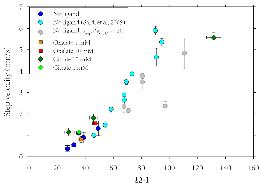
Figure 5.8 – Obtuse step velocity as a function of saturation state, in the presence of various concentrations of citrate and oxalate.
