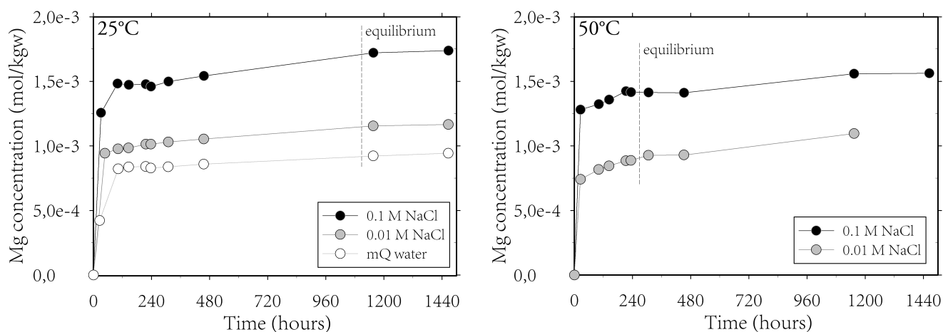
Figure 6.5 – Evolution of Mg concentration during the course of hydromagnesite solubility experiments at 25 and 50°C.
