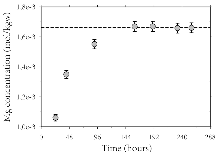
Figure 3.13 – Evolution of Mg concentration with time during the course of the magnesite solubility experiment. Stability of Mg concentration (as symbolized by the dashed line) indicates equilibrium is reached.
