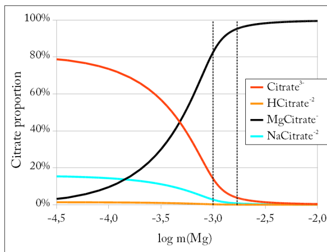
Figure 3.14 – Speciation of 1mM of citrate at 120°C as a function of total magnesium molality (in \text{mol}\cdot\text{kgw}^{-1} ). The present example was drawn at pH 8, with 90mM of NaCl as background electrolyte. Ionic strength is close to 0.1M. Vertical dashed lines indicate the range of \text{Mg}^{2+} molality investigated in our experiments with 1mM citrate.
