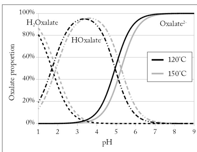
Figure 3.4 – Speciation diagram of oxalic acid at 120 and 150°C according to Kettler et al. (1998) . The speciation is largely dominated by \text{Oxalate}^{2-} at \text{pH} > 7 .
