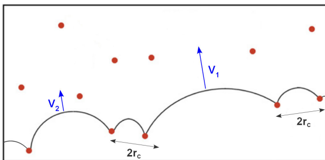
Figure 5.11 – Illustration of the step-pinning model (modified from Weaver et al. , 2007 ). Red dots represent impurities. If the distance between two adsorbed impurities is lower than 2r_c , the step segment in-between can only advance until its curvature radius reaches r_c . If impurity spacing is larger, the step segments advance at a velocity depending on their curvature ( V_1 > V_2 ).
