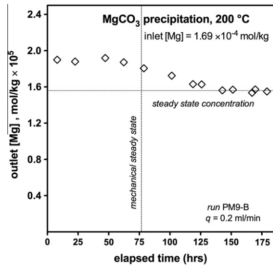
Fig. 3. Evolution of Mg concentration in the outlet fluid as a function of time during experiment PM9. Chemical steady-state is attained shortly after the time required for mechanical steady-state. The analytical uncertainty in the measurements is approximated by the symbol size.
