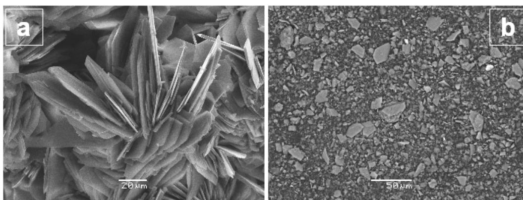
Figure 6.1 – SEM pictures of hydromagnesite seeds and precipitates. (a) Secondary electron (SE) image of a pristine hydromagnesite "flower" from the Lachambre cave network. (b) Backscattered electron (BSE) image of highly divided hydromagnesite fragments obtained after gentle grinding, and used for solubility and growth experiments. Bright spots correspond to aragonite fragments.
