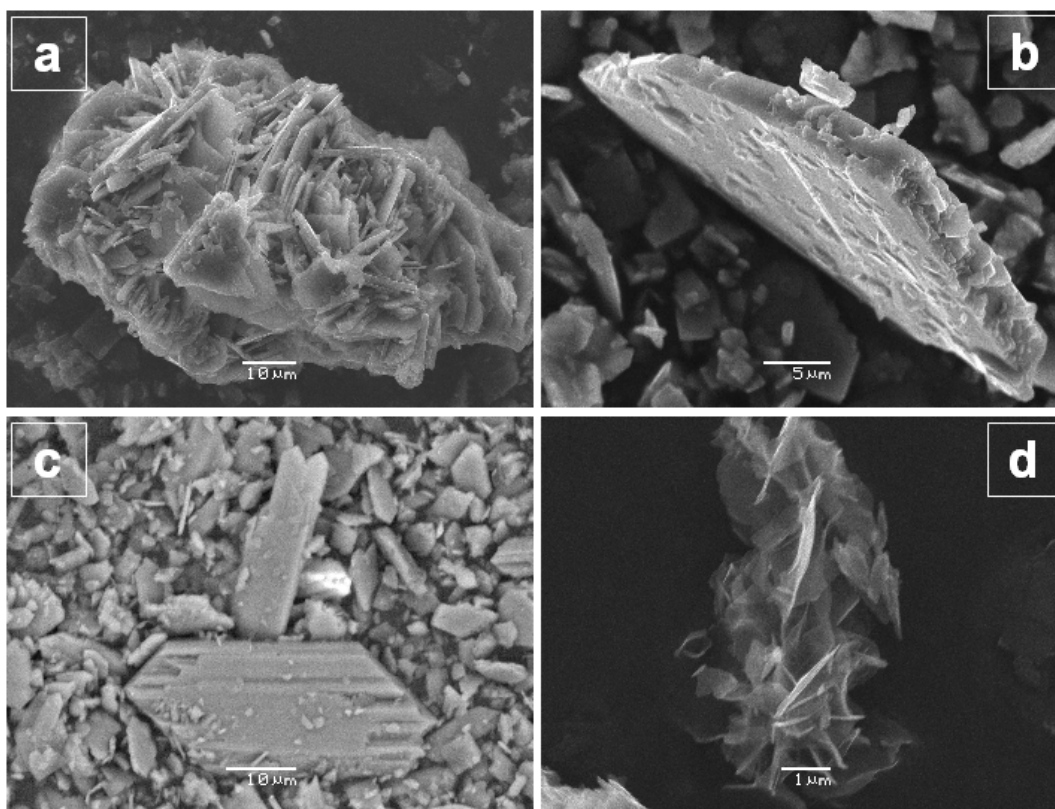
Figure 6.7 – SEM images of seed crystals after growth experiments. (a) Hydromagnesite agglomerate formed during precipitation at 25°C (secondary electrons). (b) Close-up view of the edge of one hydromagnesite crystal grown at 25°C (SE image). (c) BSE image of individual hydromagnesite crystals obtained after growth at 75°C. The (1 0 0) face is clearly visible. (d) SE image of dypingite obtained in unseeded experiments at 25°C.
