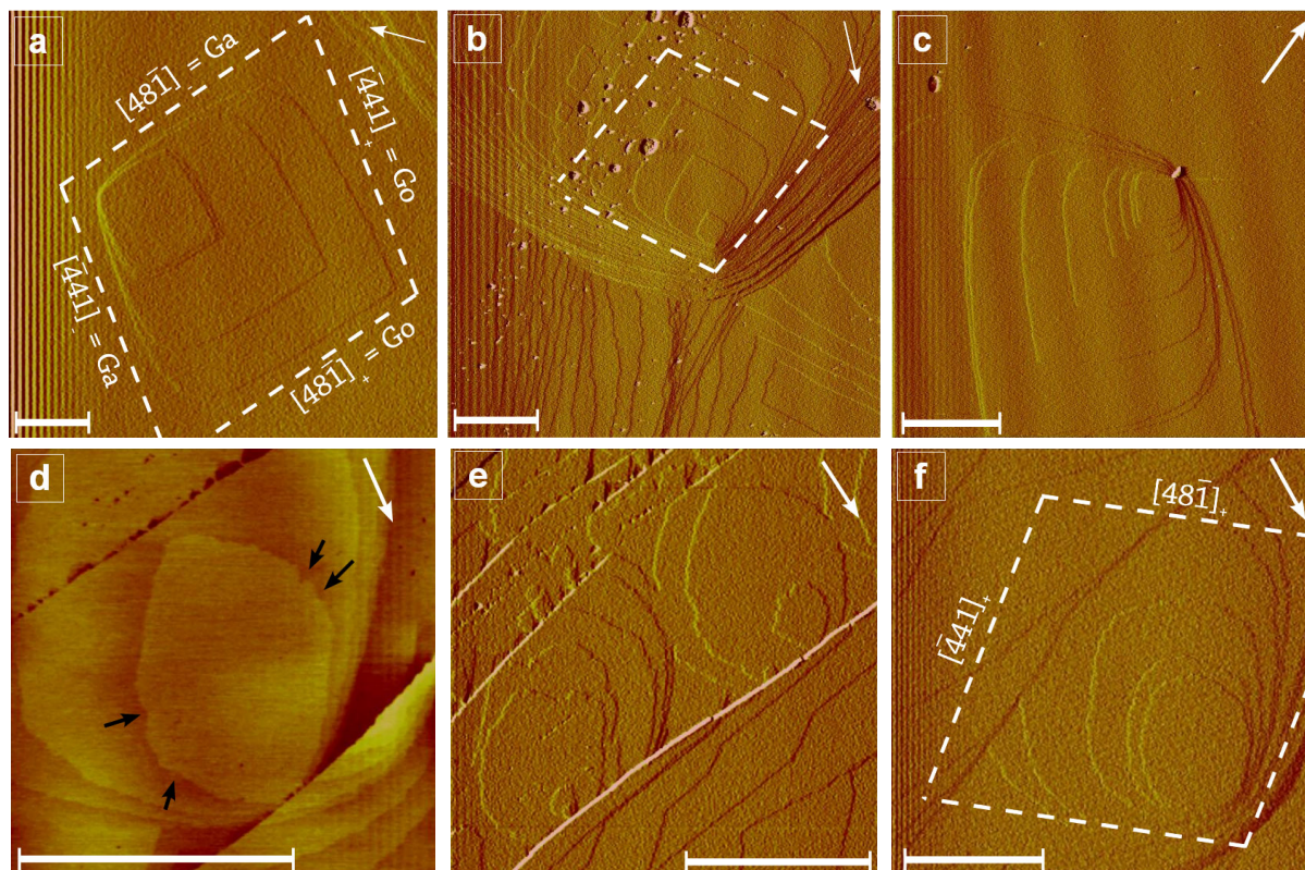
Figure 5.4 – HAFM images of magnesite hillocks in ligand-free conditions (a-c), and in the presence of oxalate (d-f). The white arrows represent the orientation of the c-axis [001] plunging downward into the plane of the page. The scale bars correspond to 1 \mu\text{m} . The rhombus materialized by the dashed white lines represent the shape of an ideal magnesite rhombus and has been drawn for comparison with the actual hillock shape.
