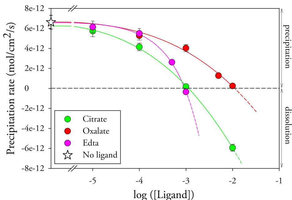
Figure 4.5 – Magnesite surface area normalized growth rates at 120°C as a function of the logarithm of total ligand concentration, at otherwise constant solution composition. The white star symbolizes the growth rate measured in the absence of ligands from a reference solution containing 1 mM Mg, 18 mM NaHCO 3 , at pH 7.71-7.76 and ionic strength 0.116 M. Plain coloured lines are guides to the eyes.
