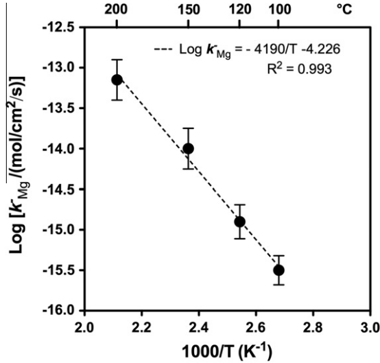
Fig. 7. Arrhenius plot of retrieved rate constants as a function of reciprocal temperature. Filled circles represent rate constants listed in Table 7, whereas the dashed line corresponds to a linear least squares fit of these rate constants. The slope of this line is consistent with E_a = 80.2 kJ/mol and A_a = 5.9 \times 10^{-5} mol/cm 2 /s.
