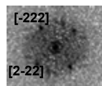
structure spinelle
